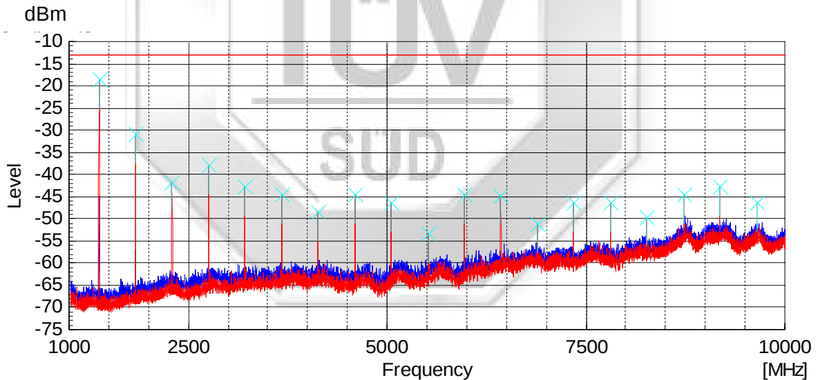
459.125MHz (Analog) 1GHz – 10GHz
