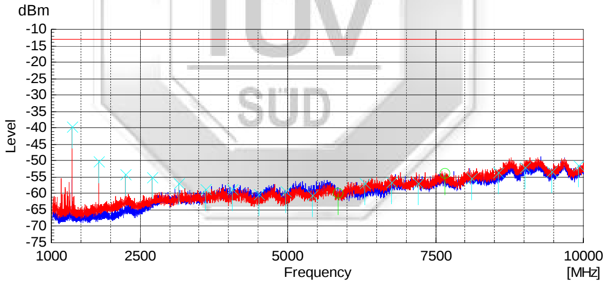
450.65MHz (Analog) 1GHz – 10GHz
