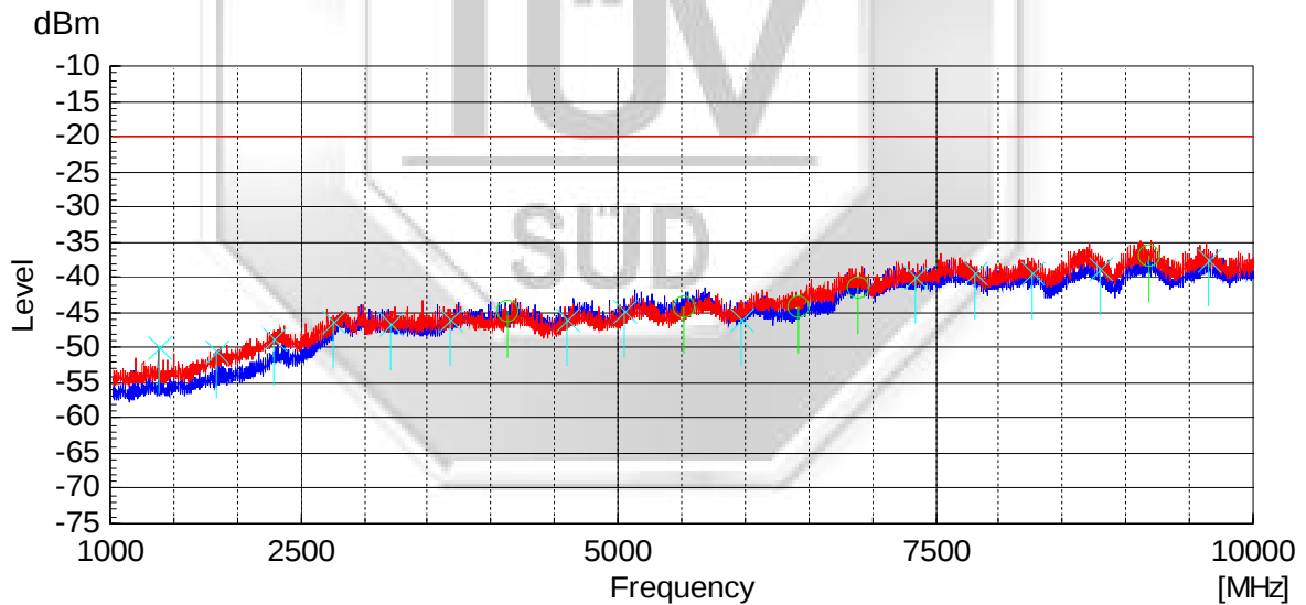
459.125MHz (Digital) 1GHz – 10GHz
