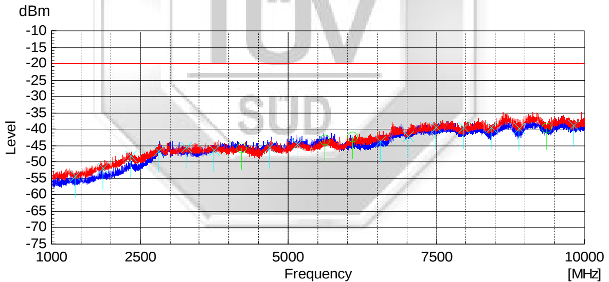
467.775MHz (Digital) 1GHz – 10GHz
