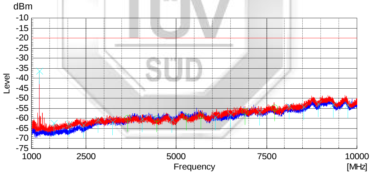
406.2MHz (Digital) 1GHz – 10GHz
