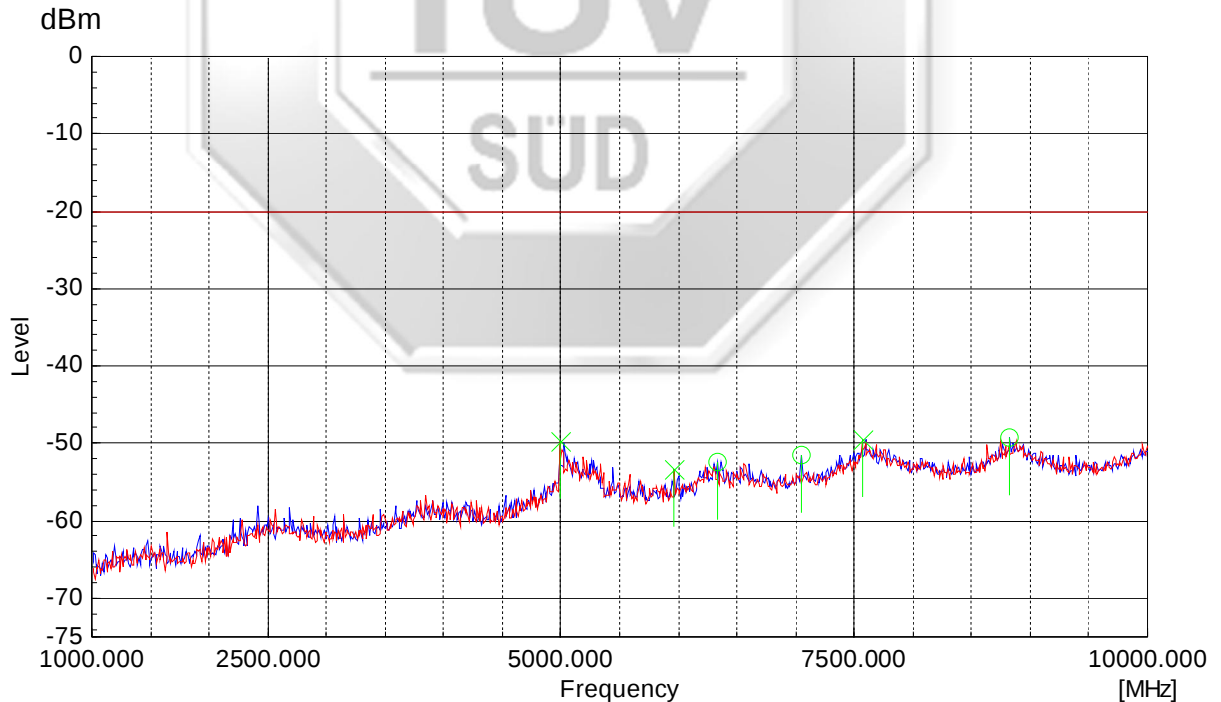
467.775MHz (Digital) 1GHz – 10GHz
