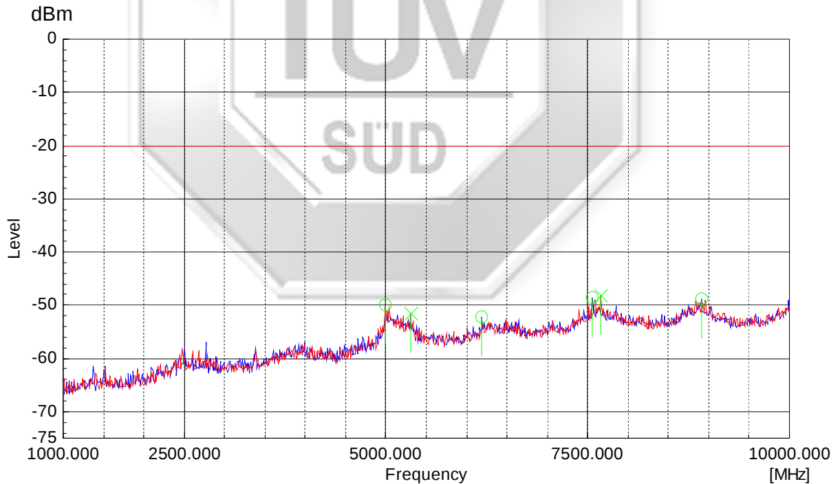
511.9875MHz (Digital) 1GHz – 10GHz
