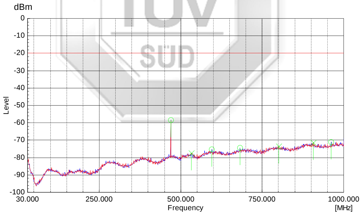
467.775MHz (Digital) 30MHz – 1GHz
