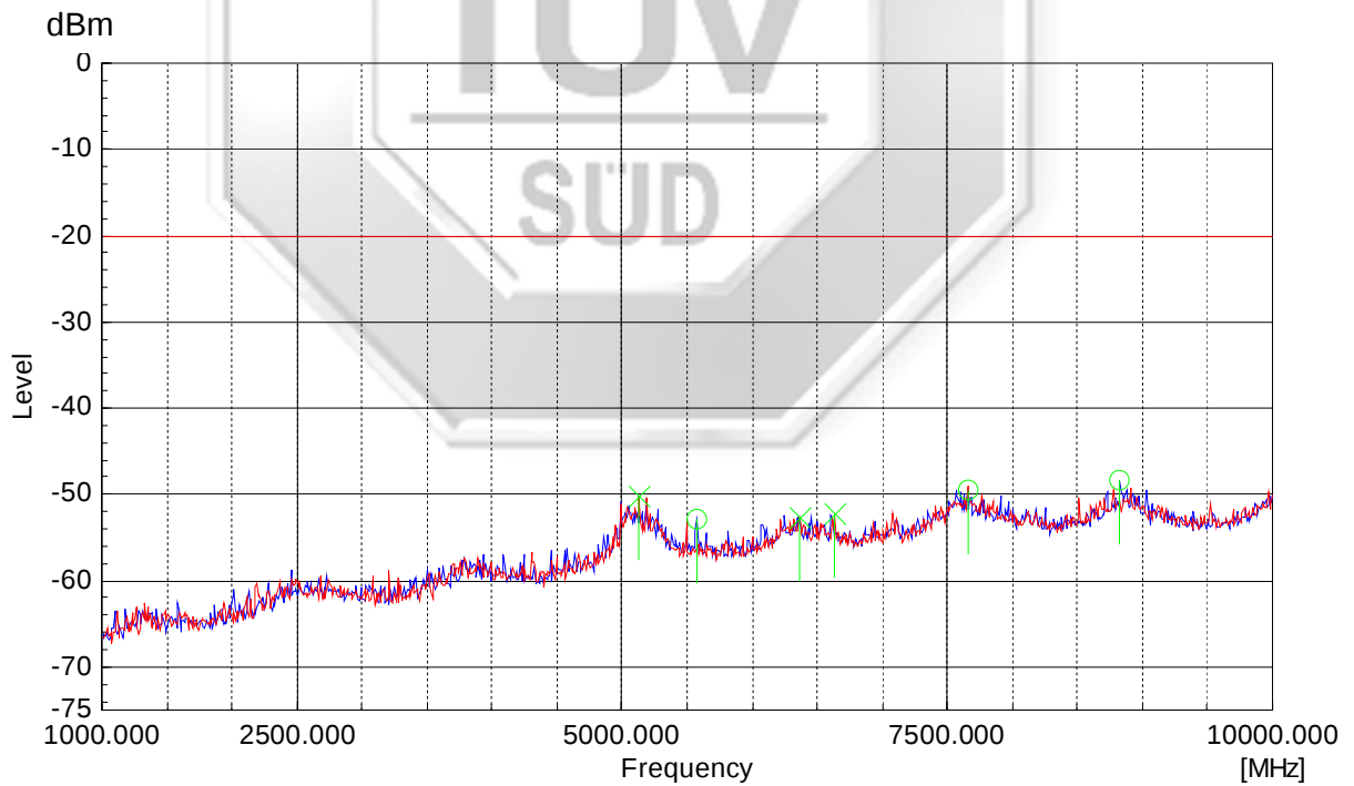
459.125MHz (Digital) 1GHz – 10GHz
