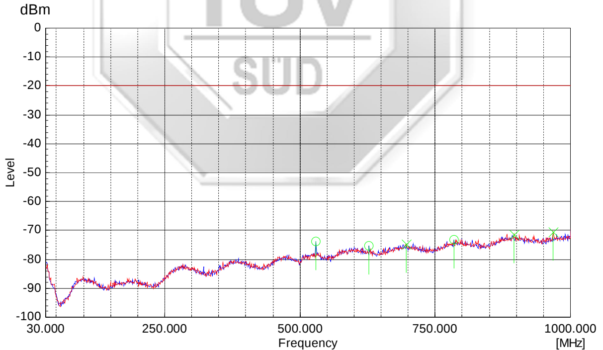
467.775MHz (Digital) 30MHz – 1GHz
