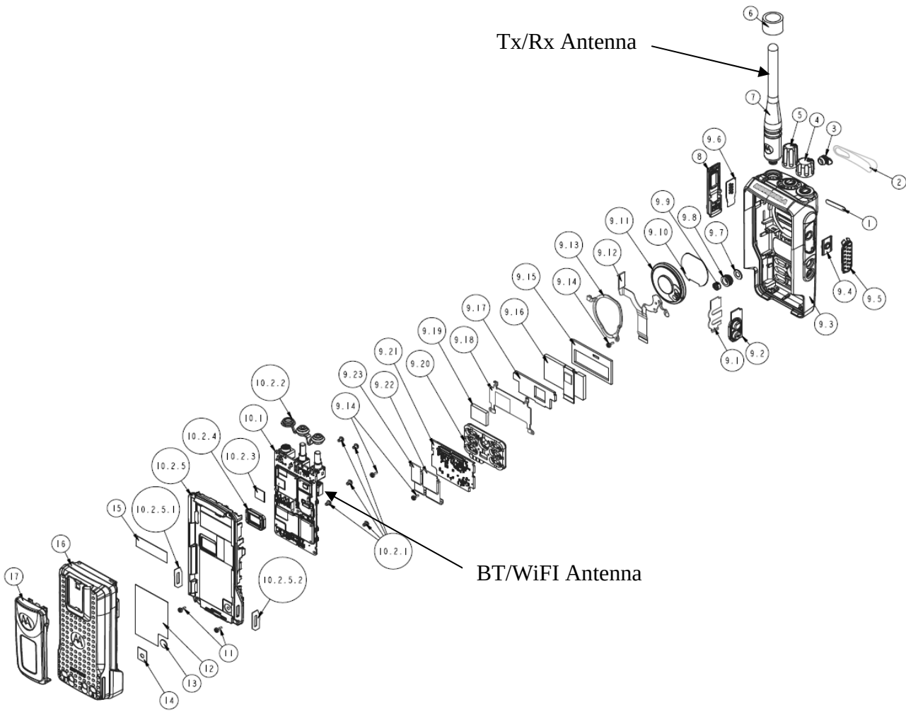
Exploded View of FKP Radio
