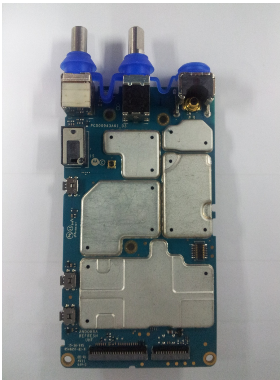
RF board with Shields (Top)
