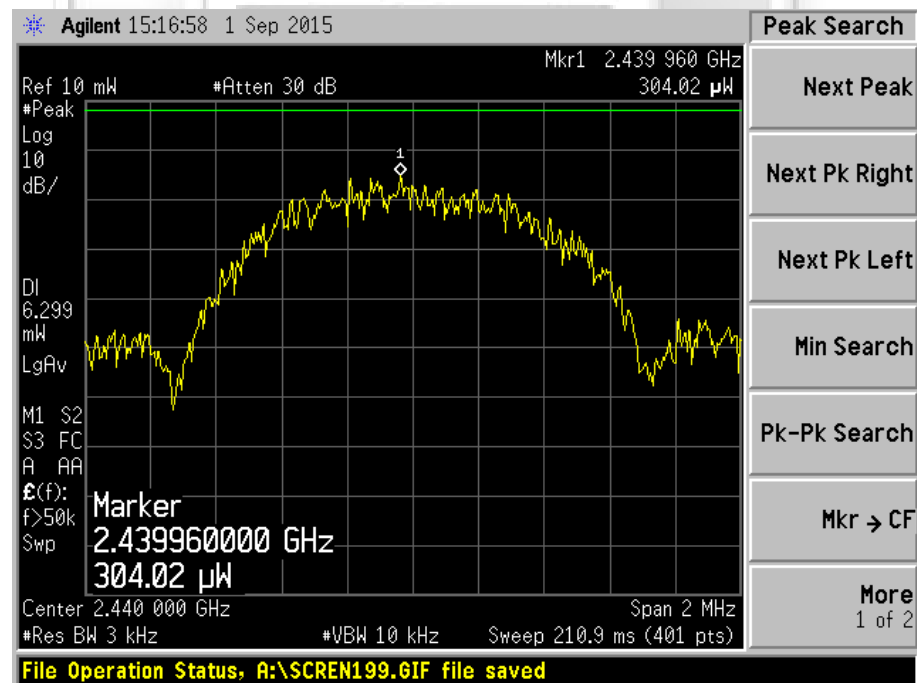
Plot 40 – Channel 19
