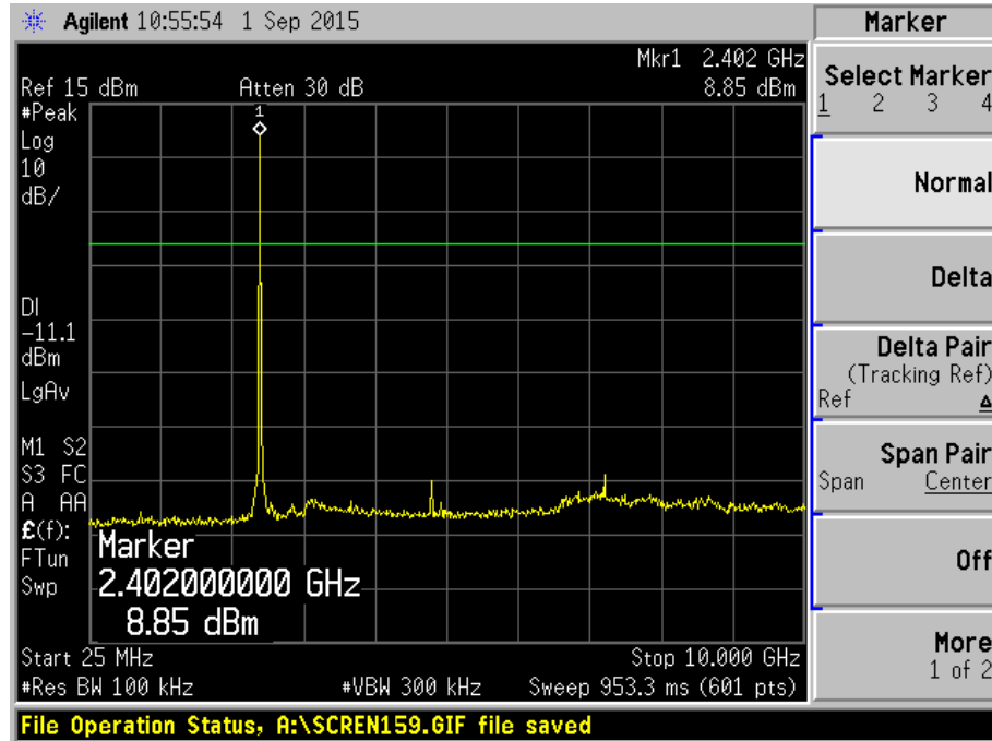
Plot 7 – Channel 0
