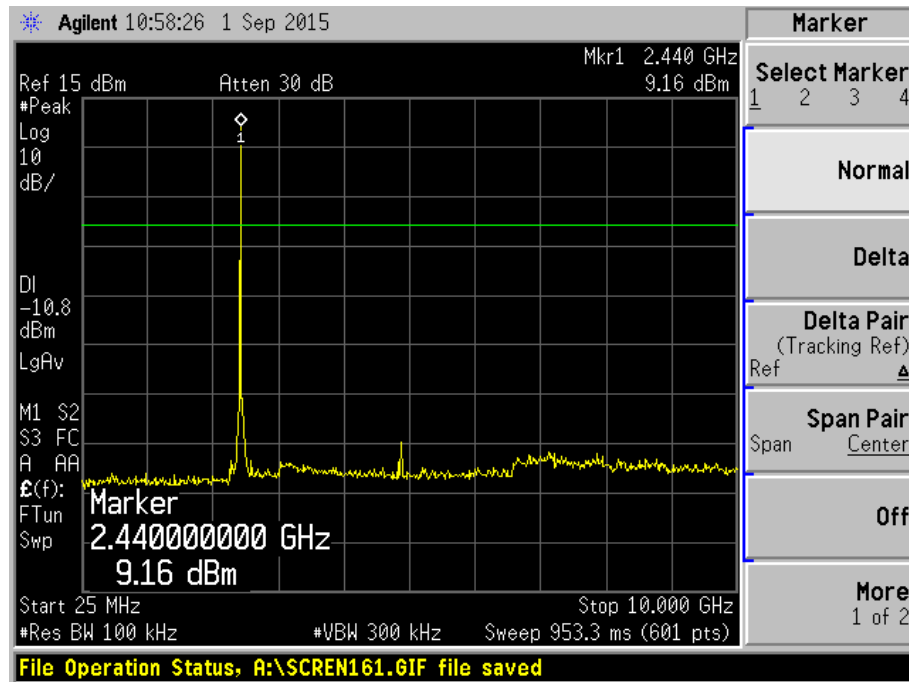
Plot 9 – Channel 19
