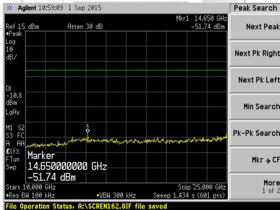
Plot 10 – Channel 19
