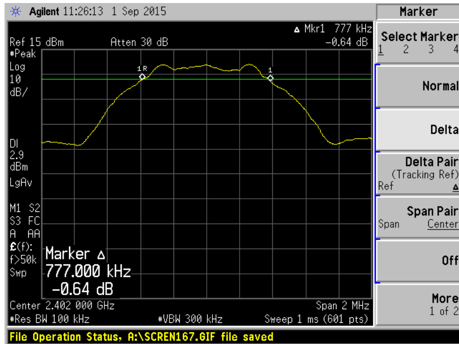
Plot 1 - Channel 0
