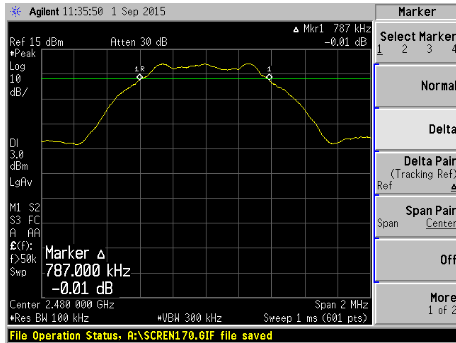
Plot 3 - Channel 39
