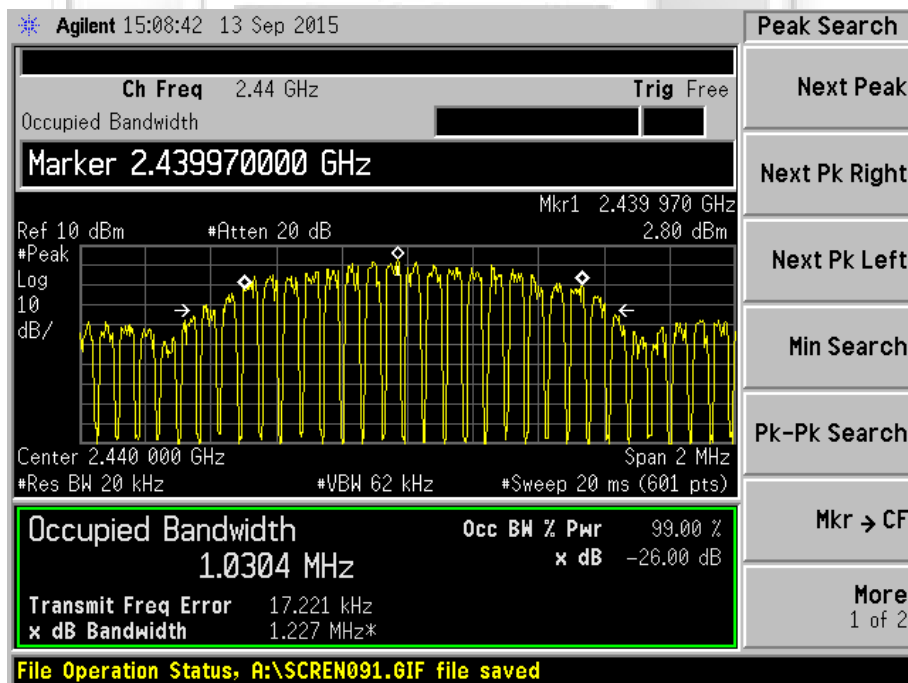
Plot 5 - Channel 19
