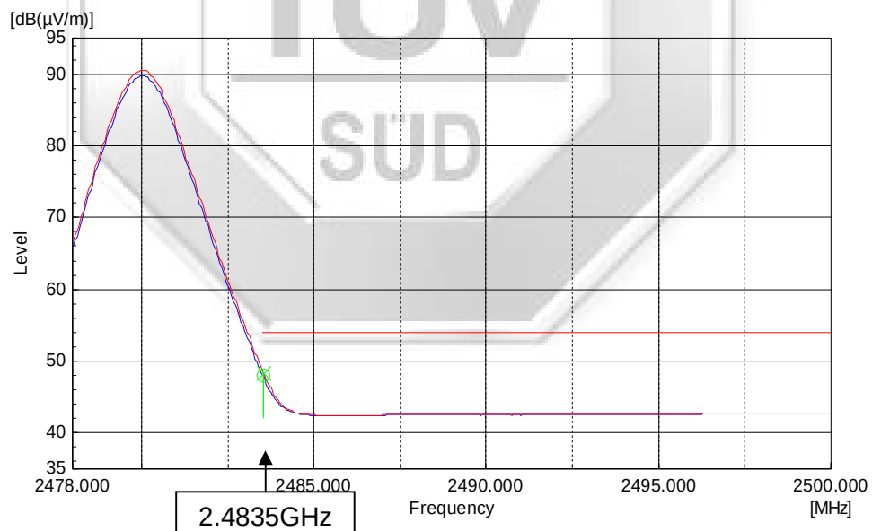
Plot 71 – Average Plot at Upper Band Edge at 2.4835GHz
