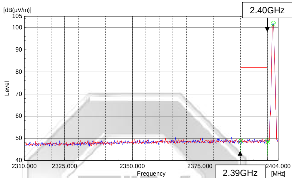
Plot 66 – Lower Band Edge at 2.4000GHz
