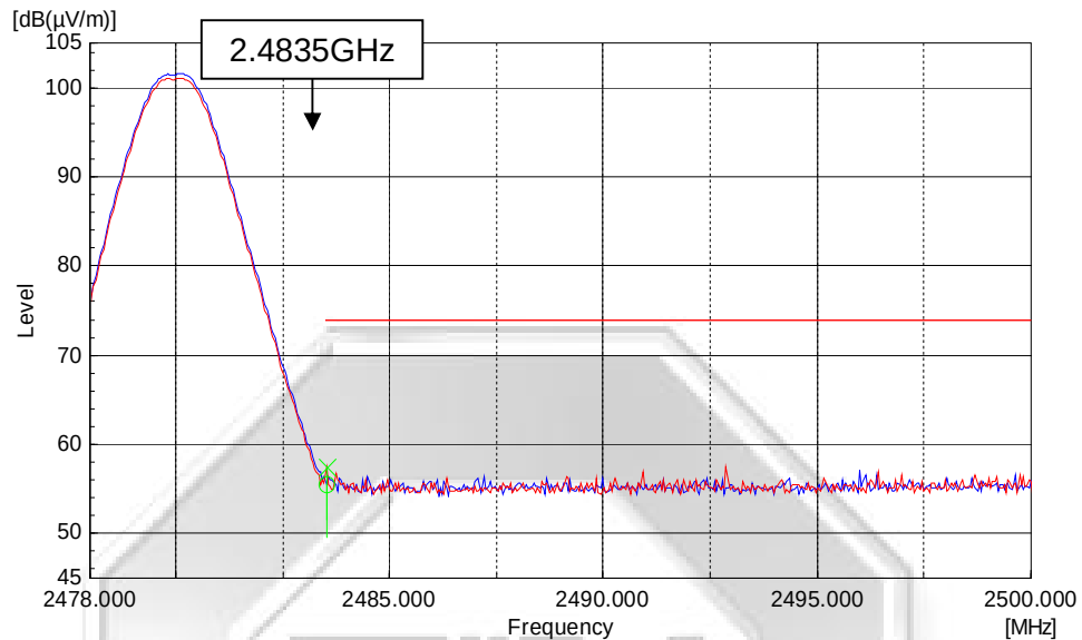
Plot 70 – Peak Plot at Upper Band Edge at 2.4835GHz
