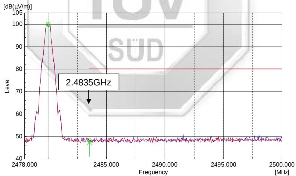
Plot 67 – Upper Band Edge at 2.4835GHz
