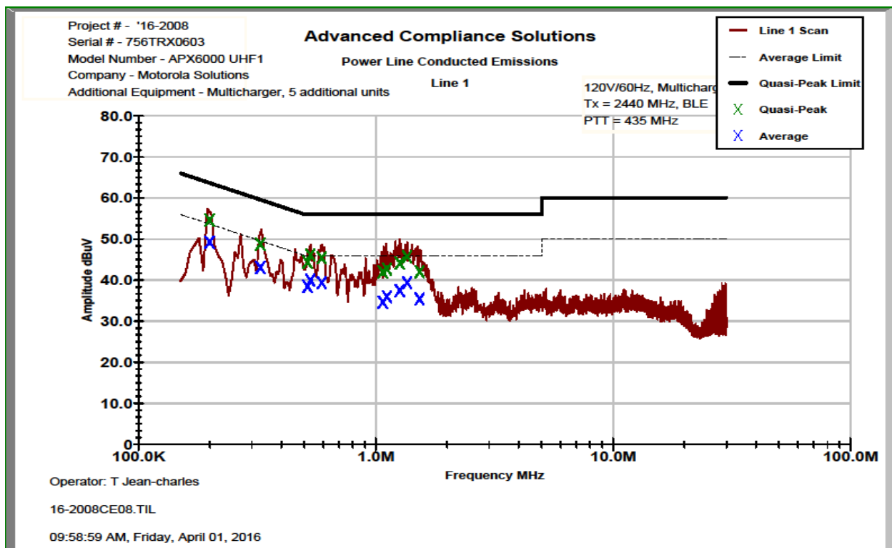
Figure 7.6.2-1: Conducted Emissions Results – Line 1
