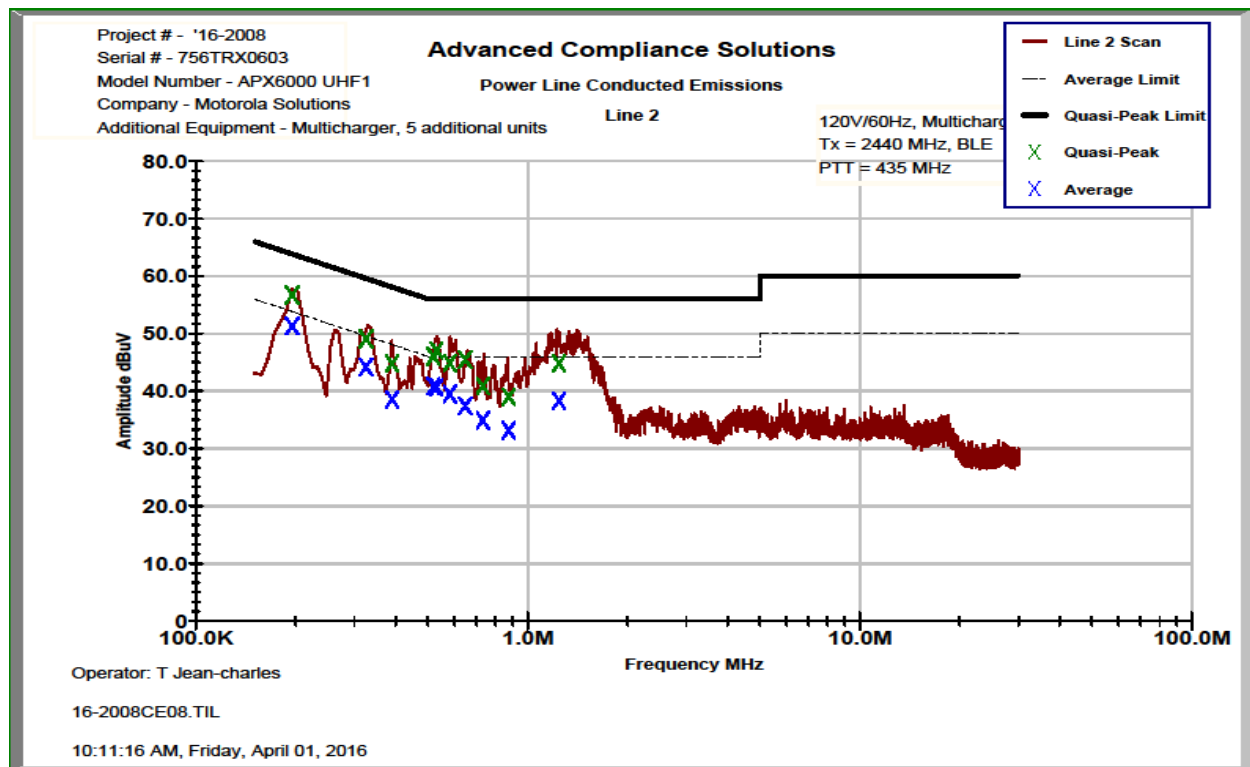
Figure 7.6.2-2: Conducted Emissions Results – Line 2
