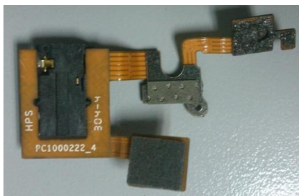
Photograph 9-9: Top side of aux flex
