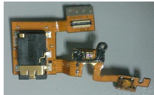
Photograph 9-10: Bottom side of aux flex
