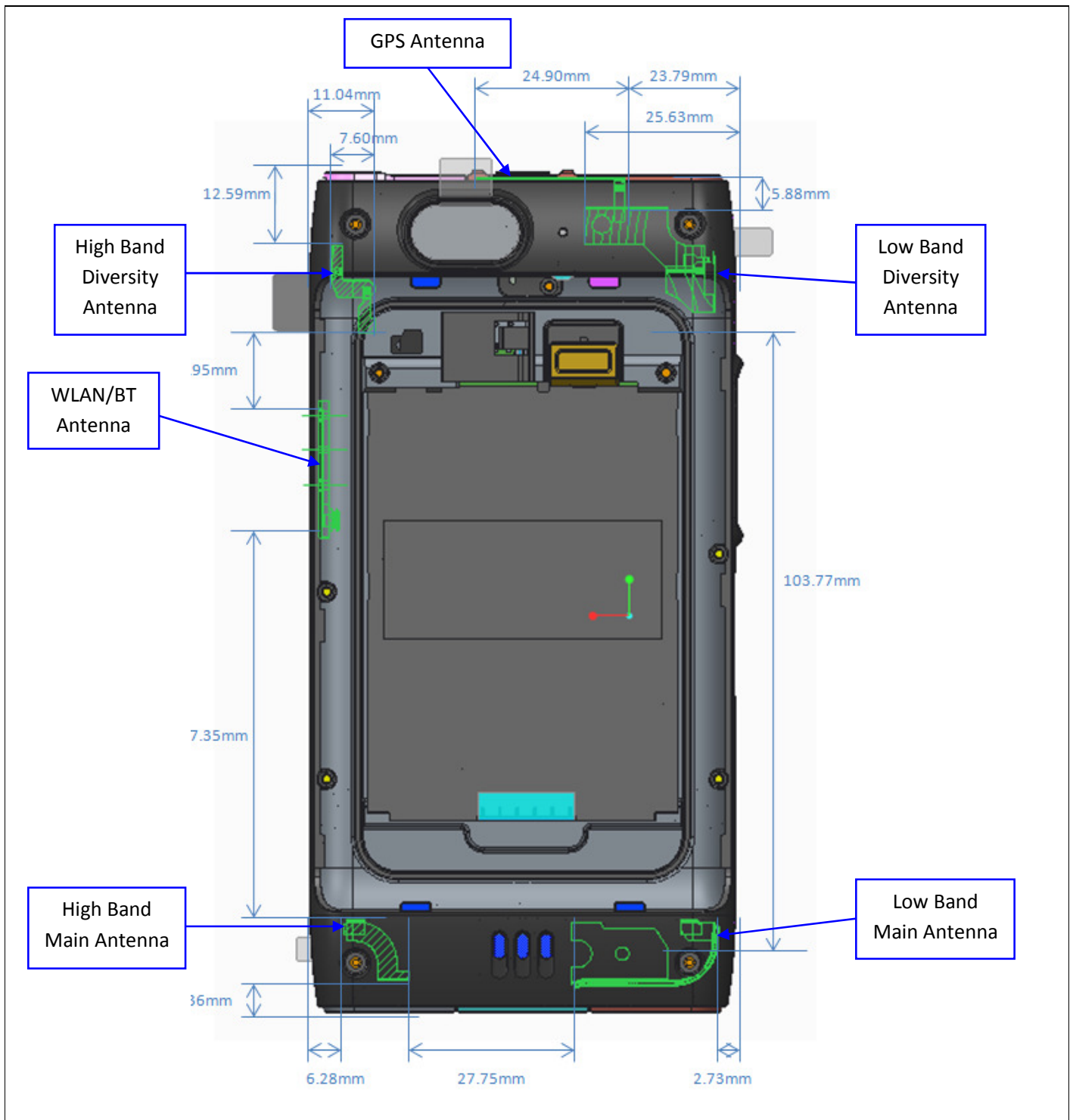
Photograph 9-15: Antenna locations and spacing
