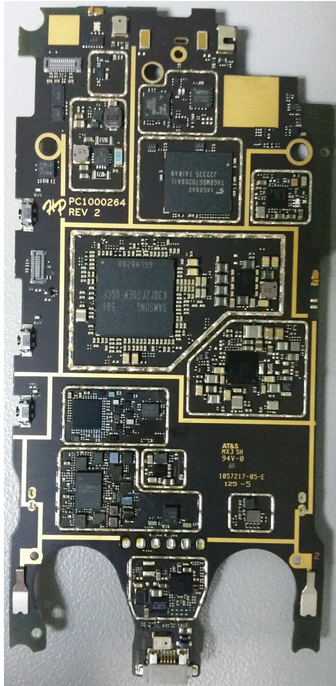
Photograph 9-3: Top side of main board, without shields
