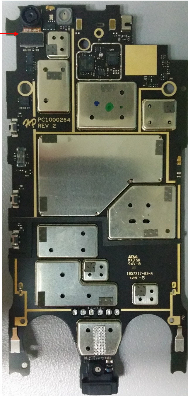
Photograph 9-11: Top side of main board with front camera
