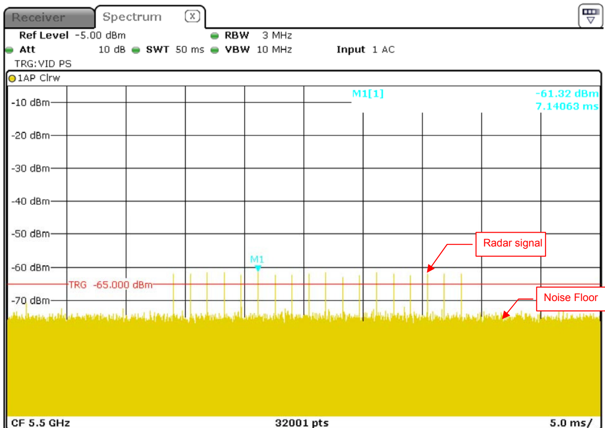
Radar Signal 0
