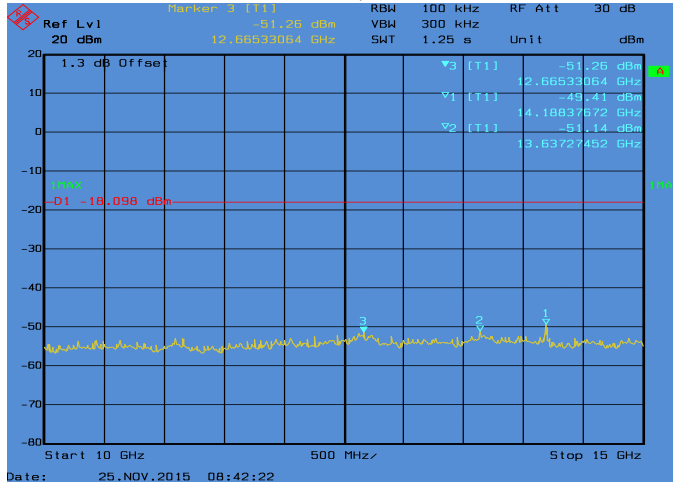
Conducted Emissions. Bluetooth, Frequency 2480 MHz Emission Level, 10 GHz -> 15 GHz
