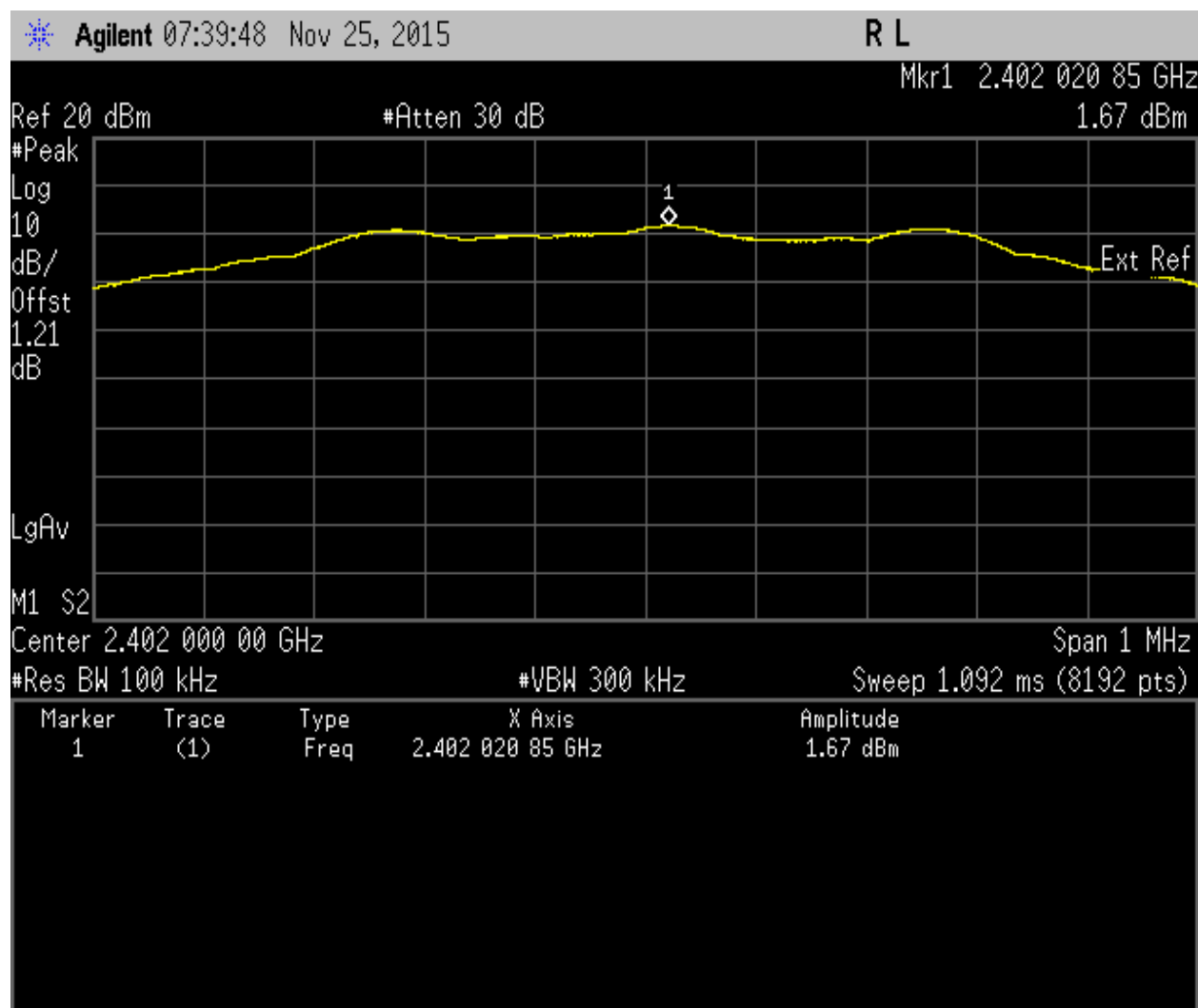
Maximum Peak Power Spectral Density. Bluetooth Frequency 2402 MHz
