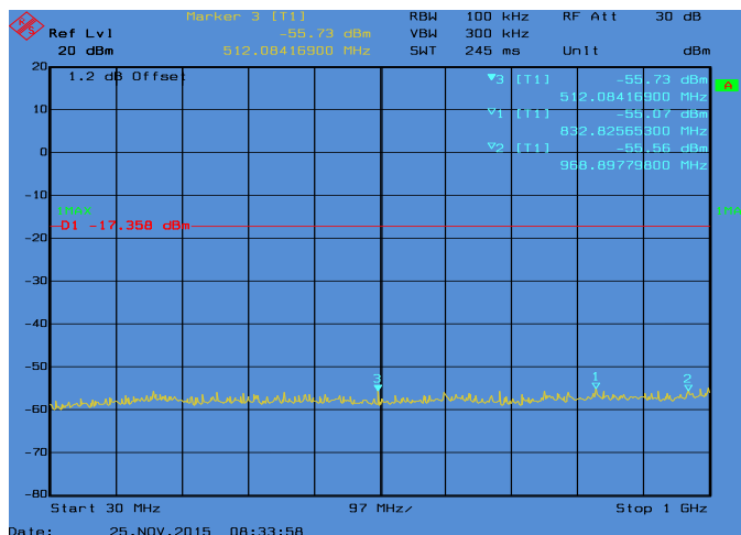
Conducted Emissions. Bluetooth, Frequency 2402 MHz Emission Level, 30 MHz -> 1 GHz
