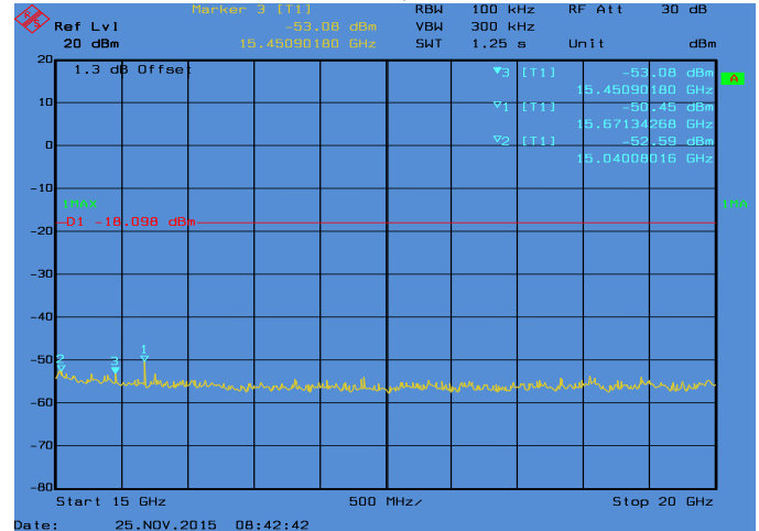
Conducted Emissions. Bluetooth, Frequency 2480 MHz Emission Level, 15 GHz -> 20 GHz
