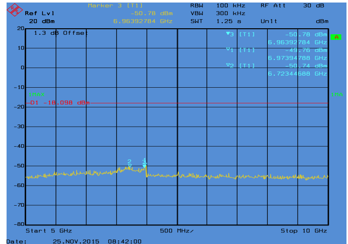
Conducted Emissions. Bluetooth, Frequency 2480 MHz Emission Level, 5 GHz -> 10 GHz
