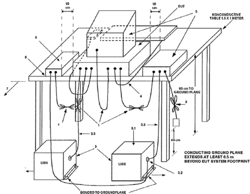
Figure 1: AC Power Line Conducted Emission Test Setup Diagram (Table Top Equipment)
