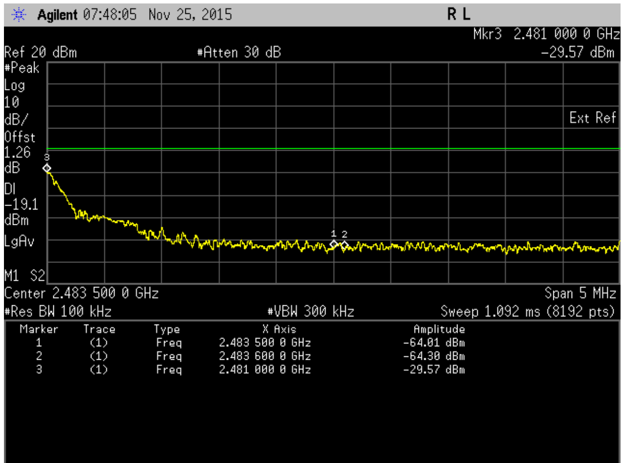
Band Edge (100 kHz). Bluetooth Frequency 2480 MHz Band Edge
