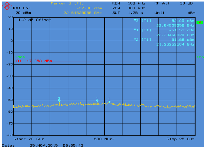
Conducted Emissions. Bluetooth, Frequency 2402 MHz Emission Level, 20 GHz -> 25 GHz
