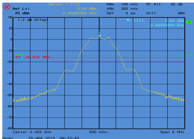
Conducted Emissions. Bluetooth, Frequency 2402 MHz Reference Level
