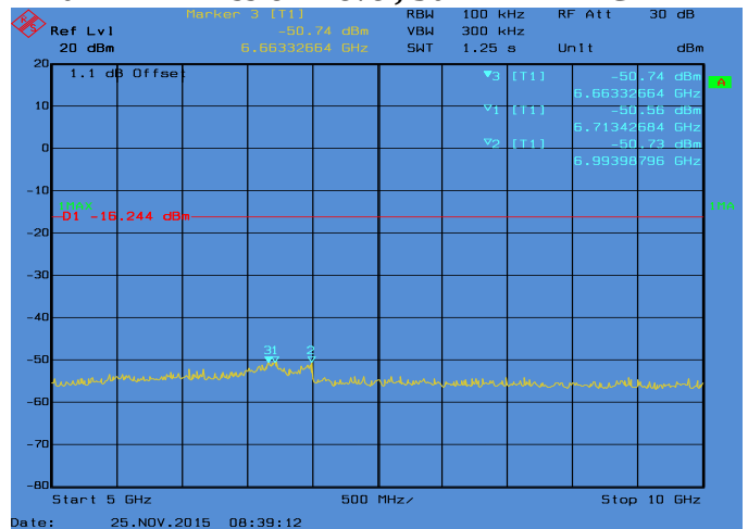
Conducted Emissions. Bluetooth, Frequency 2440 MHz Emission Level, 5 GHz -> 10 GHz
