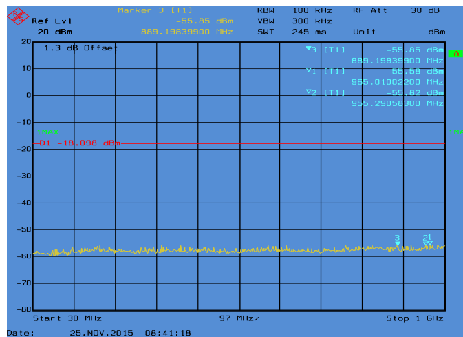
Conducted Emissions. Bluetooth, Frequency 2480 MHz Emission Level, 30 MHz -> 1 GHz
