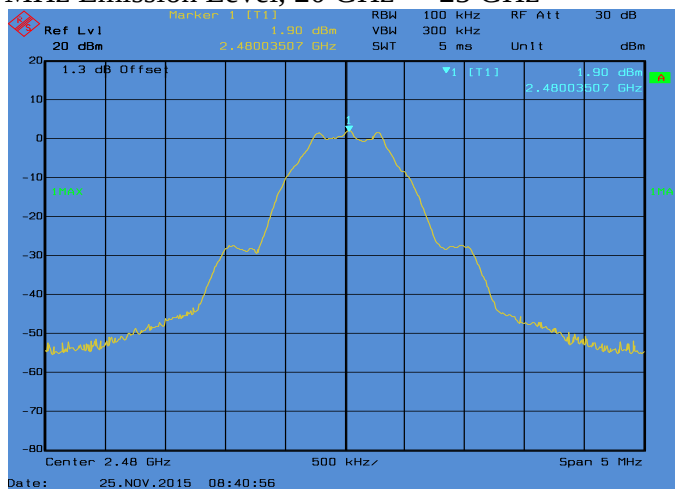
Conducted Emissions. Bluetooth, Frequency 2480 MHz Reference Level
