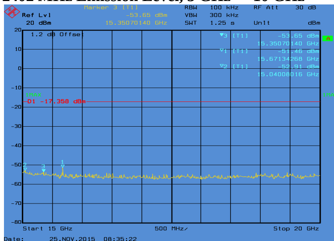
Conducted Emissions. Bluetooth, Frequency 2402 MHz Emission Level, 15 GHz -> 20 GHz
