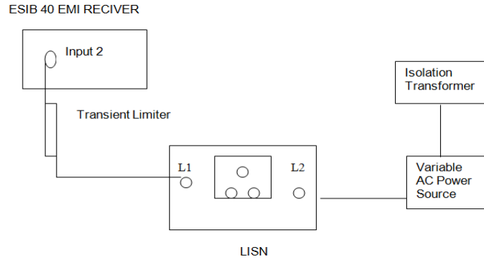
Figure 2: AC Power Line Conducted Emission Test System General Equipment Block Diagram.
