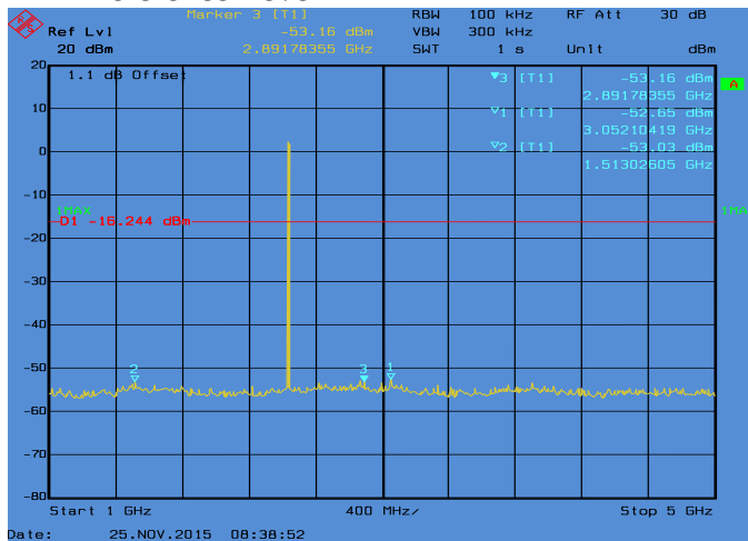
Conducted Emissions. Bluetooth, Frequency 2440 MHz Emission Level, 1 GHz -> 5 GHz
