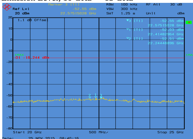
Conducted Emissions. Bluetooth, Frequency 2440 MHz Emission Level, 20 GHz -> 25 GHz
