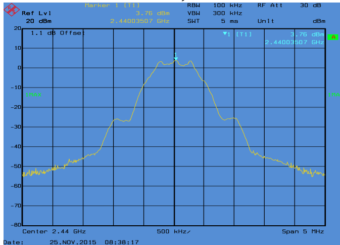
Conducted Emissions. Bluetooth, Frequency 2440 MHz Reference Level
