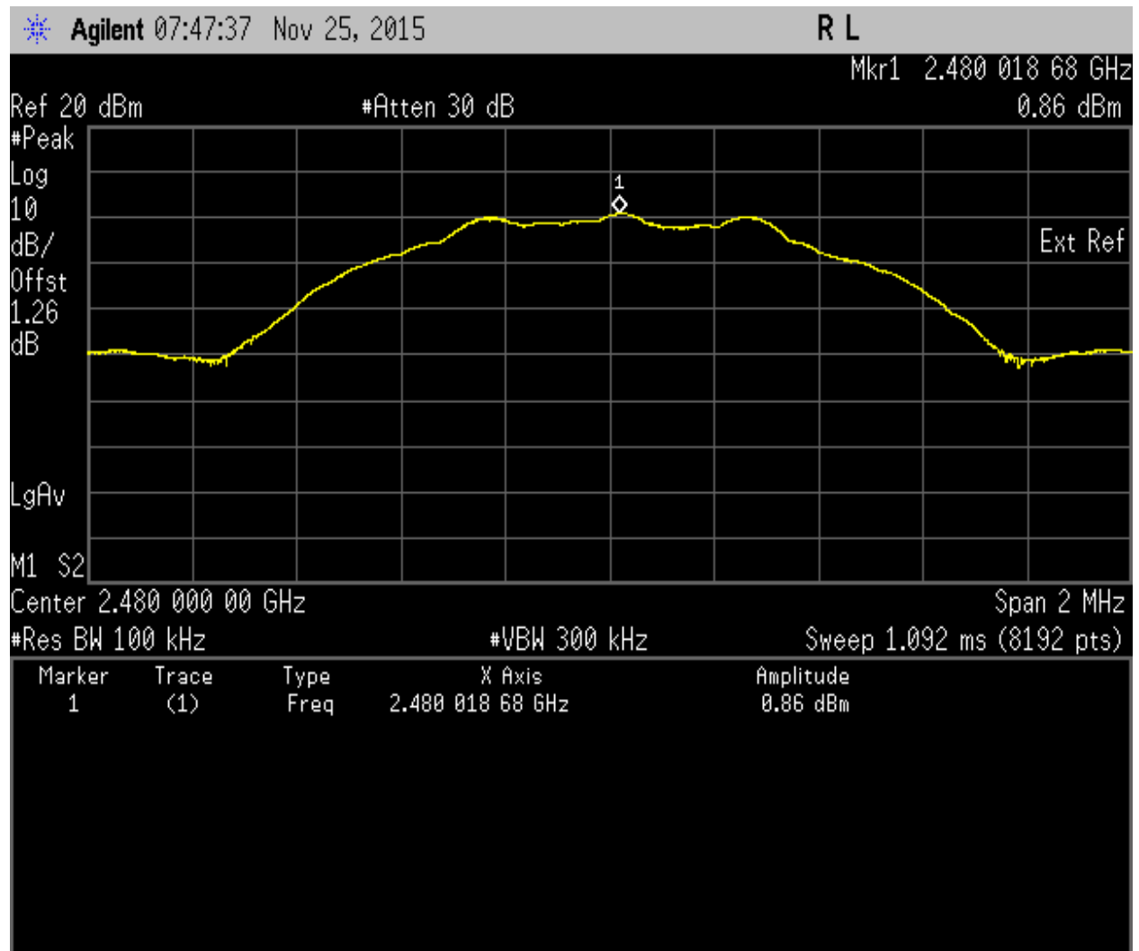
Maximum Peak Power Spectral Density. Bluetooth Frequency 2480 MHz
