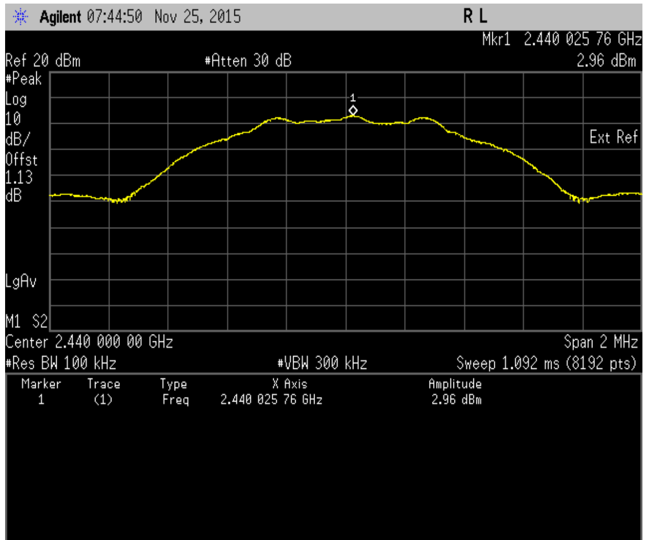
Maximum Peak Power Spectral Density. Bluetooth Frequency 2440 MHz
