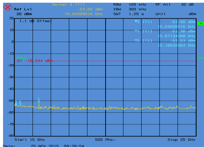
Conducted Emissions. Bluetooth, Frequency 2440 MHz Emission Level, 15 GHz -> 20 GHz
