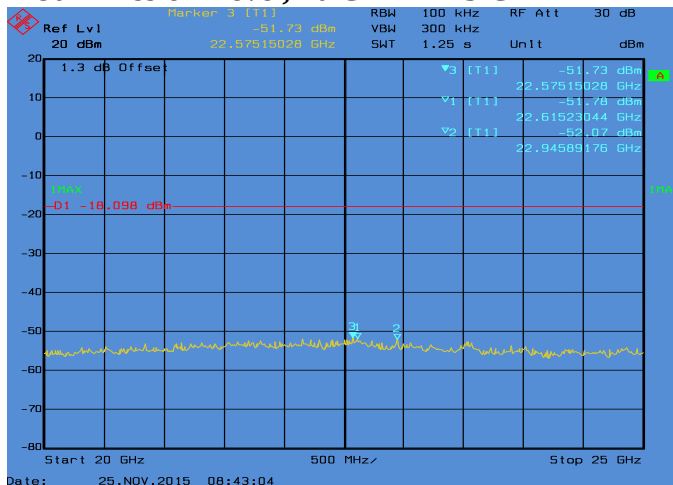
Conducted Emissions. Bluetooth, Frequency 2480 MHz Emission Level, 20 GHz -> 25 GHz
