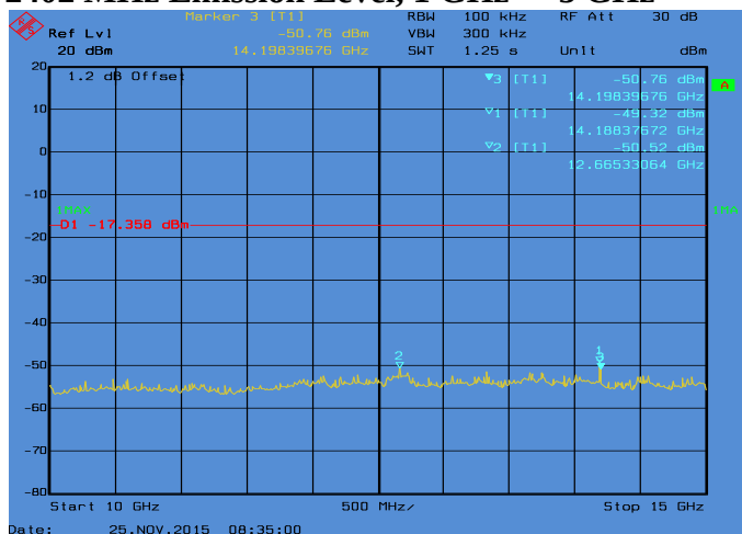
Conducted Emissions. Bluetooth, Frequency 2402 MHz Emission Level, 10 GHz -> 15 GHz
