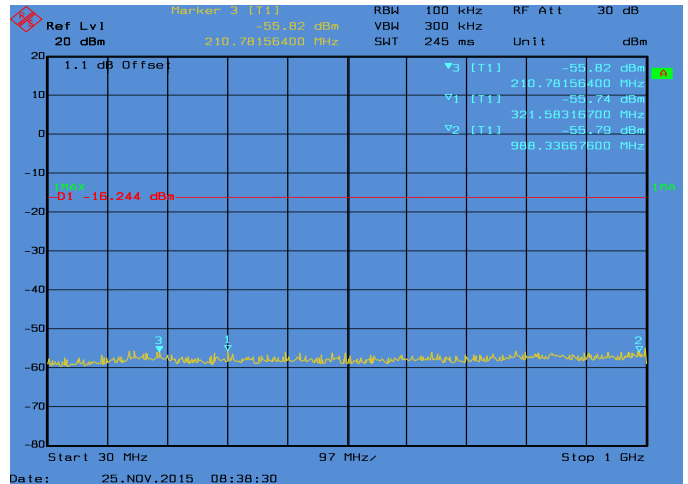
Conducted Emissions. Bluetooth, Frequency 2440 MHz Emission Level, 30 MHz -> 1 GHz
