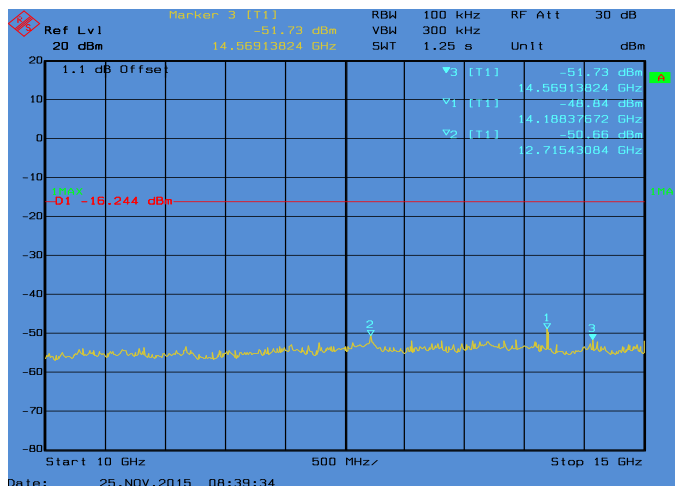
Conducted Emissions. Bluetooth, Frequency 2440 MHz Emission Level, 10 GHz -> 15 GHz
