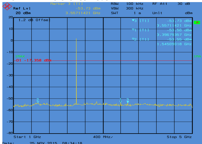
Conducted Emissions. Bluetooth, Frequency 2402 MHz Emission Level, 1 GHz -> 5 GHz
