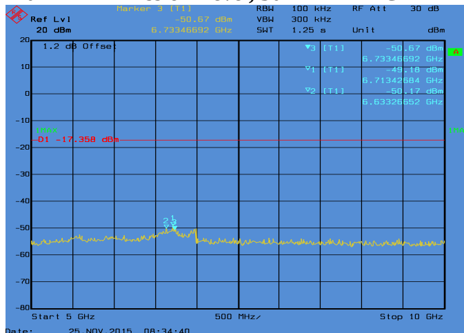
Conducted Emissions. Bluetooth, Frequency 2402 MHz Emission Level, 5 GHz -> 10 GHz
