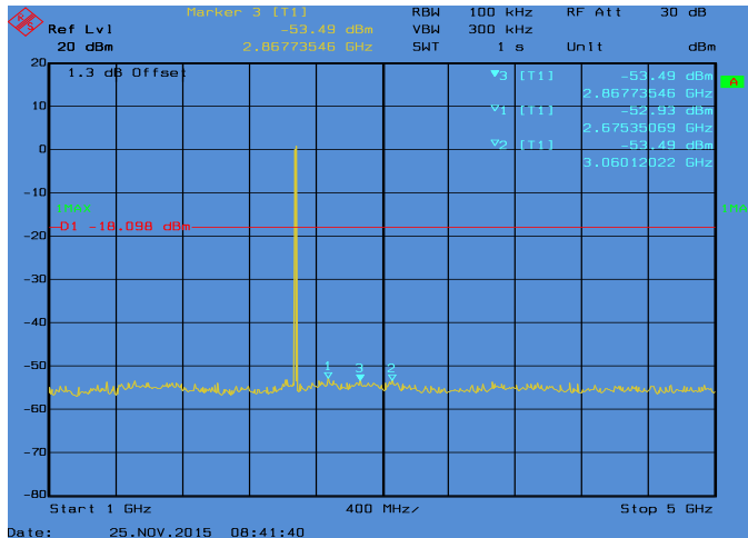
Conducted Emissions. Bluetooth, Frequency 2480 MHz Emission Level, 1 GHz -> 5 GHz
