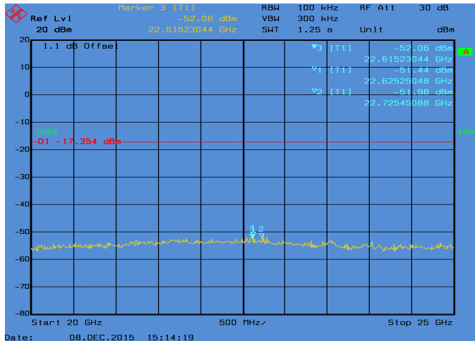
Conducted Emissions. 802.11n_20, Frequency 2437 MHz Emission Level, 20 GHz -> 25 GHz
