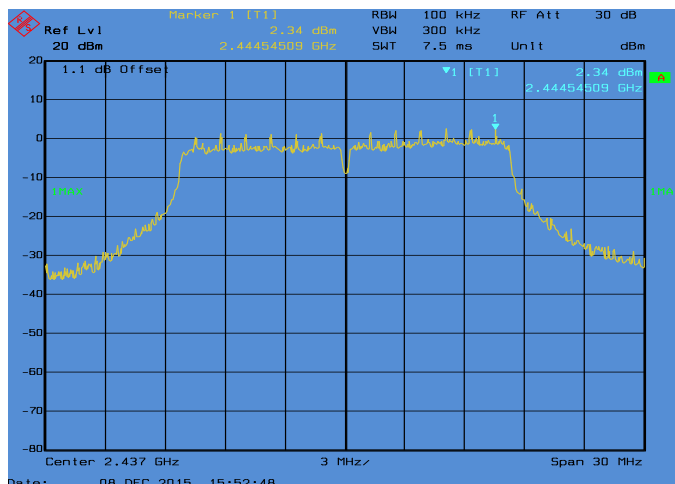
Conducted Emissions. 802.11g, Frequency 2437 MHz Reference Level
