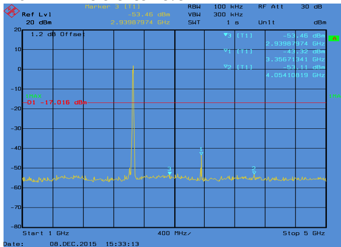
Conducted Emissions. 802.11n_20, Frequency 2462 MHz Emission Level, 1 GHz -> 5 GHz
