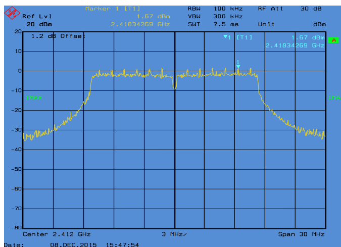
Conducted Emissions. 802.11g, Frequency 2412 MHz Reference Level
