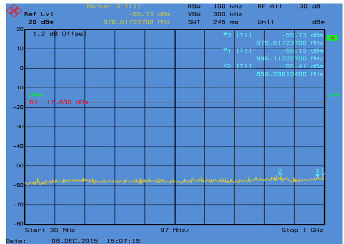
Conducted Emissions. 802.11n_20, Frequency 2412 MHz Emission Level, 30 MHz -> 1 GHz
