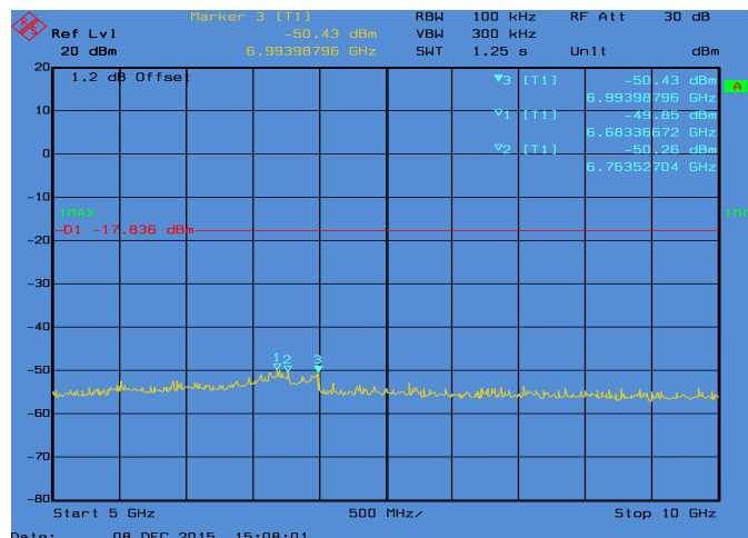
Conducted Emissions. 802.11n_20, Frequency 2412 MHz Emission Level, 5 GHz -> 10 GHz
