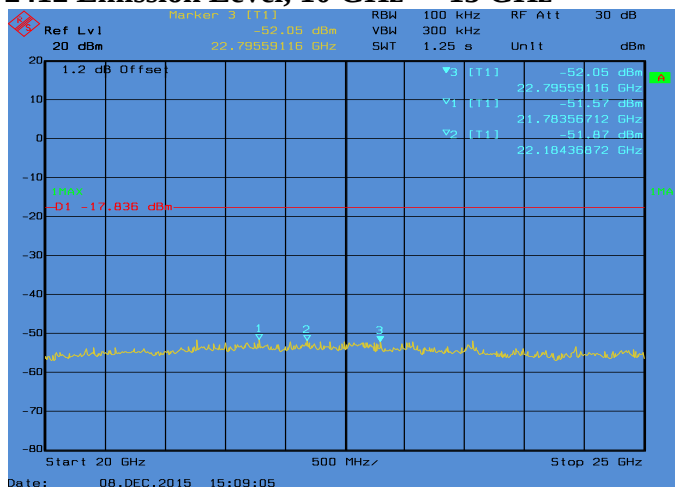
Conducted Emissions. 802.11n_20, Frequency 2412 MHz Emission Level, 20 GHz -> 25 GHz
