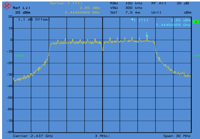
Conducted Emissions. 802.11n_20, Frequency 2437 MHz Reference Level
