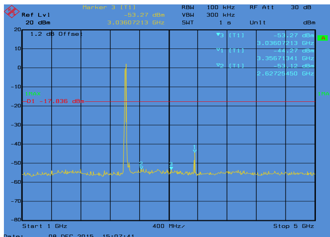
Conducted Emissions. 802.11n_20, Frequency 2412 MHz Emission Level, 1 GHz -> 5 GHz
