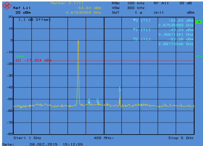
Conducted Emissions. 802.11n_20, Frequency 2437 MHz Emission Level, 1 GHz -> 5 GHz
