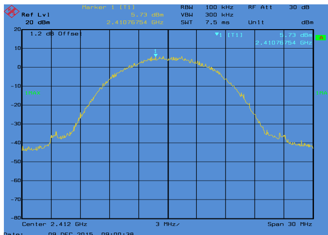
Conducted Emissions. 802.11b, Frequency 2412 MHz Reference Level
