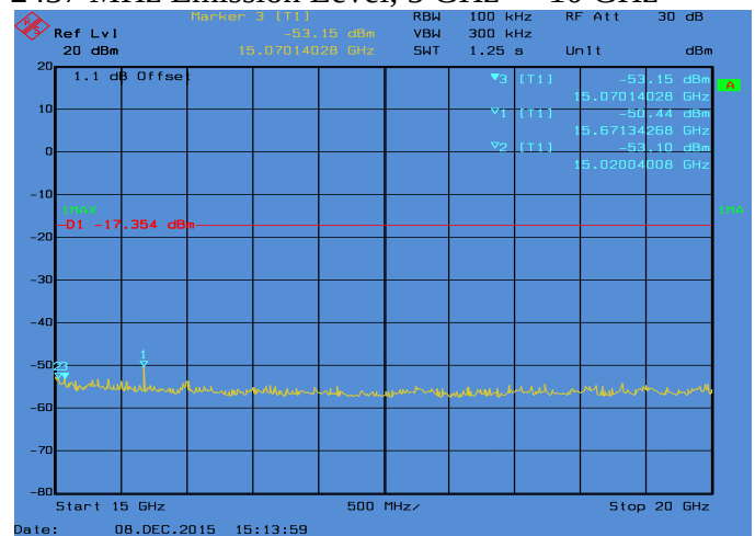
Conducted Emissions. 802.11n_20, Frequency 2437 MHz Emission Level, 15 GHz -> 20 GHz
