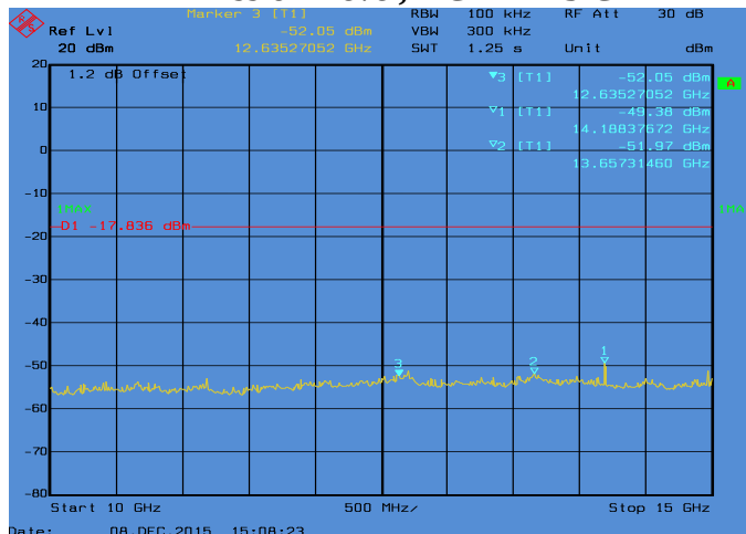
Conducted Emissions. 802.11n_20, Frequency 2412 MHz Emission Level, 10 GHz -> 15 GHz
