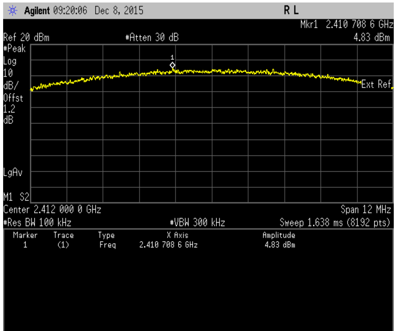
Maximum Peak Power Spectral Density. 802.11b Frequency 2412 MHz
