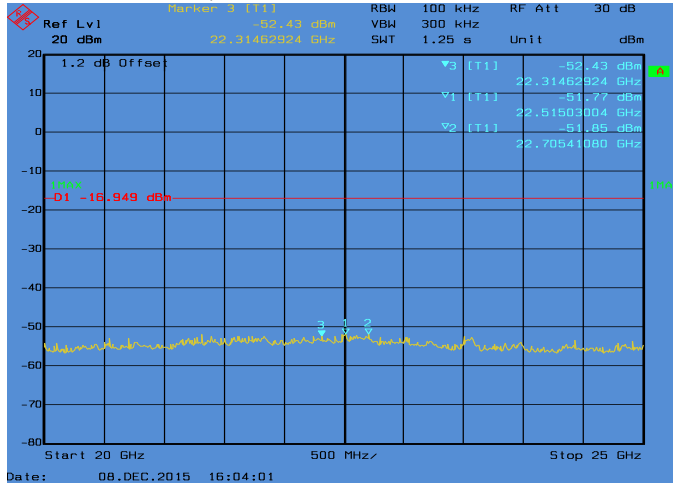
Conducted Emissions. 802.11g, Frequency 2462 MHz Emission Level, 20 GHz -> 25 GHz
