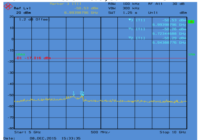
Conducted Emissions. 802.11n_20, Frequency 2462 MHz Emission Level, 5 GHz -> 10 GHz
