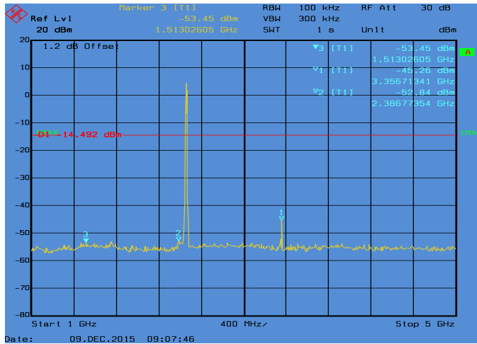
Conducted Emissions. 802.11b, Frequency 2462 MHz Emission Level, 1 GHz -> 5 GHz
