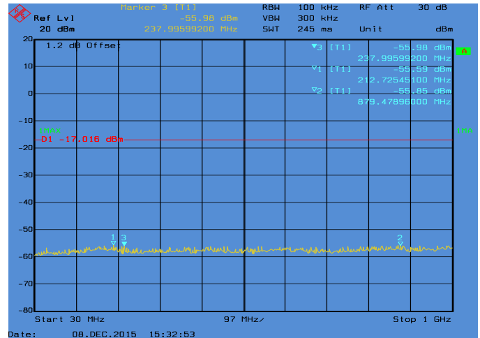
Conducted Emissions. 802.11n_20, Frequency 2462 MHz Emission Level, 30 MHz -> 1 GHz
