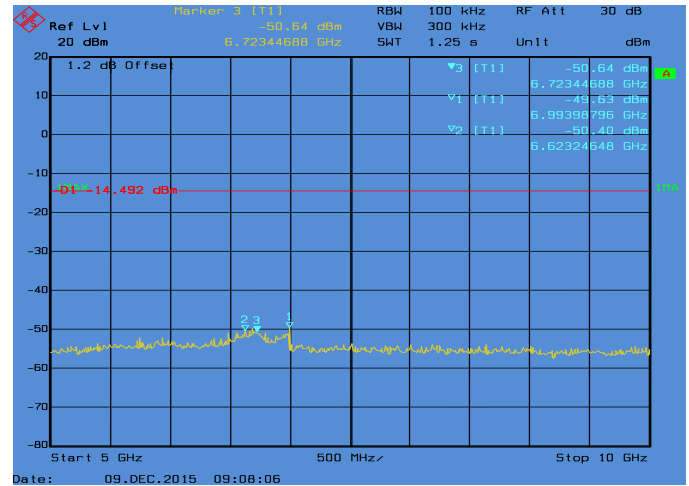
Conducted Emissions. 802.11b, Frequency 2462 MHz Emission Level, 5 GHz -> 10 GHz
