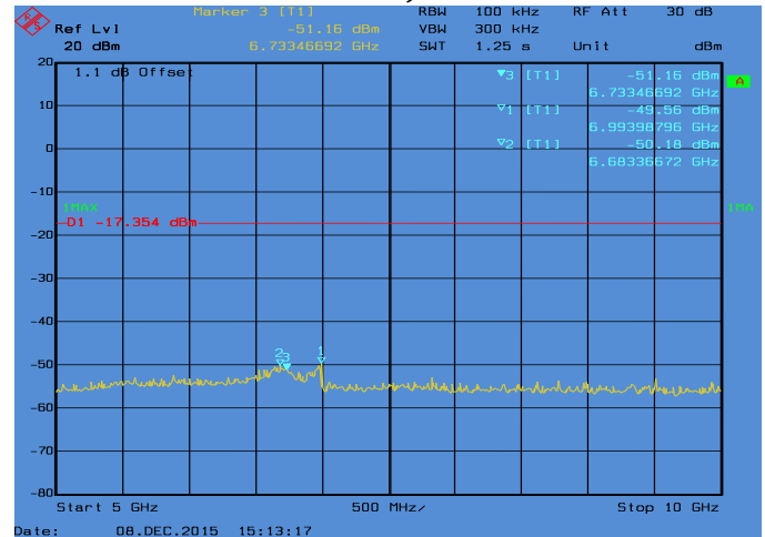
Conducted Emissions. 802.11n_20, Frequency 2437 MHz Emission Level, 5 GHz -> 10 GHz
