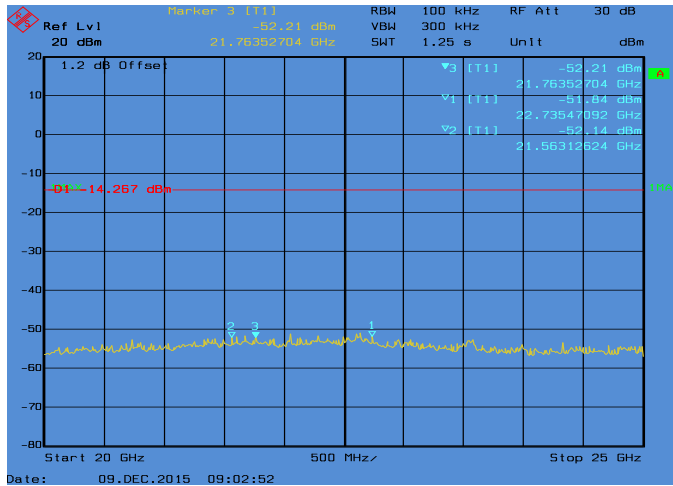
Conducted Emissions. 802.11b, Frequency 2412 MHz Emission Level, 20 GHz -> 25 GHz
