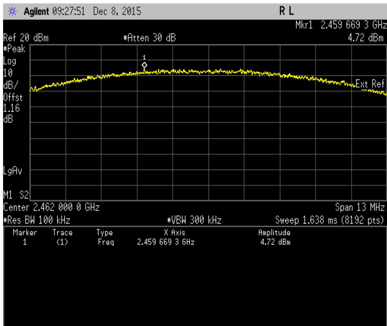
Maximum Peak Power Spectral Density. 802.11b Frequency 2462 MHz
