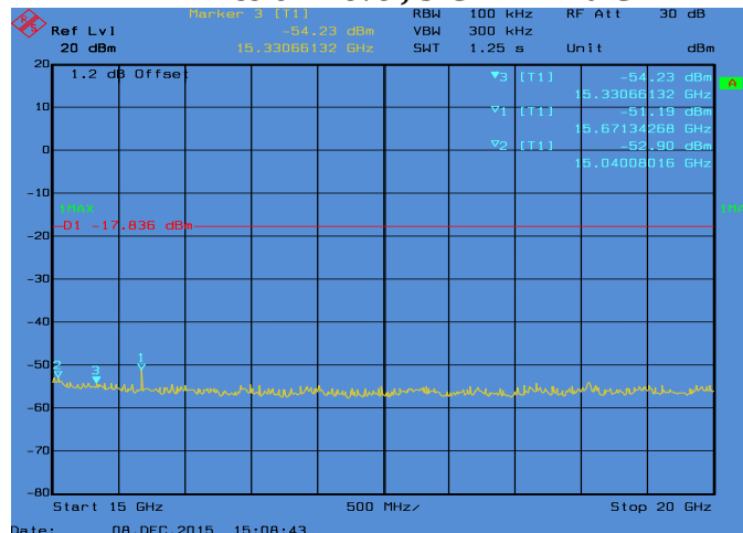
Conducted Emissions. 802.11n_20, Frequency 2412 MHz Emission Level, 15 GHz -> 20 GHz
