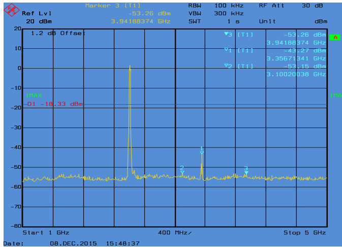
Conducted Emissions. 802.11g, Frequency 2412 MHz Emission Level, 1 GHz -> 5 GHz
