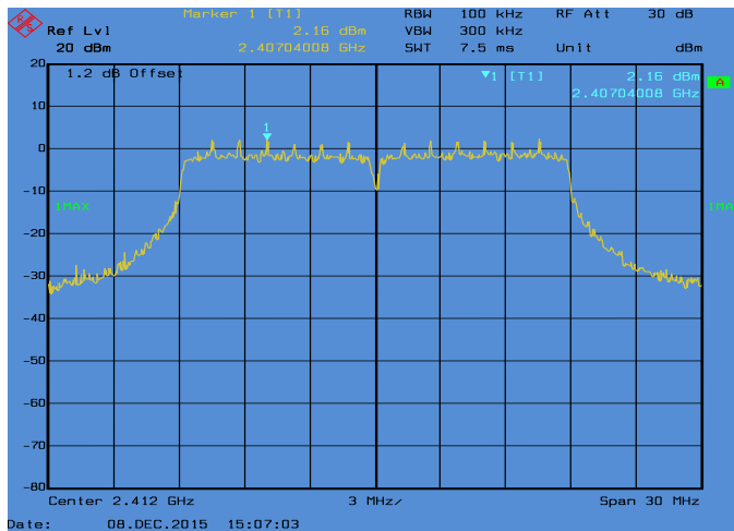
Conducted Emissions. 802.11n_20, Frequency 2412 MHz Reference Level
