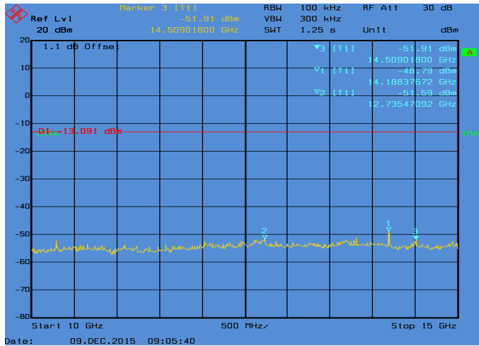
Conducted Emissions. 802.11b, Frequency 2437 Emission Level, 10 GHz -> 15 GHz
