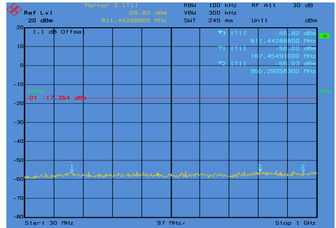
Conducted Emissions. 802.11n_20, Frequency 2437 MHz Emission Level, 30 MHz -> 1 GHz
