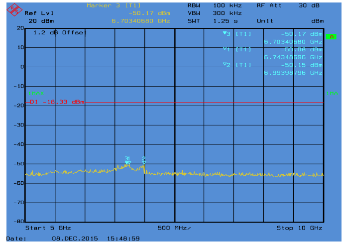
Conducted Emissions. 802.11g, Frequency 2412 MHz Emission Level, 5 GHz -> 10 GHz
