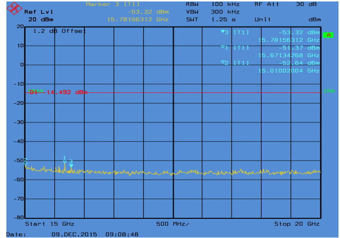
Conducted Emissions. 802.11b, Frequency 2462 MHz Emission Level, 15 GHz -> 20 GHz
