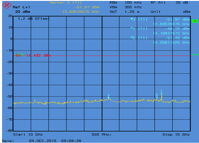
Conducted Emissions. 802.11b, Frequency 2462 MHz Emission Level, 10 GHz -> 15 GHz
