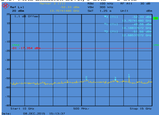
Conducted Emissions. 802.11n_20, Frequency 2437 MHz Emission Level, 10 GHz -> 15 GHz
