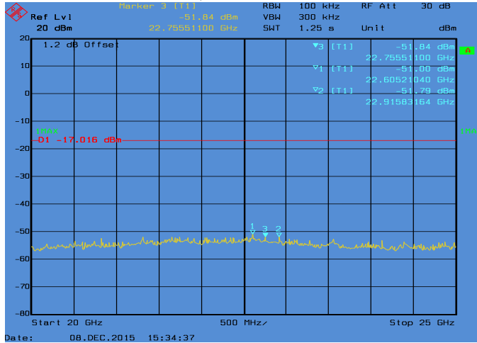
Conducted Emissions. 802.11n_20, Frequency 2462 MHz Emission Level, 20 GHz -> 25 GHz
