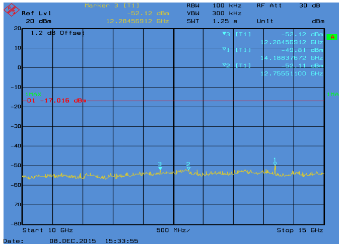
Conducted Emissions. 802.11n_20, Frequency 2462 Emission Level, 10 GHz -> 15 GHz
