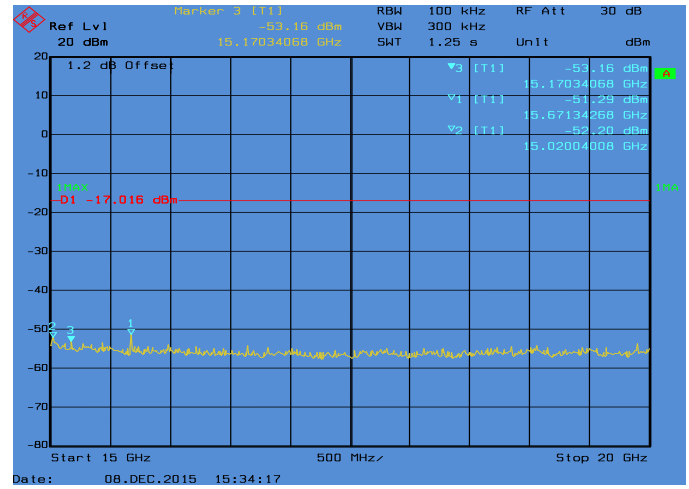
Conducted Emissions. 802.11n_20, Frequency 2462 MHz Emission Level, 15 GHz -> 20 GHz
