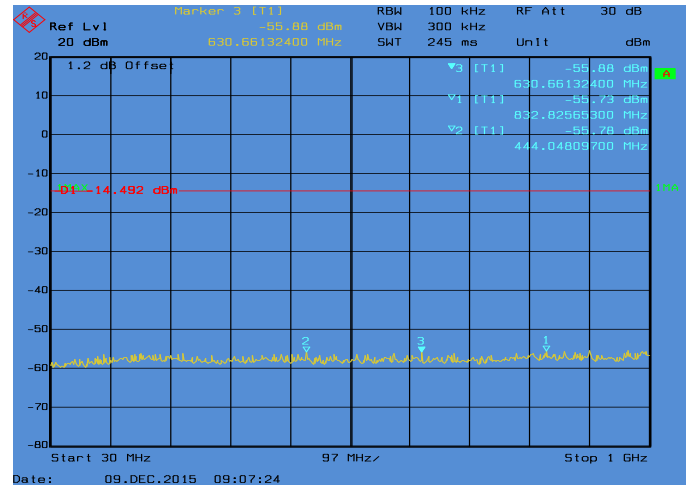
Conducted Emissions. 802.11b, Frequency 2462 MHz Emission Level, 30 MHz -> 1 GHz
