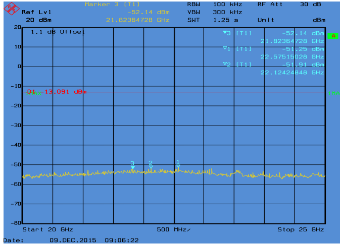
Conducted Emissions. 802.11b, Frequency 2437 MHz Emission Level, 20 GHz -> 25 GHz
