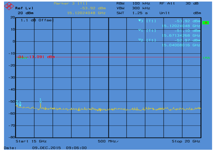
Conducted Emissions. 802.11b, Frequency 2437 MHz Emission Level, 15 GHz -> 20 GHz
