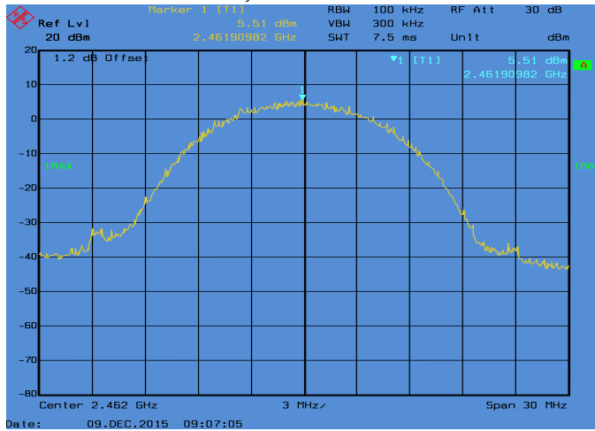
Conducted Emissions. 802.11b, Frequency 2462 MHz Reference Level
