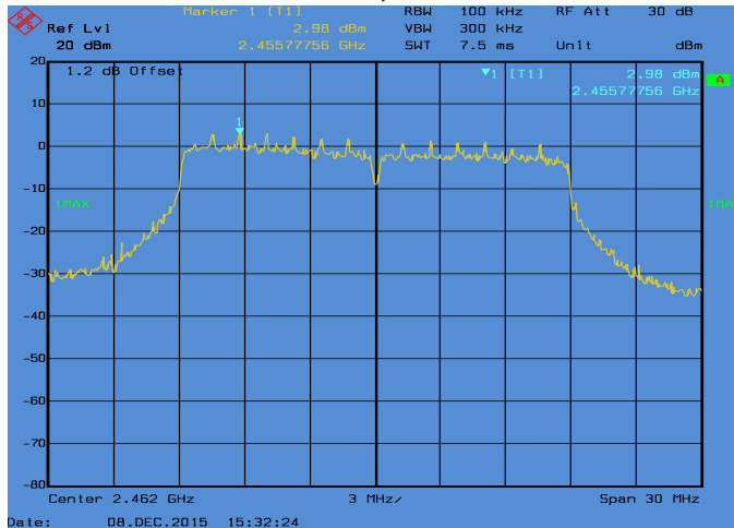
Conducted Emissions. 802.11n_20, Frequency 2462 MHz Reference Level
