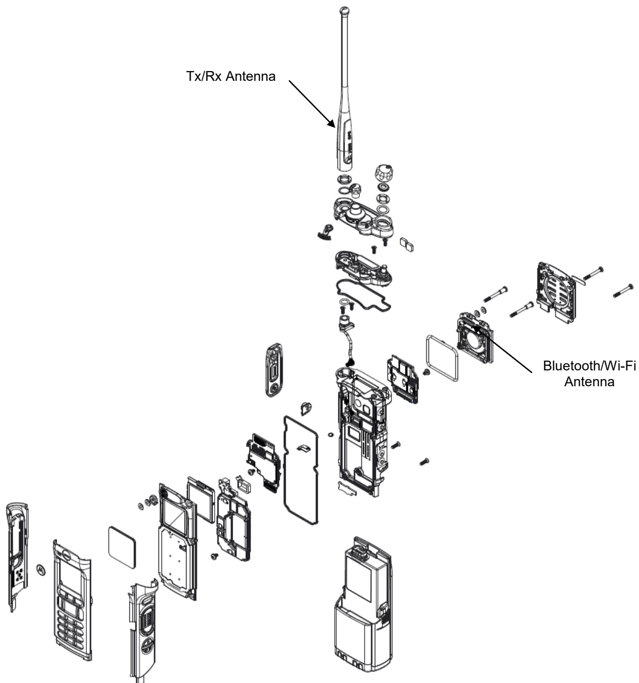
Exploded view of Model 3.5
