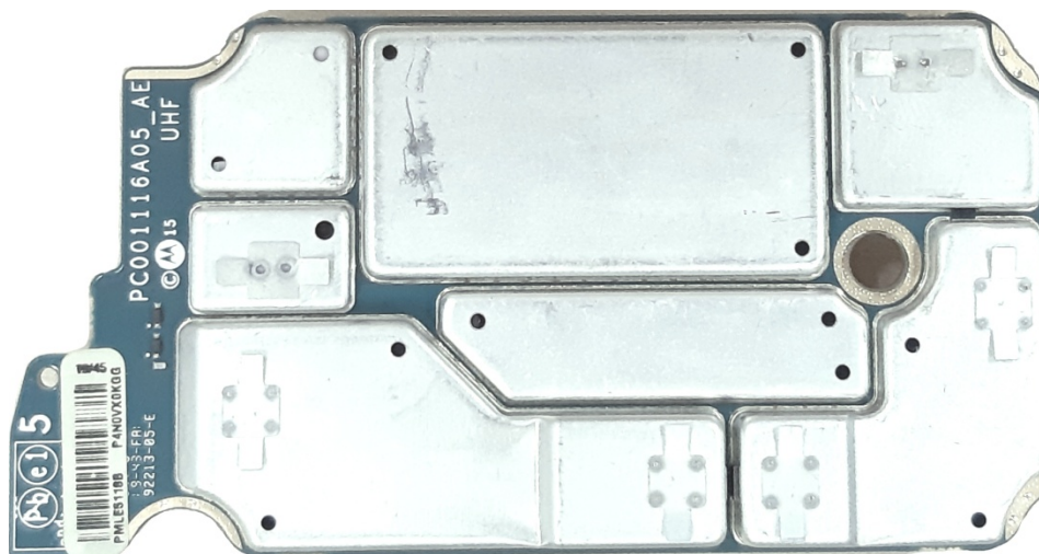
RF board with Shields (Top)
