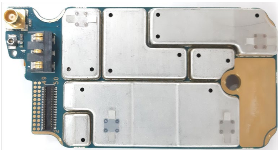
RF board with Shields (Bottom)
