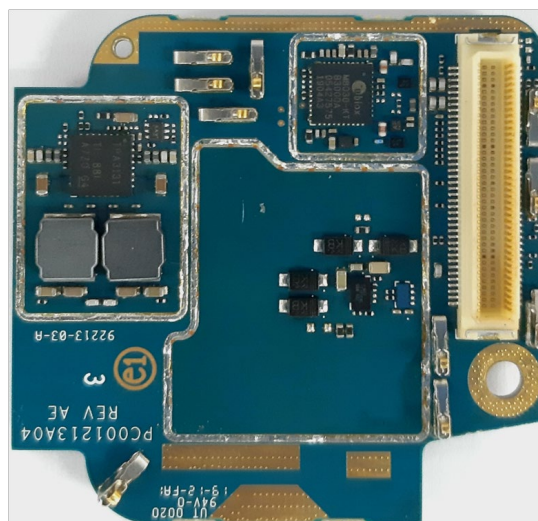
Expansion board without shields (Bottom)
