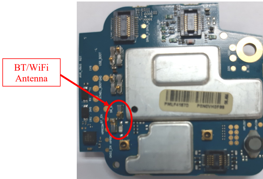
Expansion board with shields (Top)
