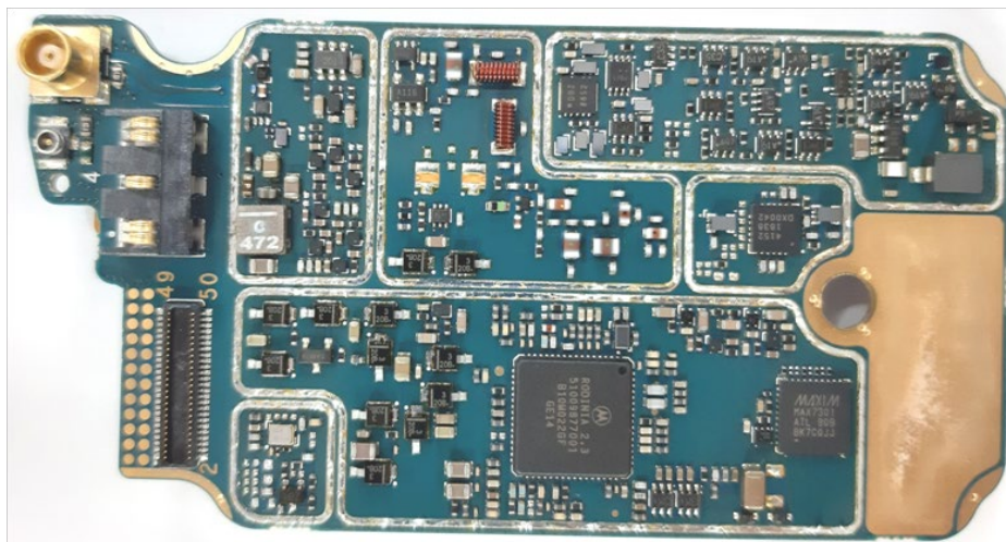
RF board without Shields (Bottom)
