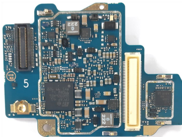
Vocon board without shields (Bottom)
