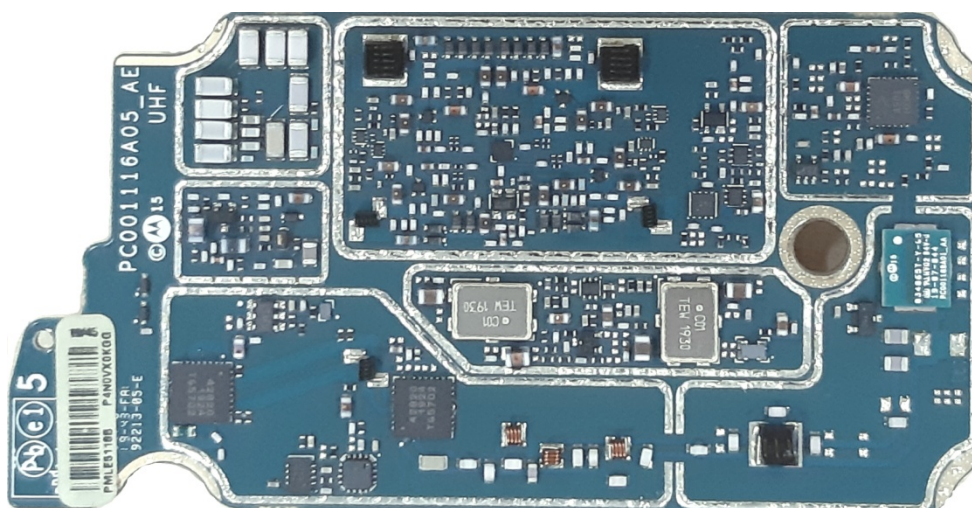
RF board without Shields (Top)
