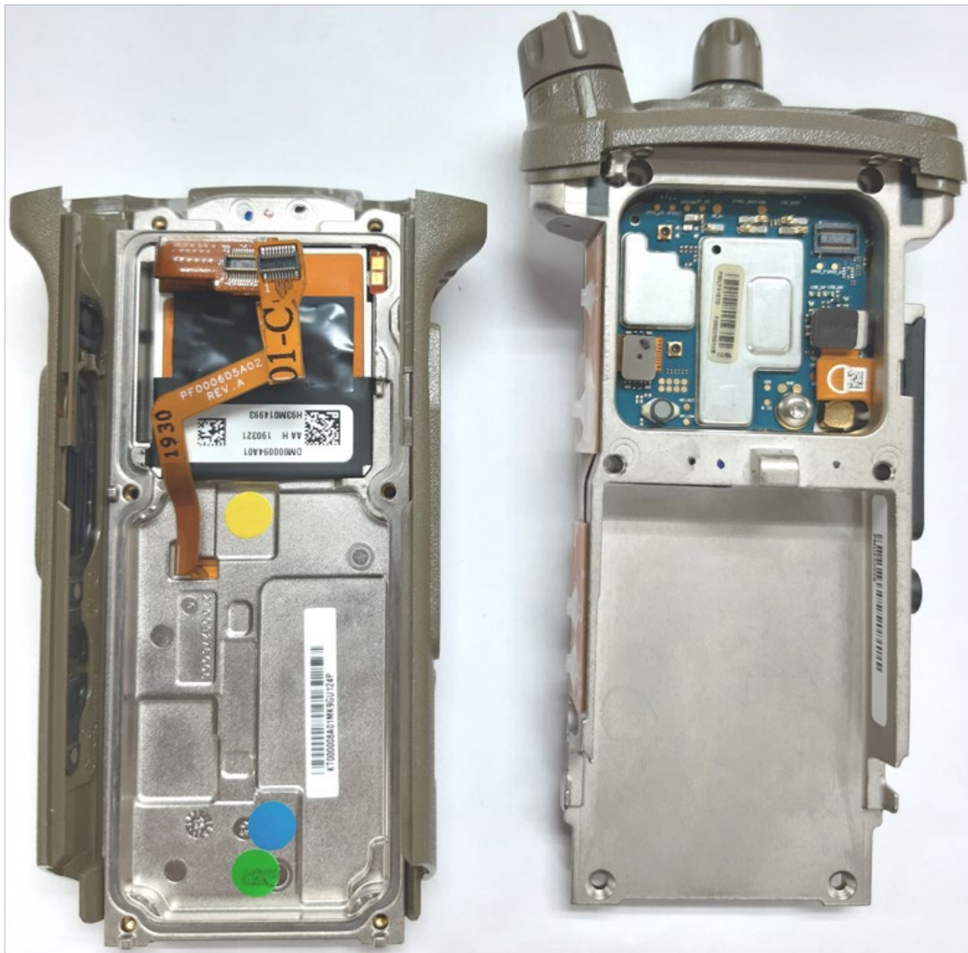
Expansion board with chassis and housing of Model 3.5 (Back side)
