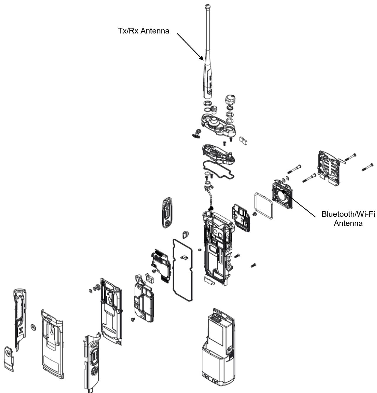
Exploded view of Model 1.5
