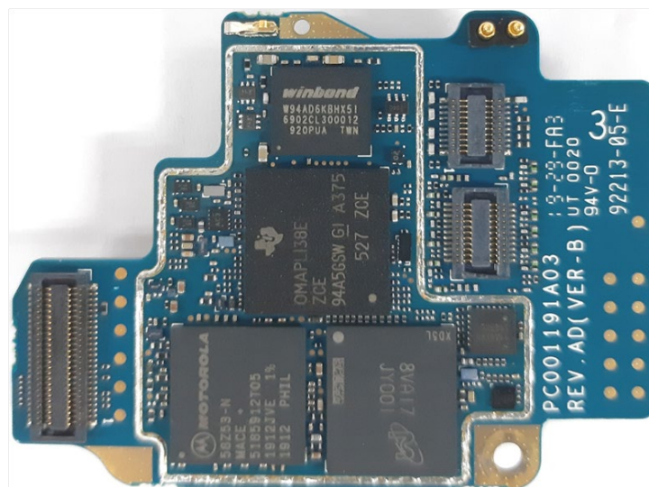
Vocon board without shields (Top)
