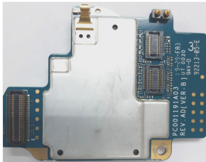
Vocon board with shields (Top)
