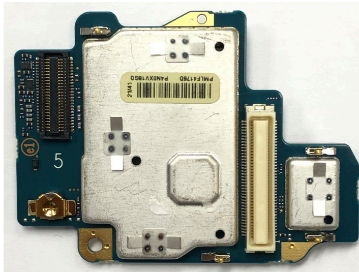
Vocon board with shields (Bottom)
