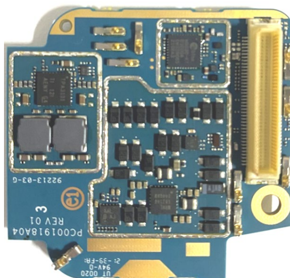
Expansion board without shields (Bottom)
