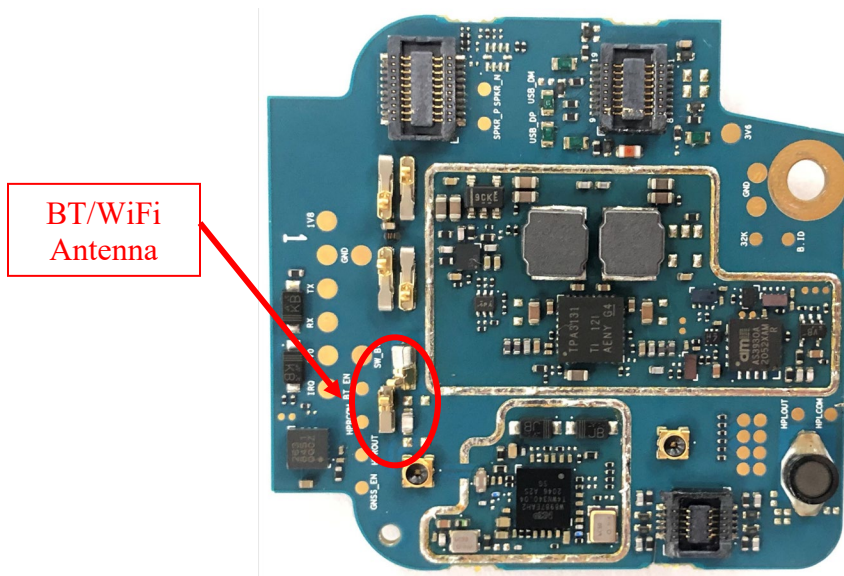
Expansion board without shields (Top)
