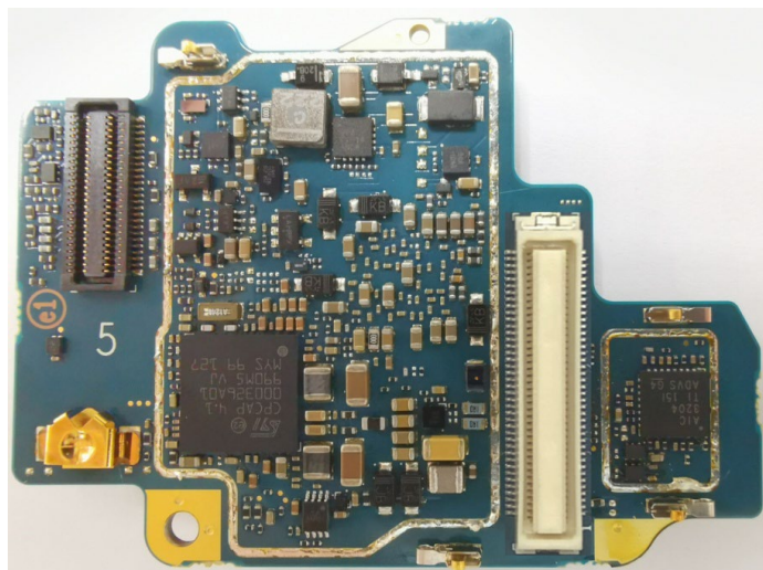
Vocon board without shields (Bottom)
