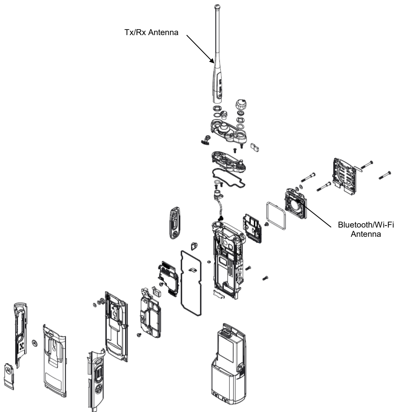
Exploded view of Model 1.5
