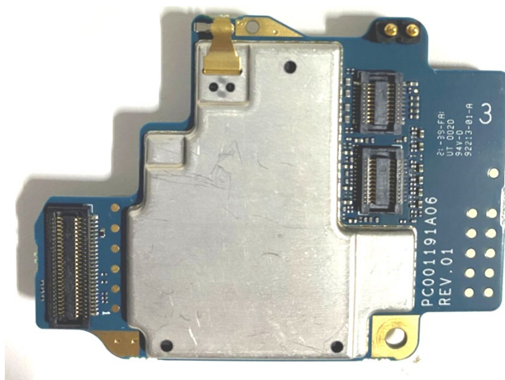
Vocon board with shields (Top)
