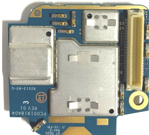
Expansion board with shields (Bottom)
