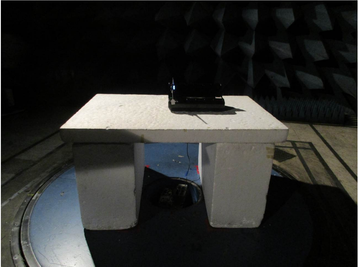
Figure 3: Radiated Emissions – Front View – Below 1 GHz
