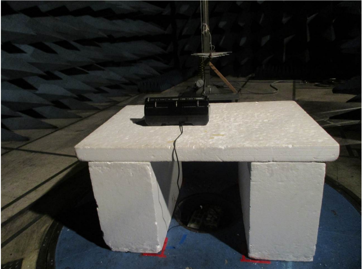
Figure 6: Radiated Emissions – Back View – 200 MHz – 1 GHz
