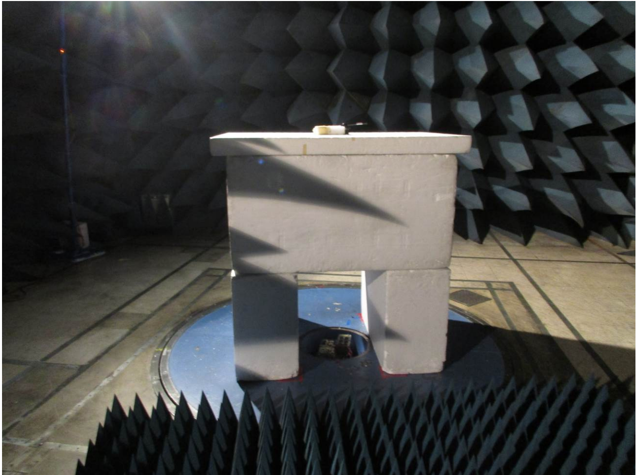
Figure 1: Radiated Band Edge Emissions – Front View
