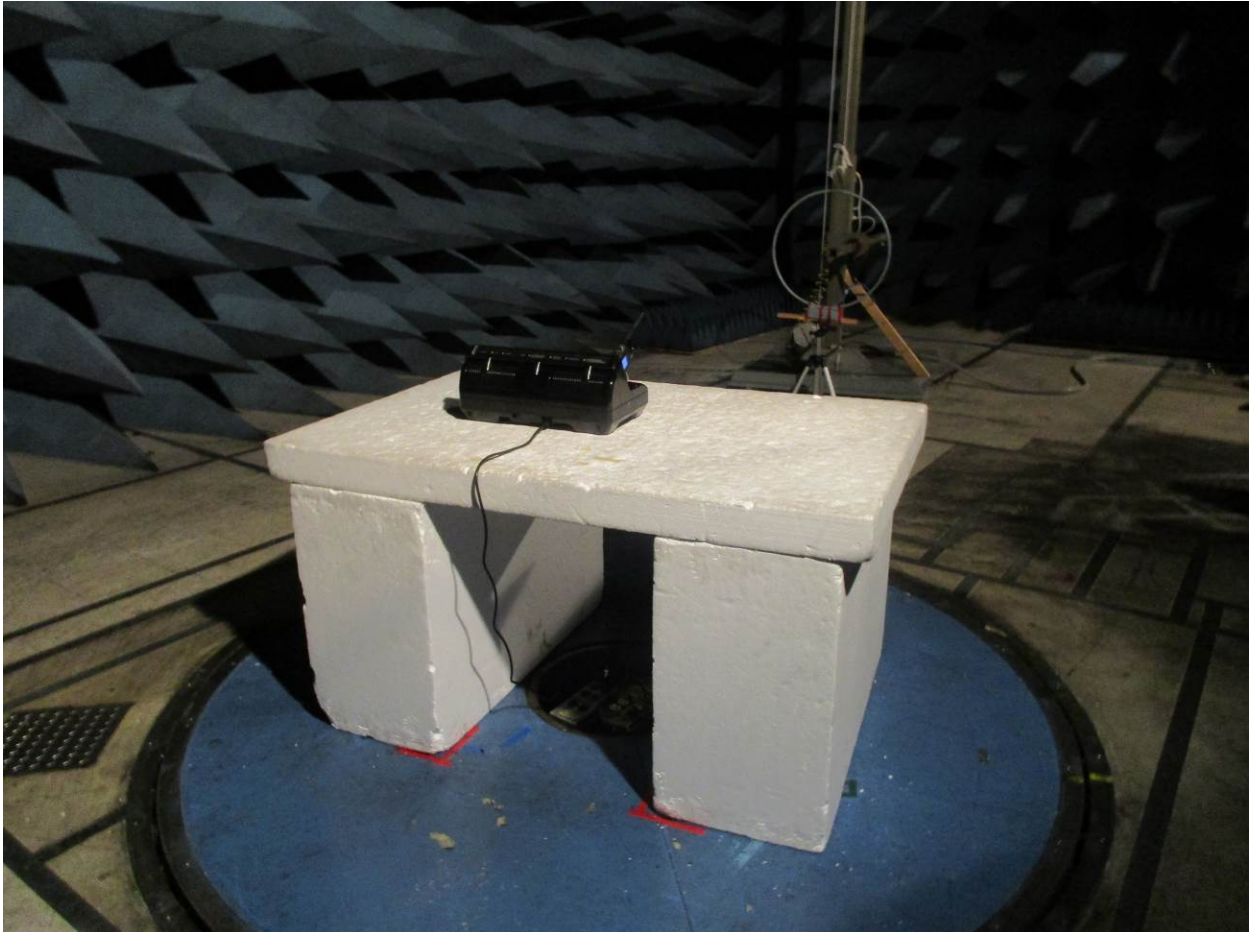
Figure 4: Radiated Emissions – Back View – 9 kHz – 30 MHz
