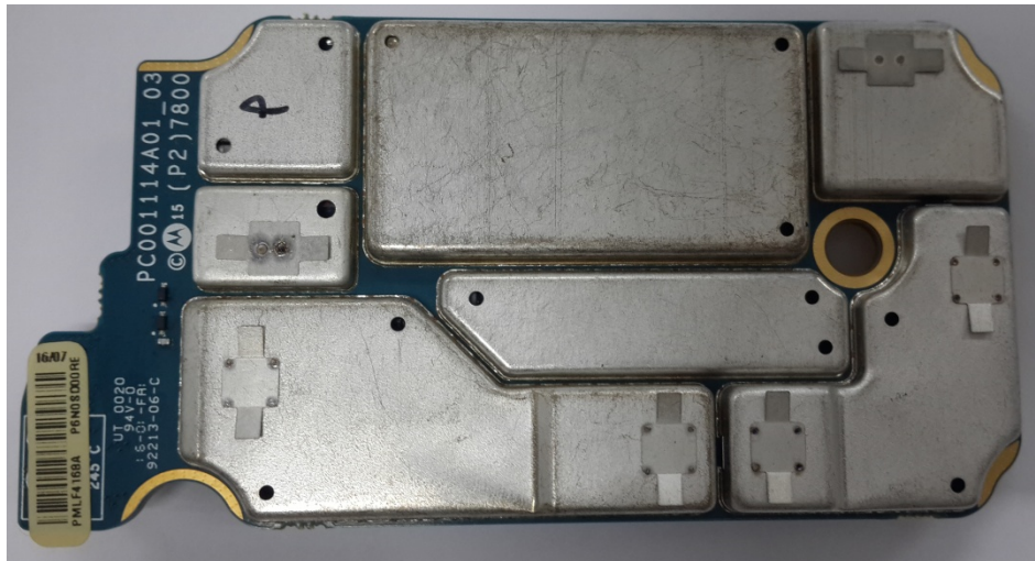
RF board with Shields (Top) (APX6000/APX5000/APX6000XE/APX6000Li/SRX2200)
