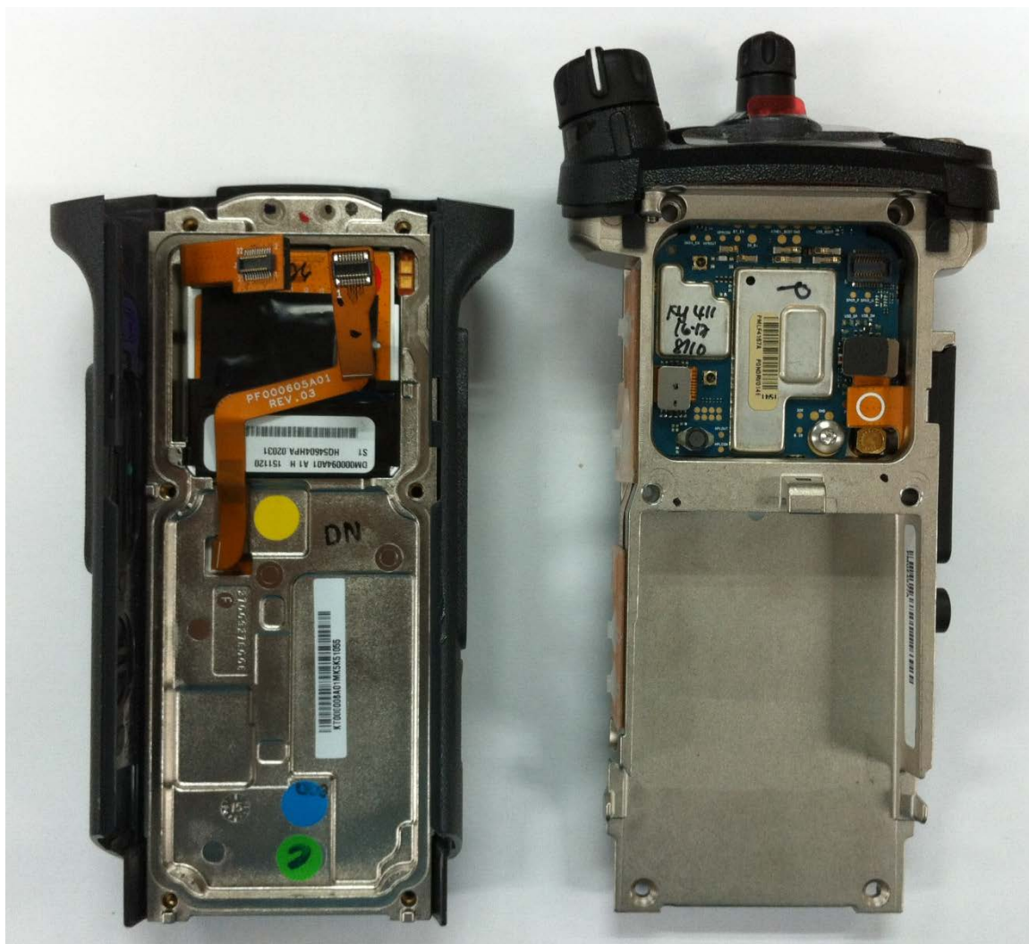
Expansion board with chassis and housing of APX6000/APX6000Li/APX5000 Model 3.5 (Back side)
