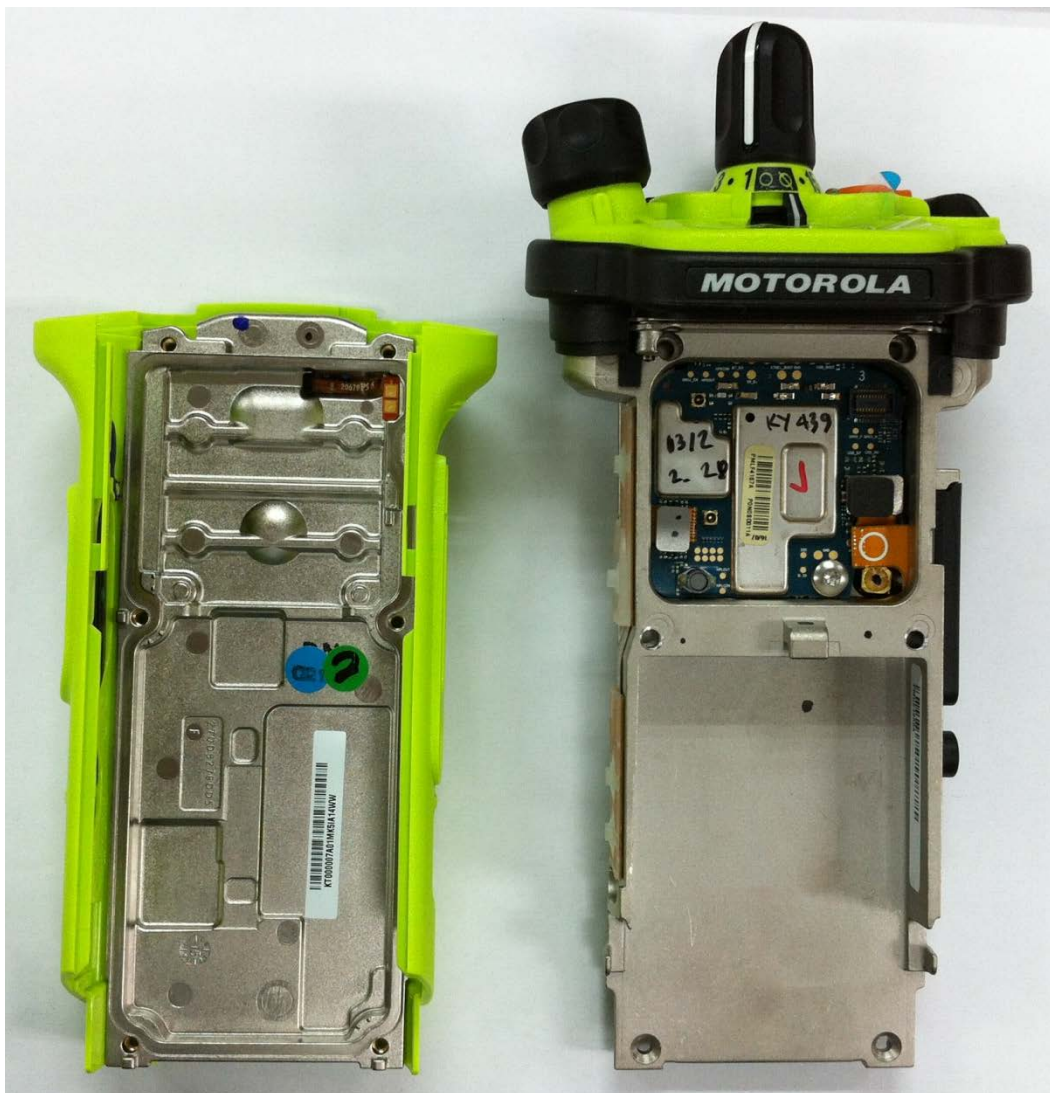
Expansion board with chassis and housing of APX6000XE Model 1.5 (Back side)
