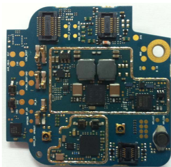
Expansion board without shields (Top) (APX6000/APX5000/APX6000XE/APX6000Li/SRX2200)
