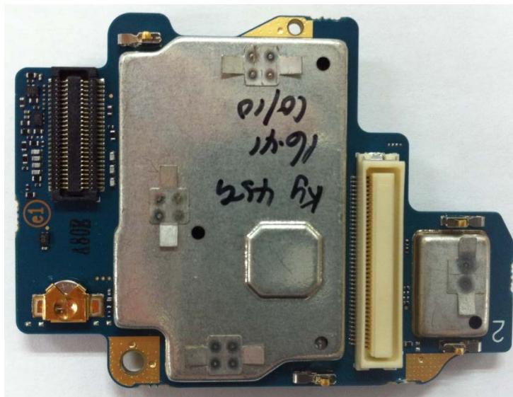
Vocon board with shields (Bottom) (APX6000/APX5000/APX6000XE/APX6000Li/SRX2200)
