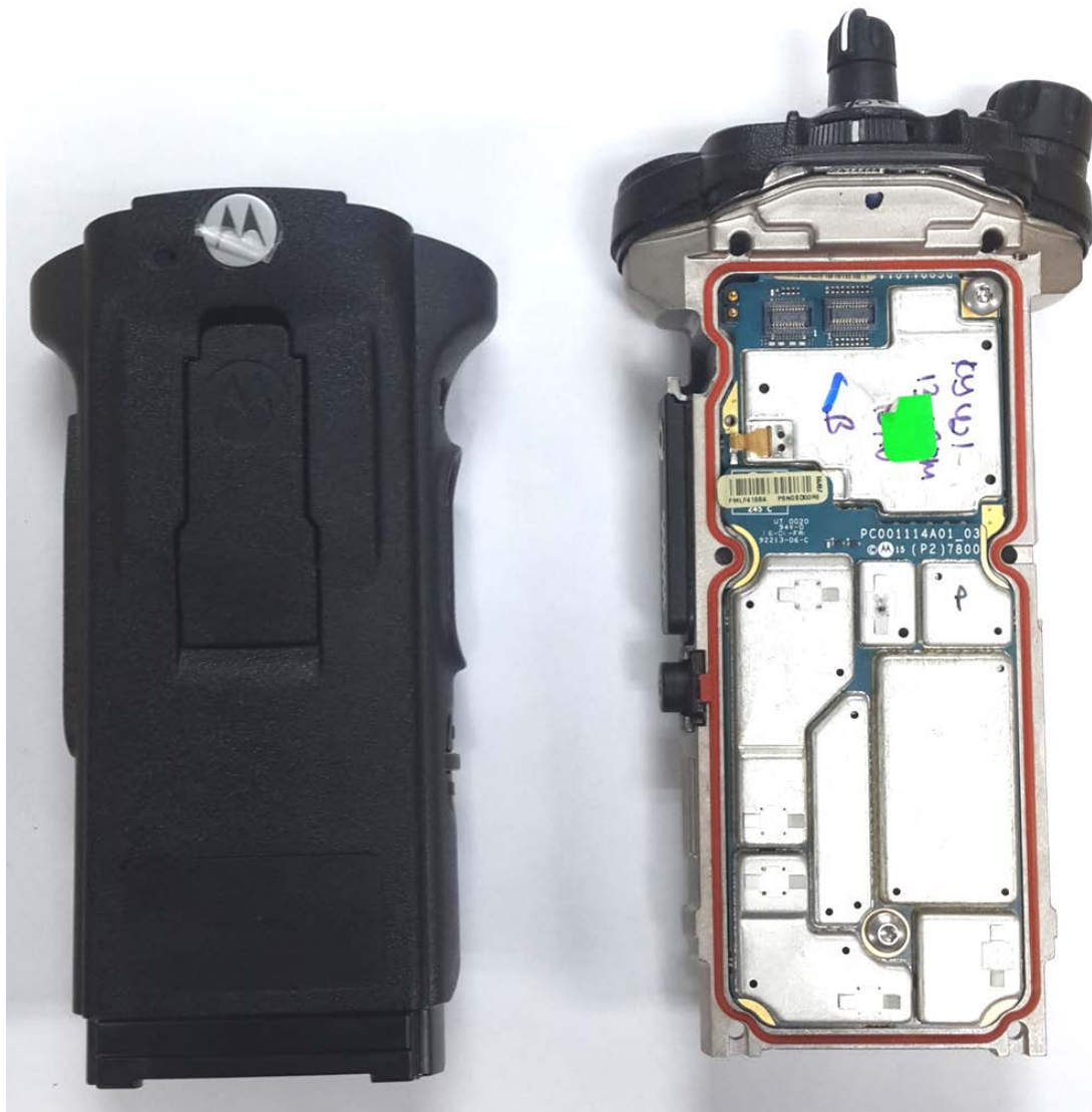
RF and Vocon boards with chassis and housing of APX6000/APX6000Li/APX5000 Model 1.5 (Front side)
