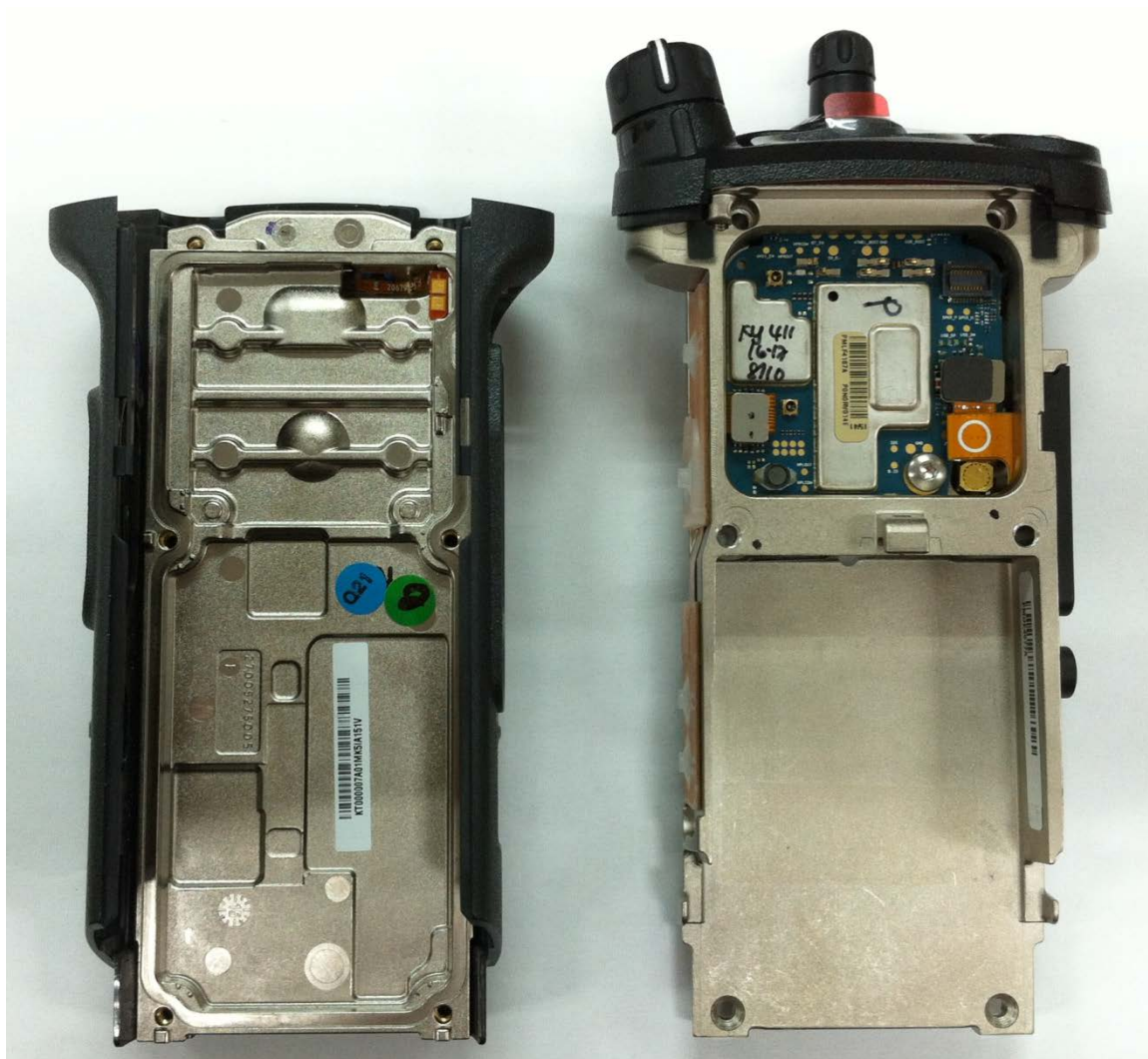
Expansion board with chassis and housing of APX6000/APX6000Li/APX5000 Model 1.5 (Back side)
