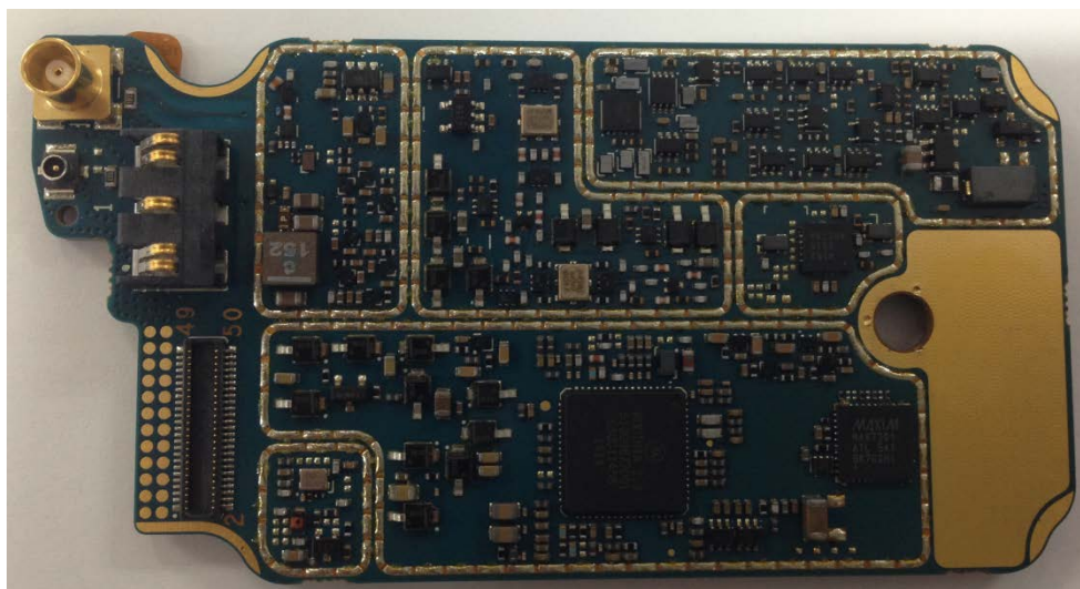
RF board without Shields (Bottom) (APX6000/APX5000/APX6000XE/APX6000Li/SRX2200)
