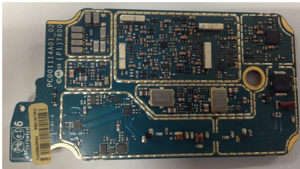
RF board without Shields (Top) (APX6000/APX5000/APX6000XE/APX6000Li/SRX2200)
