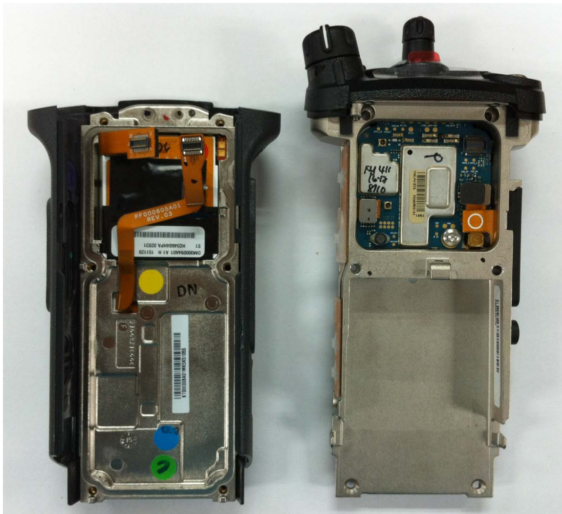
Expansion board with chassis and housing of APX6000/APX6000Li/APX5000 Model 2.5 (Back side)
