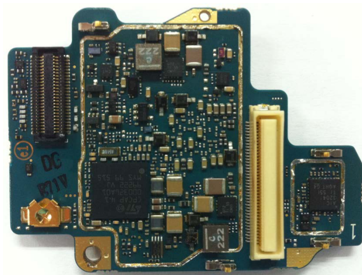
Vocon board without shields (Bottom) (APX6000/APX5000/APX6000XE/APX6000Li/SRX2200)
