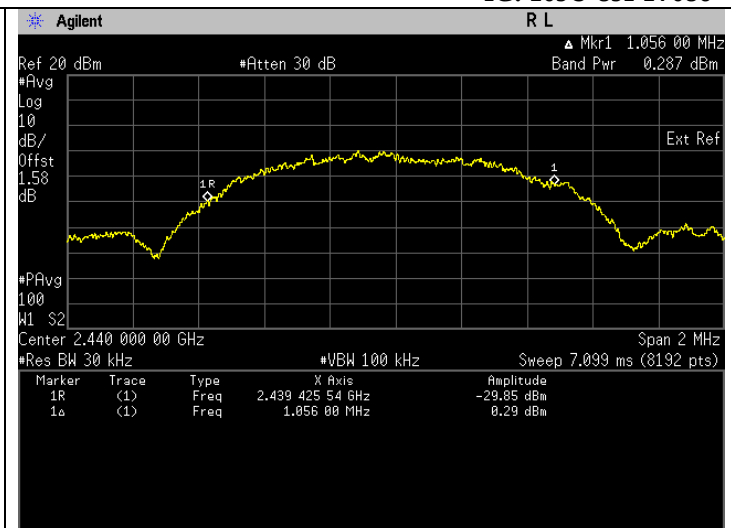
Frequency 2440 MHz
