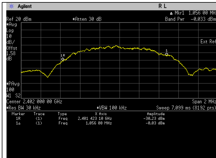
Frequency 2402 MHz
