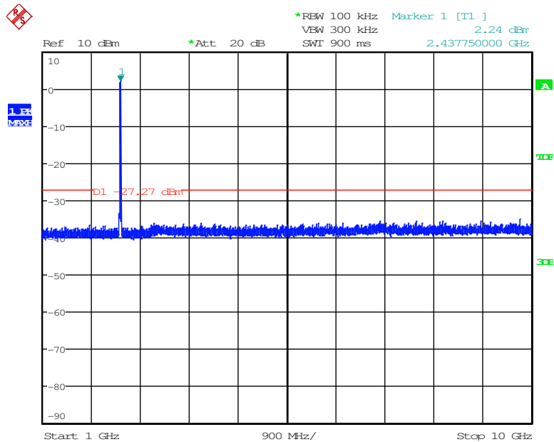
Figure 7.4.2.2-17: 30 MHz – 1 GHz –Middle Channel
