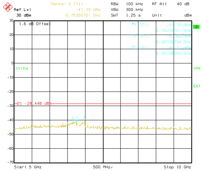
Date: 17.MAY 2019 16:08:43 Conducted Emissions. 802.11g, Frequency 2437 MHz Emission Level, 5 GHz -> 10 GHz
