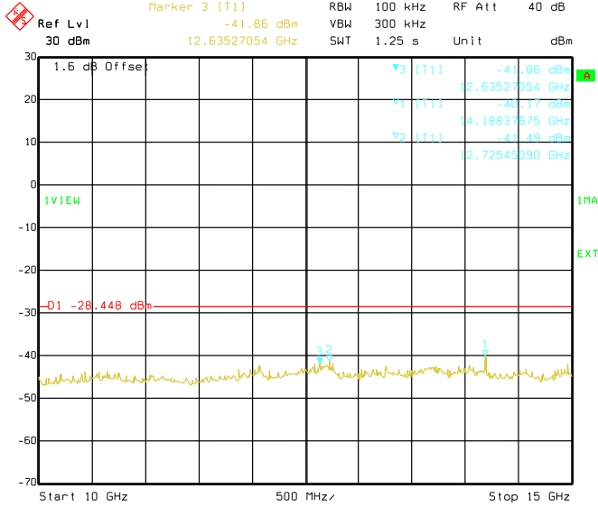
Date: 17.MAY 2019 16:09:37 Conducted Emissions. 802.11g, Frequency 2437 MHz Emission Level, 10 GHz -> 15 GHz
