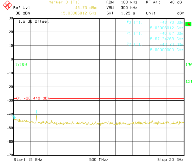
Date: 17.MAY 2019 16:10:29 Conducted Emissions. 802.11g, Frequency 2437 MHz Emission Level, 15 GHz -> 20 GHz
