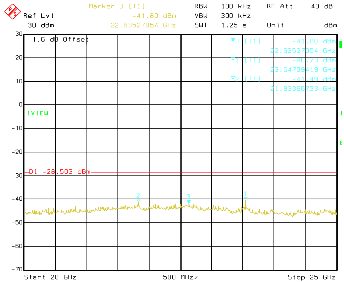
Date: 21.MAY 2019 14:31:07 Conducted Emissions. 802.11g, Frequency 2462 MHz Emission Level, 20 GHz -> 25 GHz
