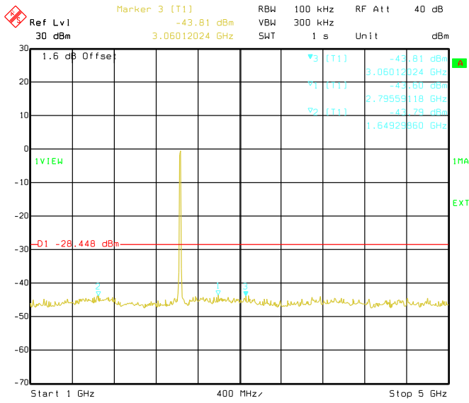
Date: 17.MAY 2019 16:07:50 Conducted Emissions. 802.11g, Frequency 2437 MHz Emission Level, 1 GHz -> 5 GHz
