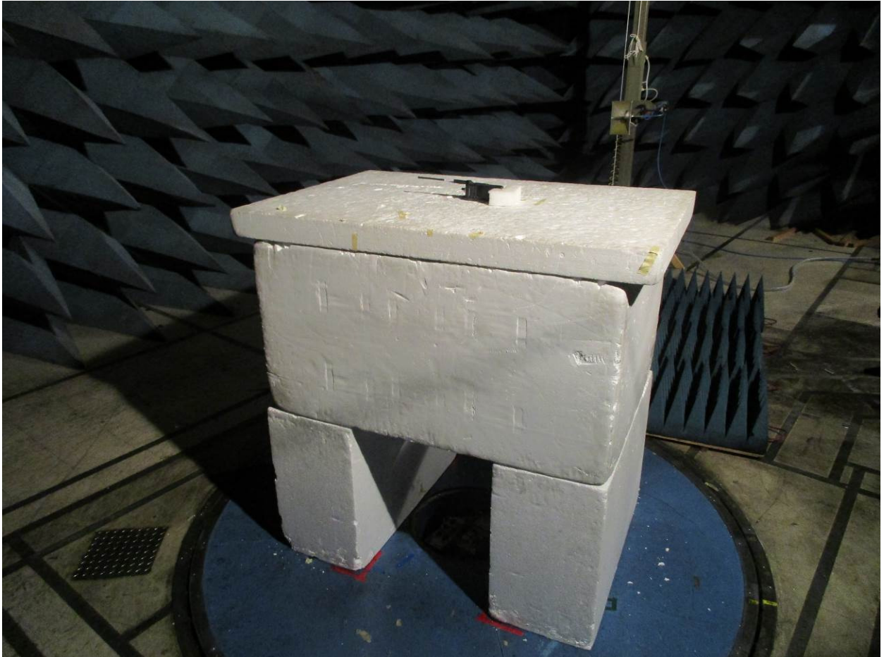
Figure 2: Radiated Emissions – Back View – Band Edge
