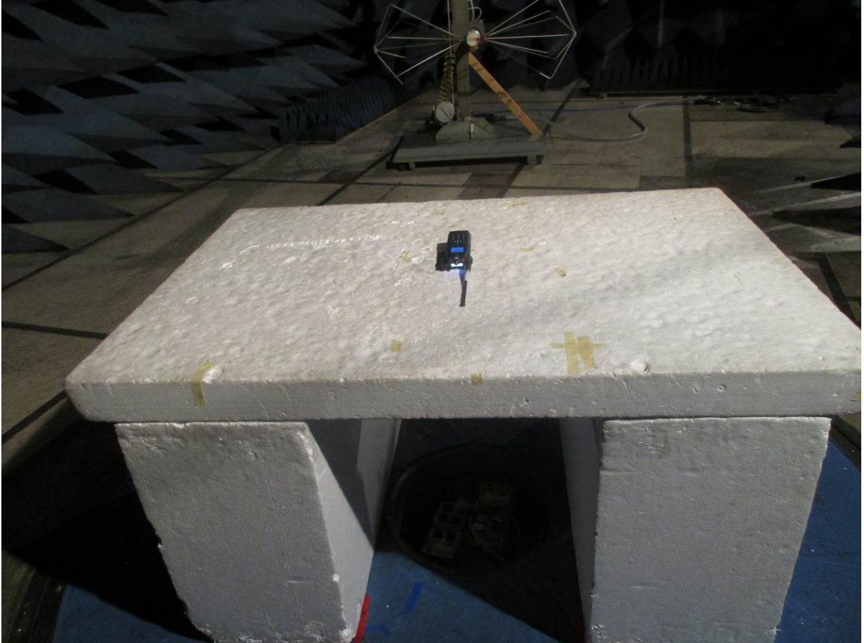
Figure 5: Radiated Emissions – Back View – 30 MHz – 200 MHz
