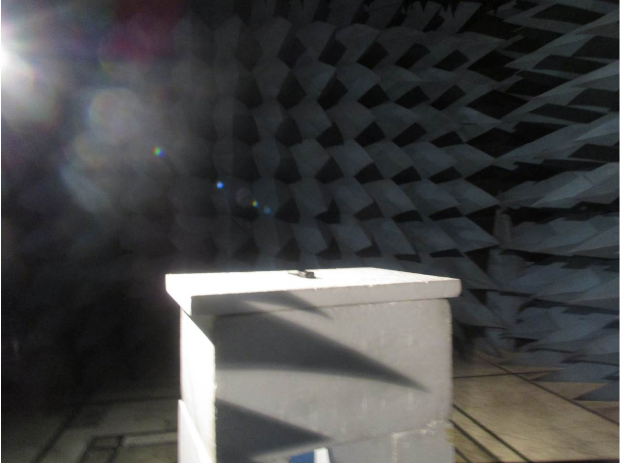
Figure 7: Radiated Emissions – Front View – Above 1 GHz
