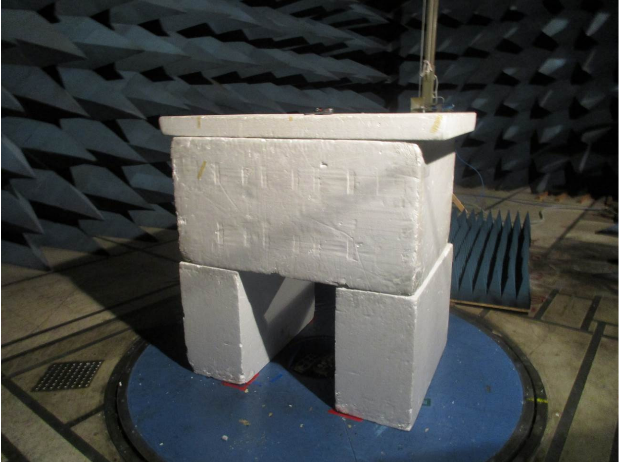
Figure 8: Radiated Emissions – Back View – Above 1 GHz
