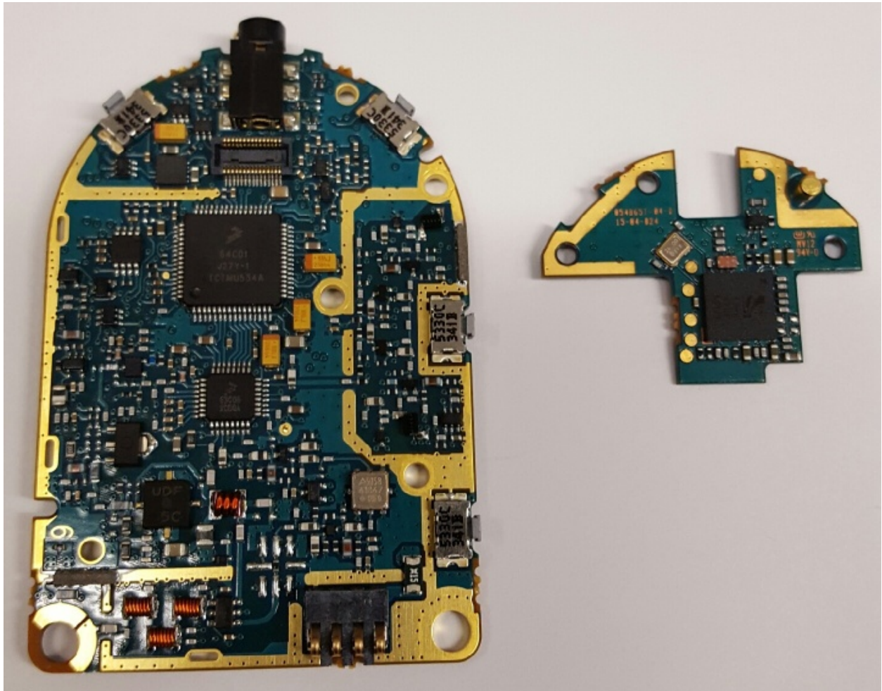
Bottom View with Shield removed
