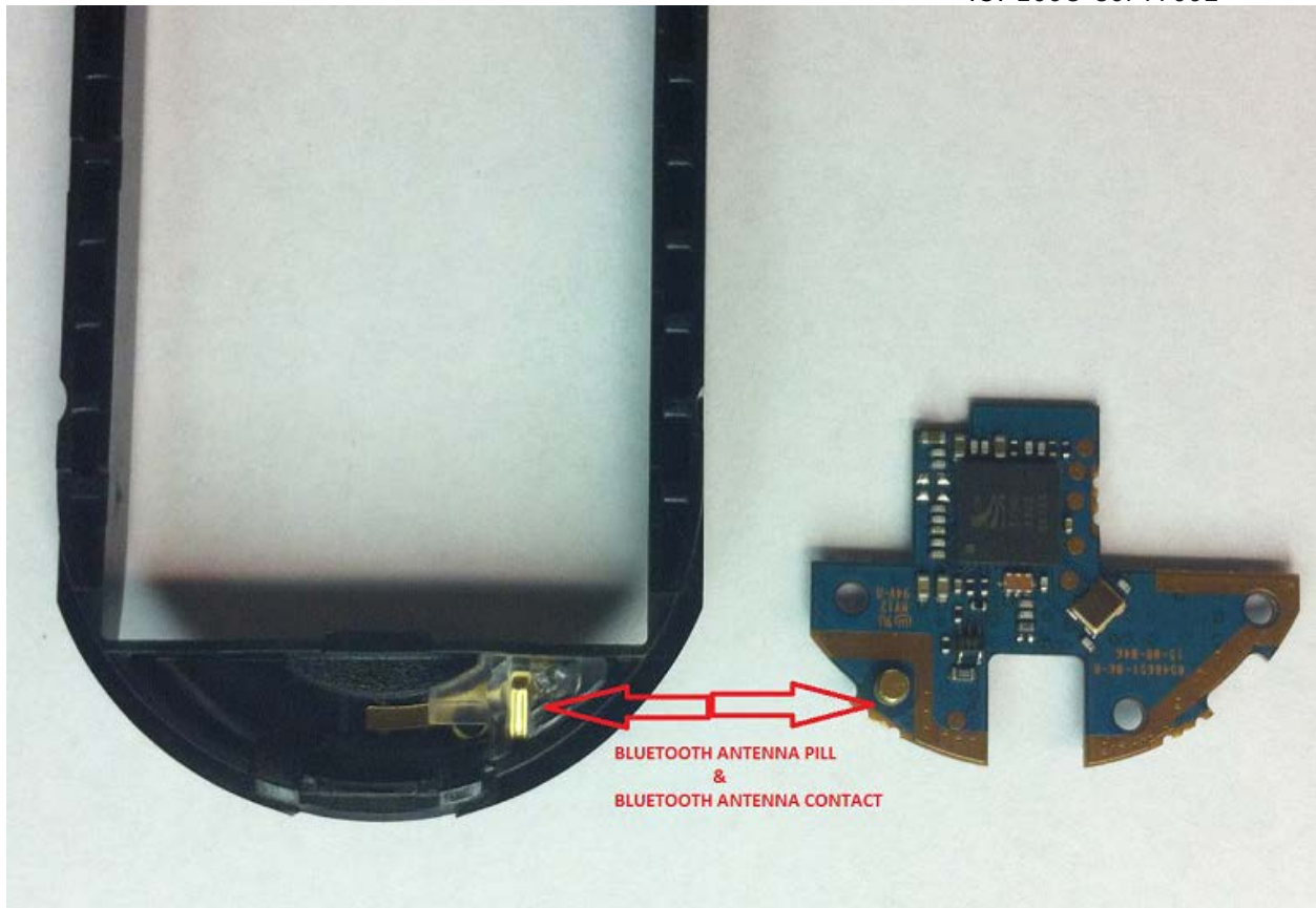
BLUETOOTH ANTENNA LOCATION
