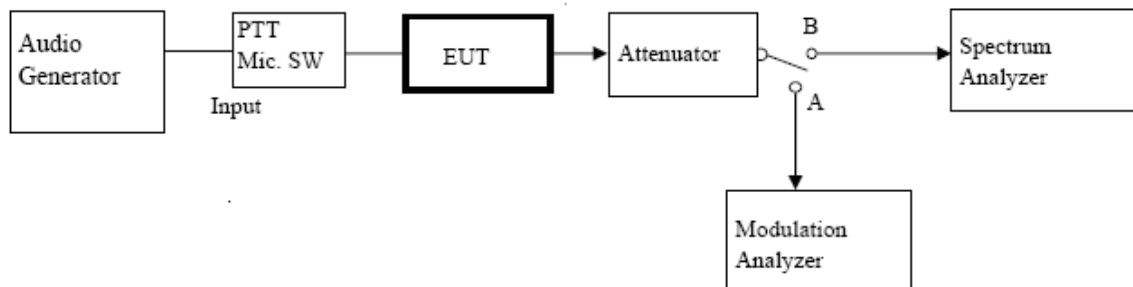
Figure 2. Occupied Bandwidth and Emission Mask Setup
