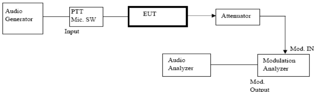
Figure 1. Audio Response setup
