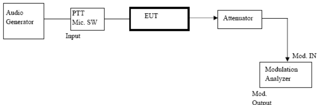
Figure 1. Modulation limiting setup
