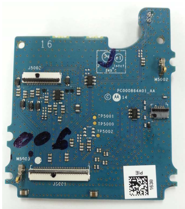
Interface board (Bottom) (APX1000+)
