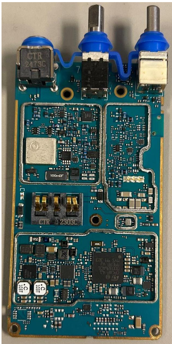
RF board without Shields (Bottom) H92QDF9PW6AN (APX 900)
