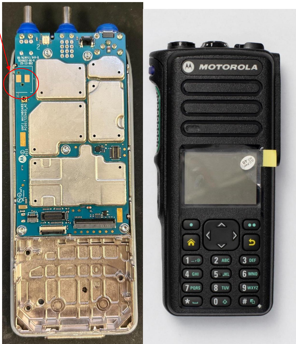
RF boards with chassis and housing (Front Side) H92QDH9PW7AN (APX 900)
