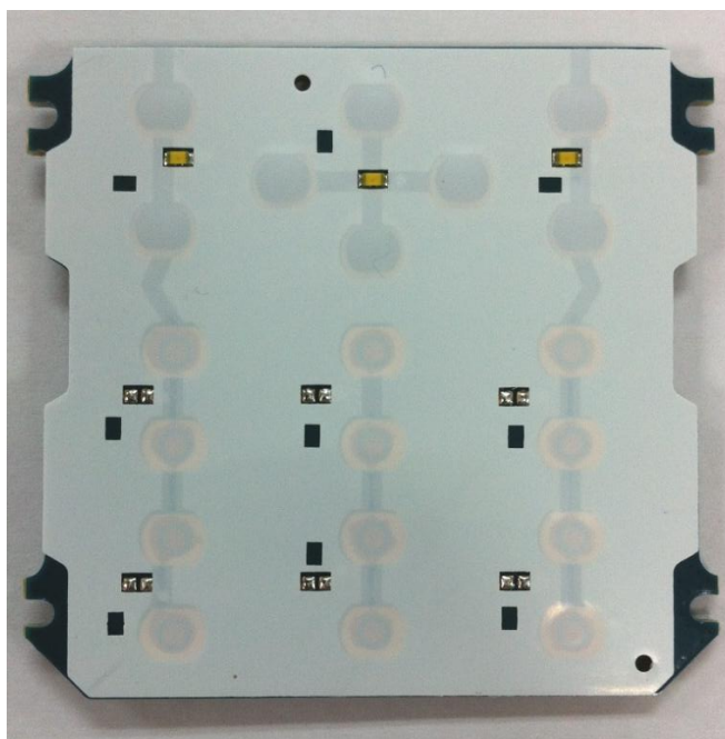
Keypad Board (Top), H92QDF9PW6AN (APX900)
