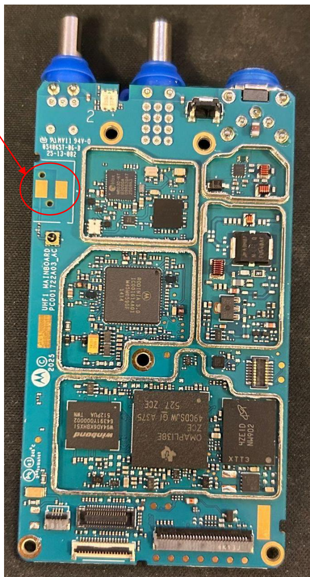
RF board without Shields (Top) H92QDH9PW7AN (APX 900)
