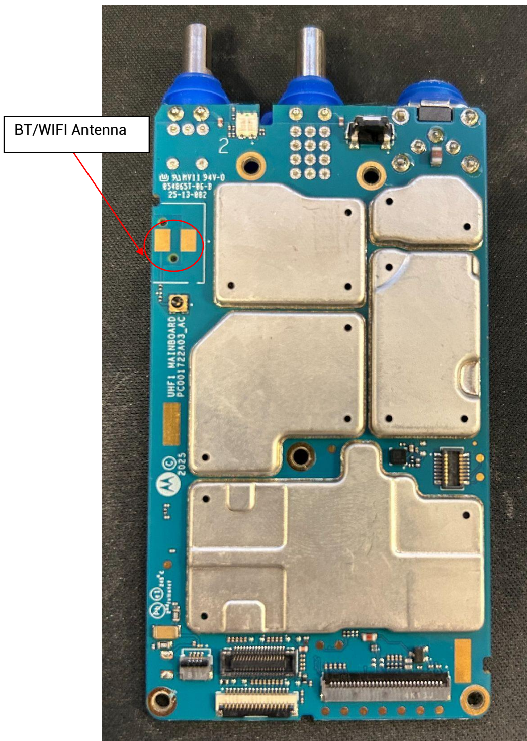
RF board with Shields (Top) H92QDF9PW6AN (APX 900)
