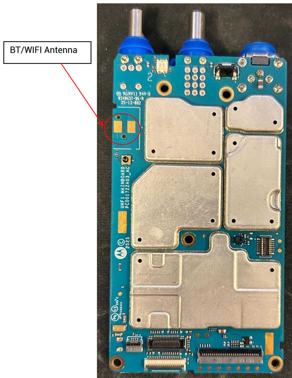
RF board with Shields (Top) H93QDH9PW7AN (VX-P 949)
