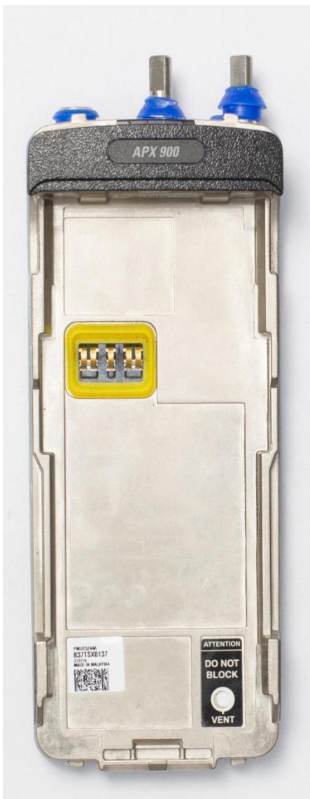
Chassis and housing for (Back Side), H92QDH9PW7AN (APX 900)
