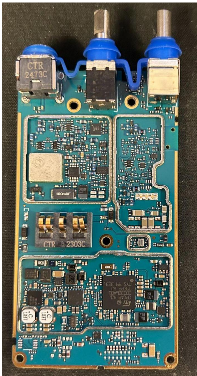
RF board without Shields (Bottom) H93QDH9PW7AN (VX-P 949)
