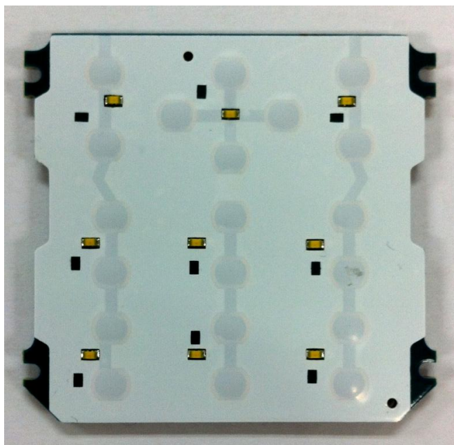
Keypad Board (Top), H92QDH9PW7AN (APX900)
