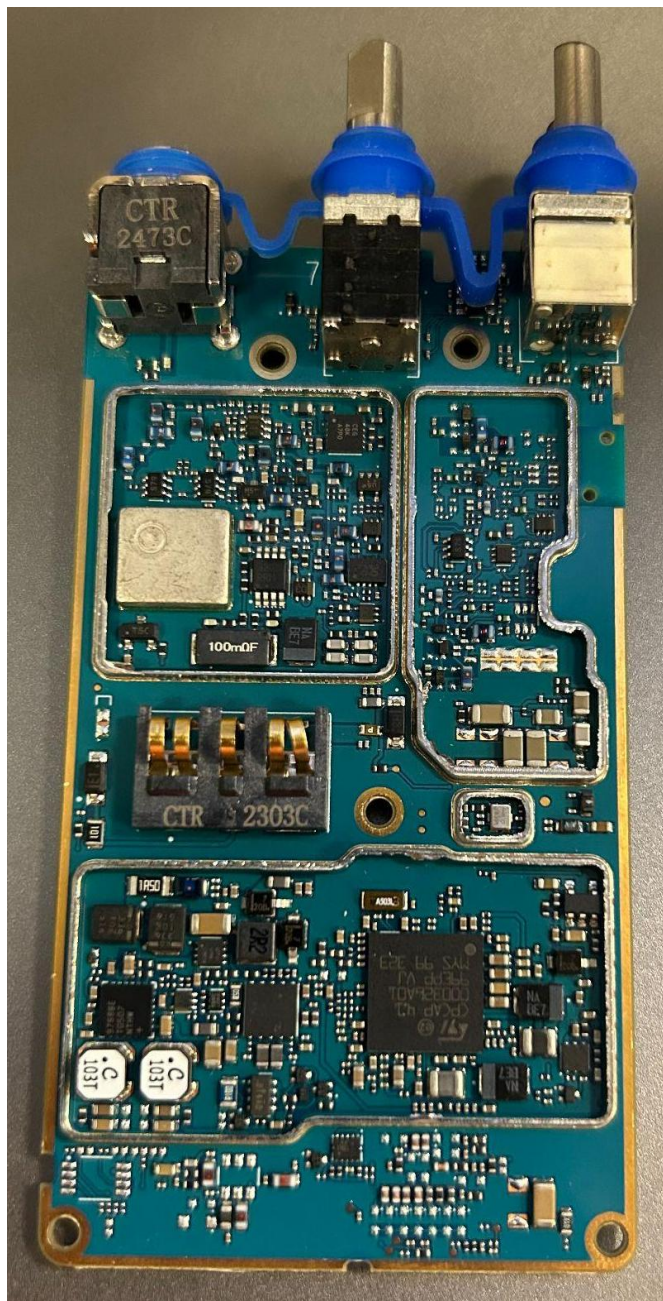
RF board without Shields (Bottom) H92QDH9PW7AN (APX 900)
