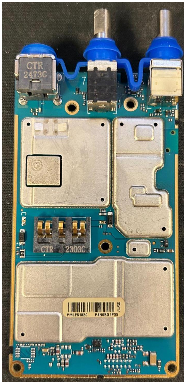
RF board with Shields (Bottom) H92QDH9PW7AN (APX 900)
