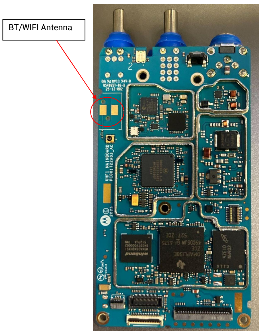
RF board without Shields (Top) H93QDH9PW7AN (VX-P 949)
