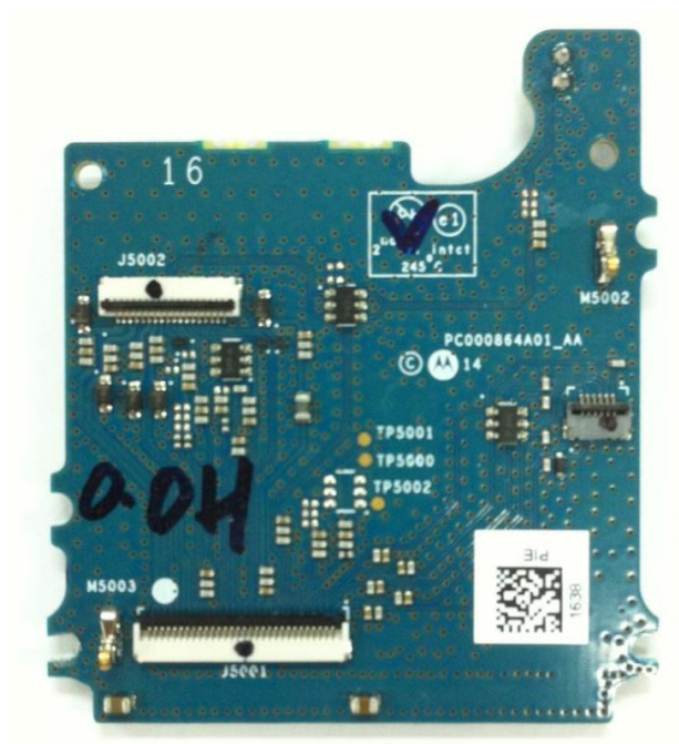
Interface Board (Bottom) H93QDH9PW7AN (VX-P949)
