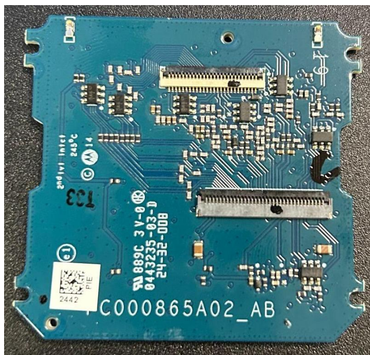
Keypad Board (Bottom) H93QDH9PW7AN (VX-P949)
