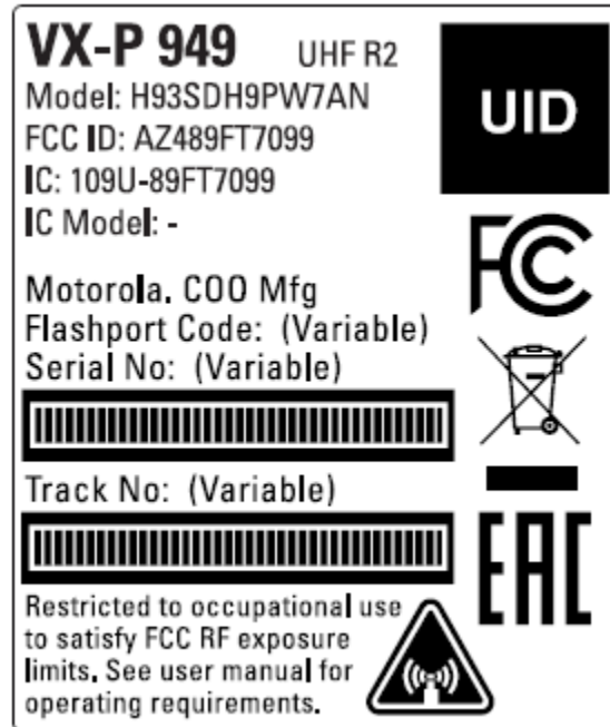
Figure 1C: FCC/IC Label for VX-P949 Model 3 (Full Keypad)
