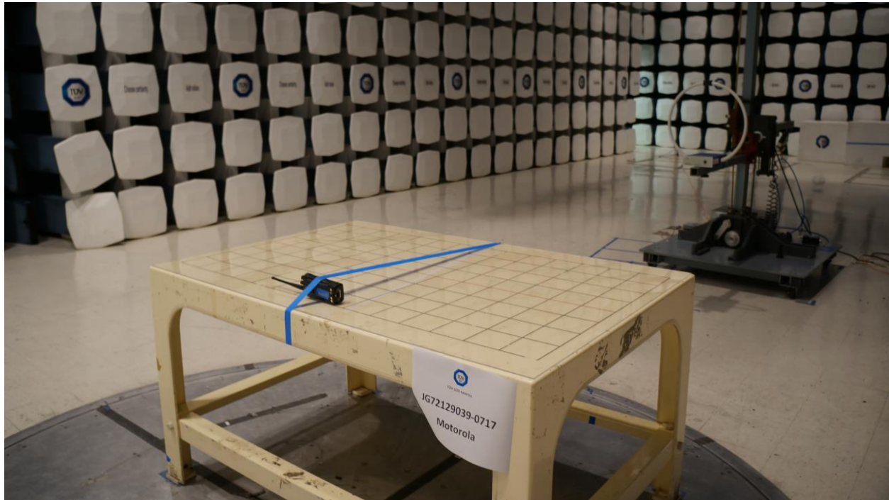
Radiated Emissions Test Setup (Below 30 MHz - Back)
