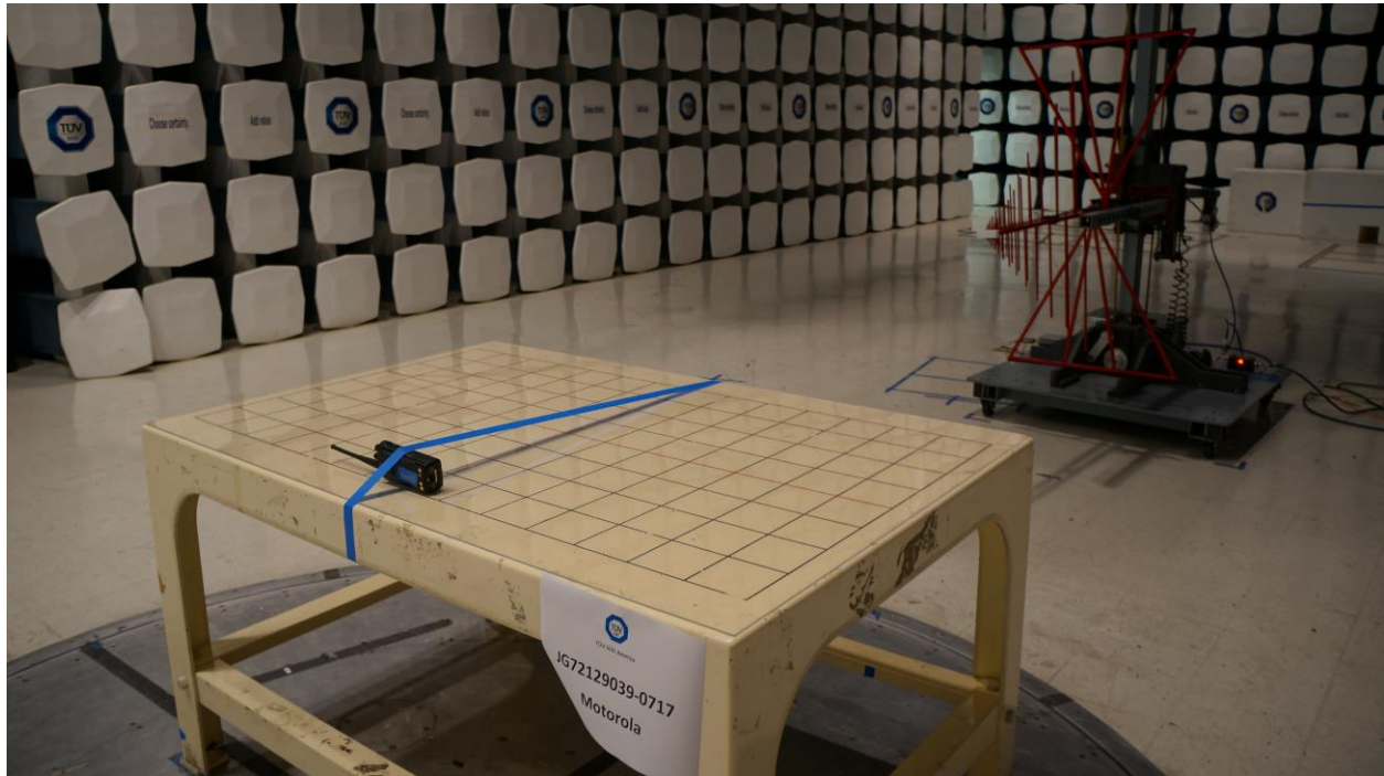
Radiated Emissions Test Setup (Below 1000 MHz - Back)
