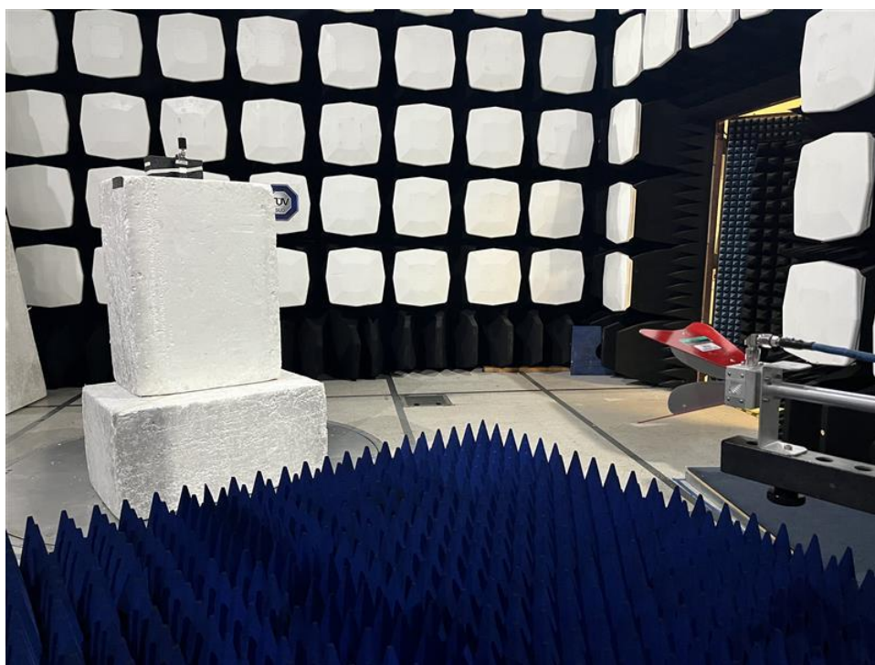
Figure A-6: Test Setup – Radiated Emissions > 1GHz
