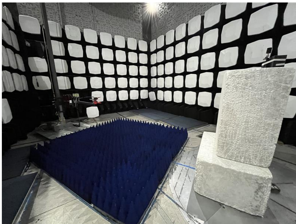
Figure A-5: Test Setup – Radiated Emissions > 1GHz
