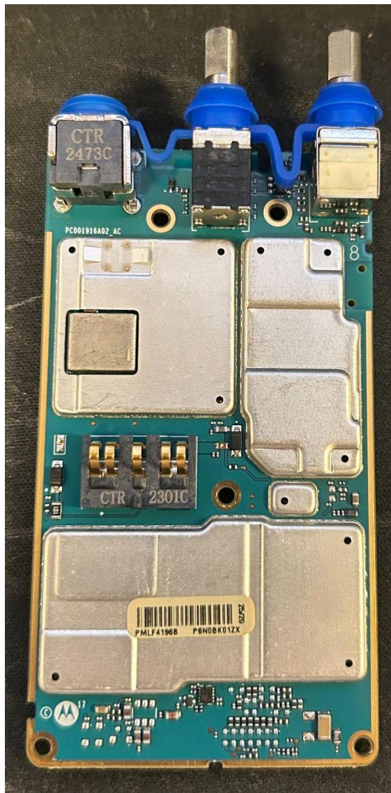
RF board with Shields (Bottom) H92WCH9PW7AN (APX 900)
