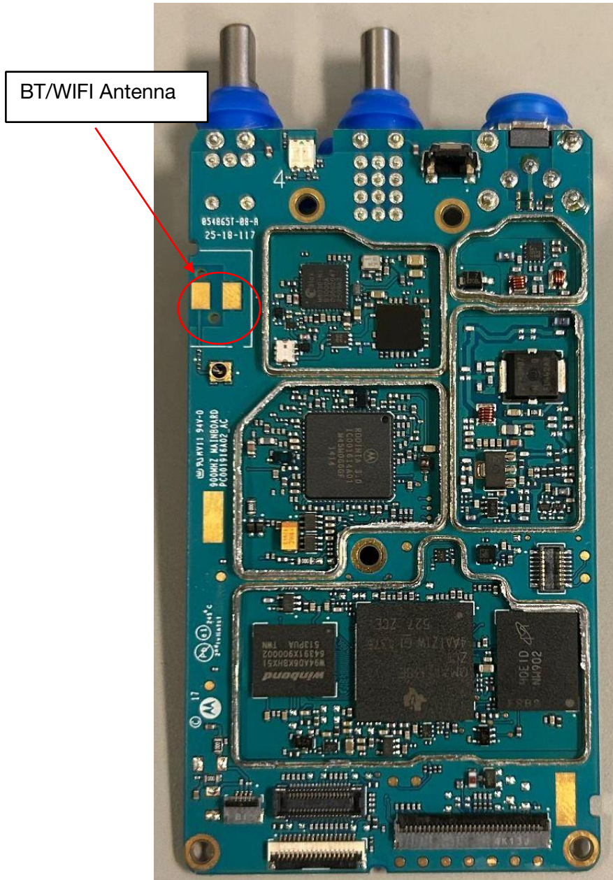
RF board without Shields (Top) H92WCH9PW7AN (APX 900)
