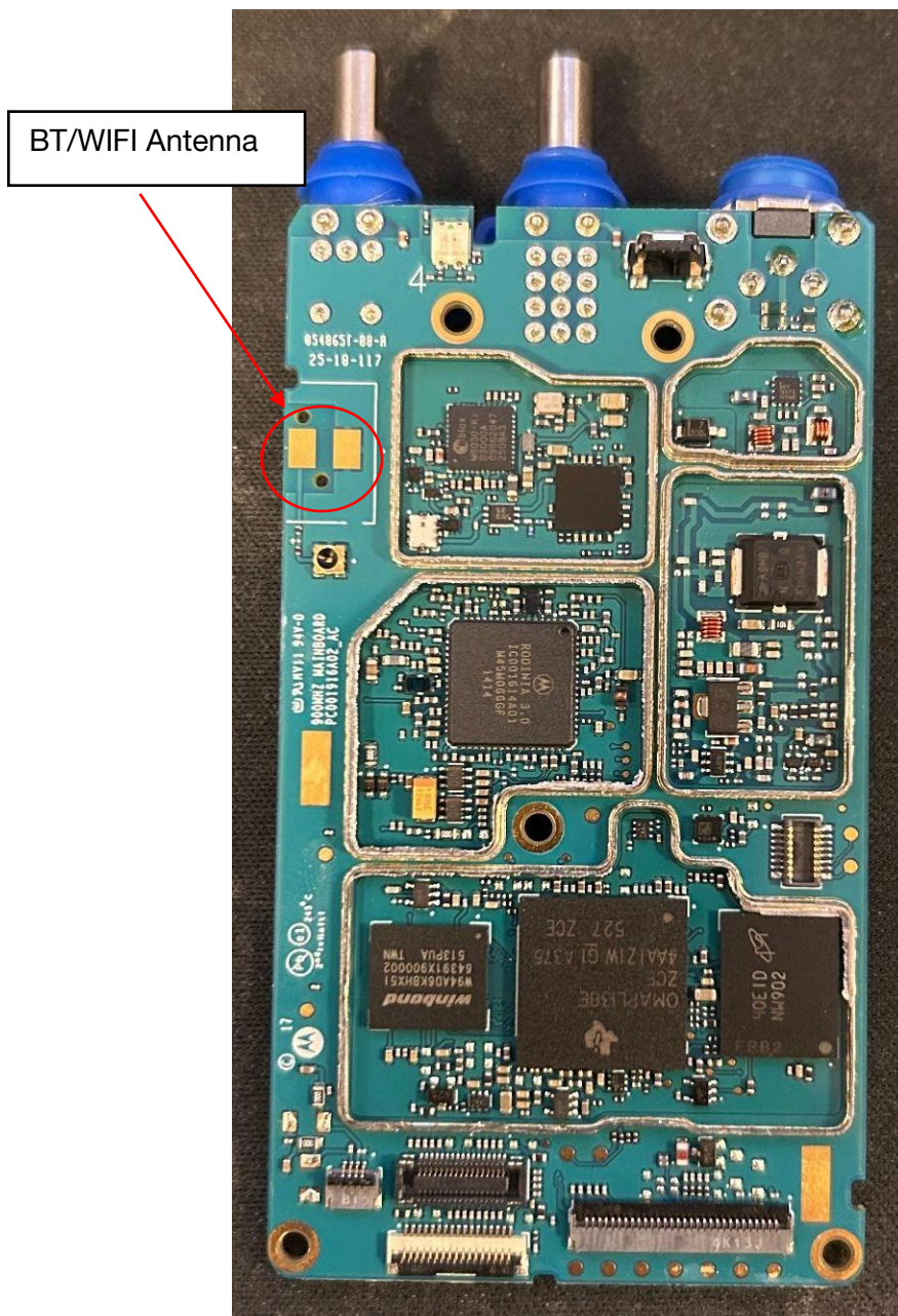
RF board without Shields (Top) H92WCF9PW6AN (APX 900)
