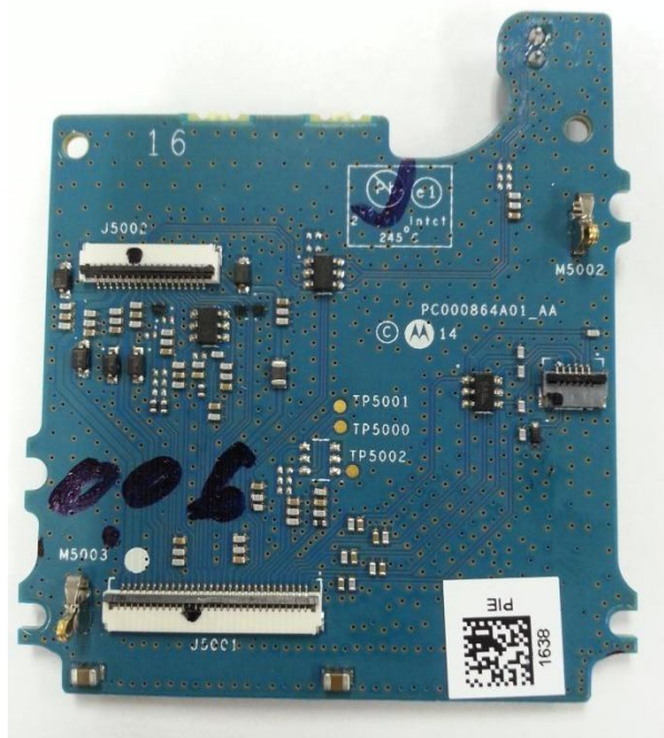
Interface board (Bottom) H92WCF9PW6AN (APX 900)
