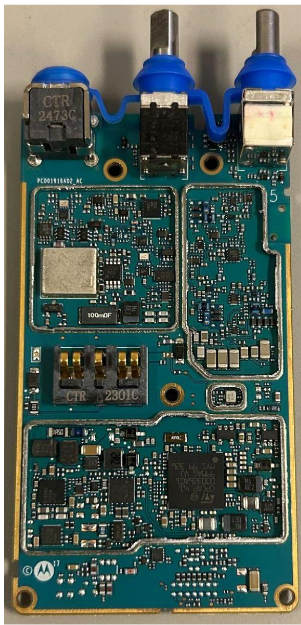
RF board without Shields (Bottom) H92WCF9PW6AN (APX 900)
