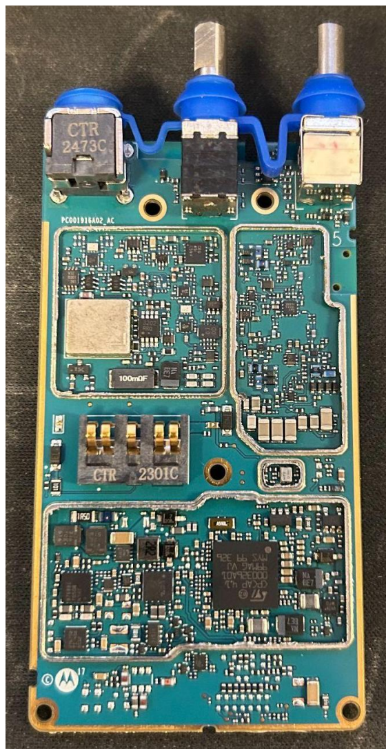
RF board without Shields (Bottom) H92WCH9PW7AN (APX 900)
