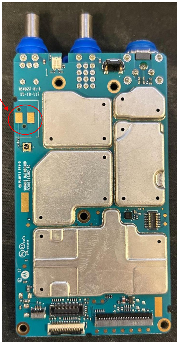
RF board with Shields (Top) H92WCH9PW7AN (APX 900)
