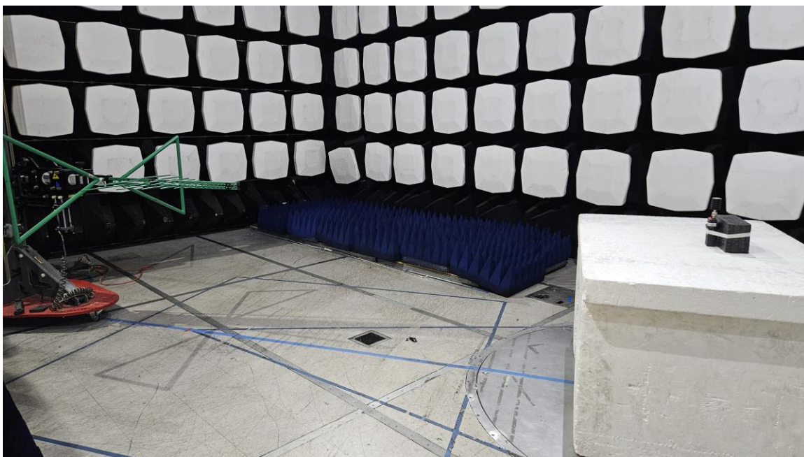
Figure A-4: Test Setup – Radiated Emissions < 1GHz
