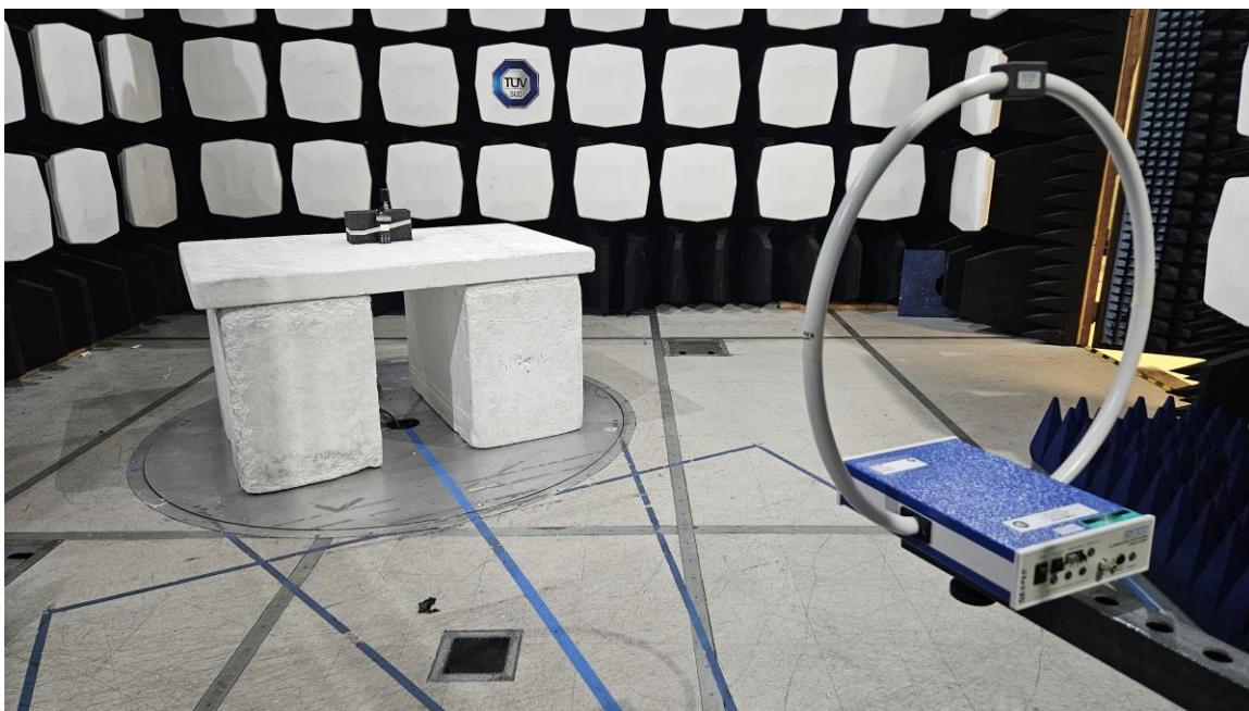
Figure A-1: Test Setup – Radiated Emissions <30 MHz
