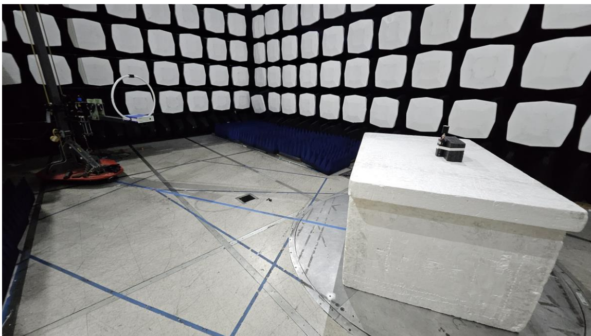
Figure A-2: Test Setup – Radiated Emissions < 30 MHz
