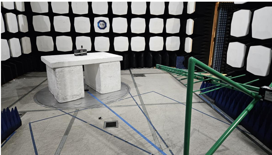
Figure A-3: Test Setup – Radiated Emissions < 1GHz
