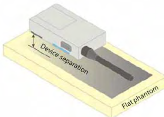
Fig-4.5 Illustration for Two-way Radio Setup
