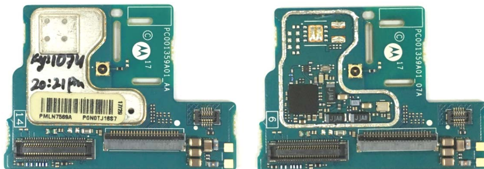
WIFI Board with and without Shield (Bottom)
