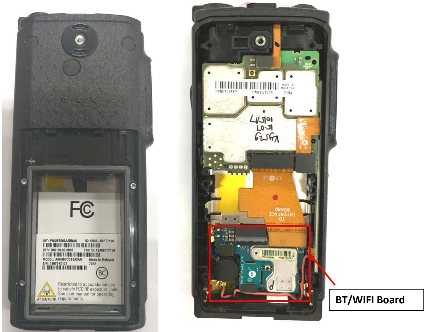
Chassis and Housing (Back)
