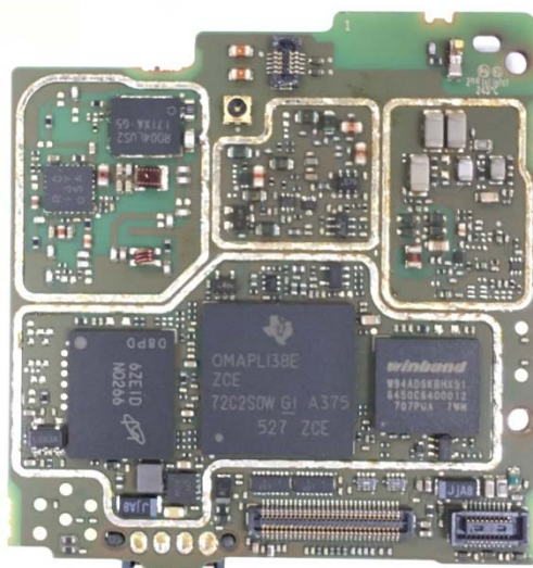
RF board without Shields (Bottom)
