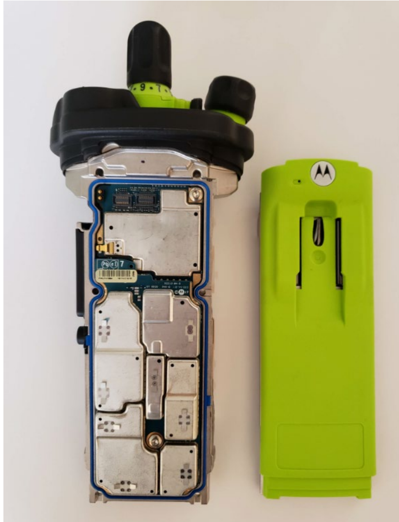
Exhibit 9I RF Board with chassis and housing (Front), Model 1.5
