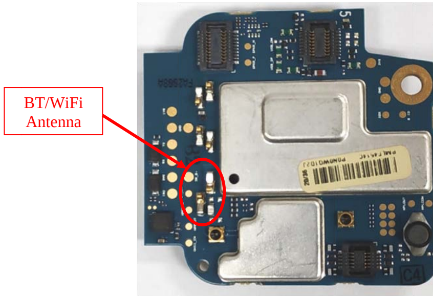
Expansion board with shields (Top) (APX8000H/ APX8000HXE)
