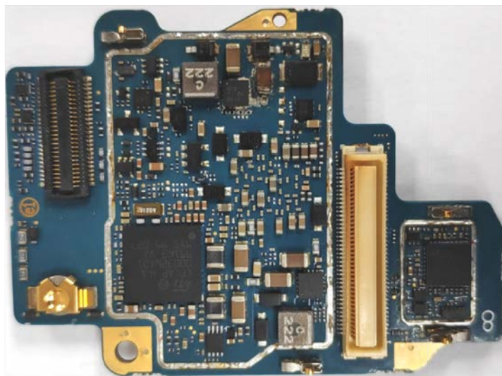
Vocon board without shields (Bottom) (APX8000H/ APX8000HXE)
