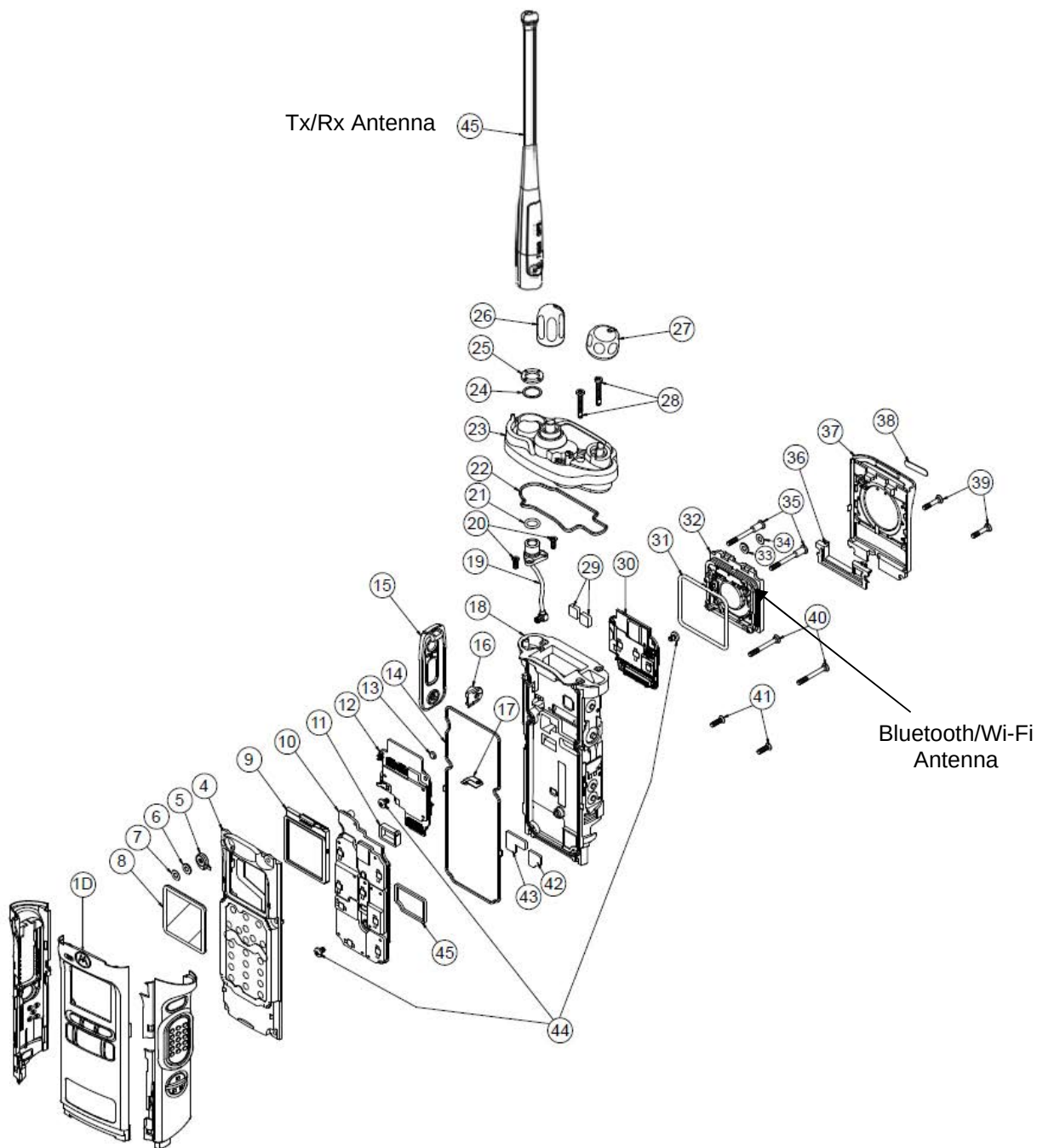
Exploded view of APX8000HXE Model 2.5 GRN
