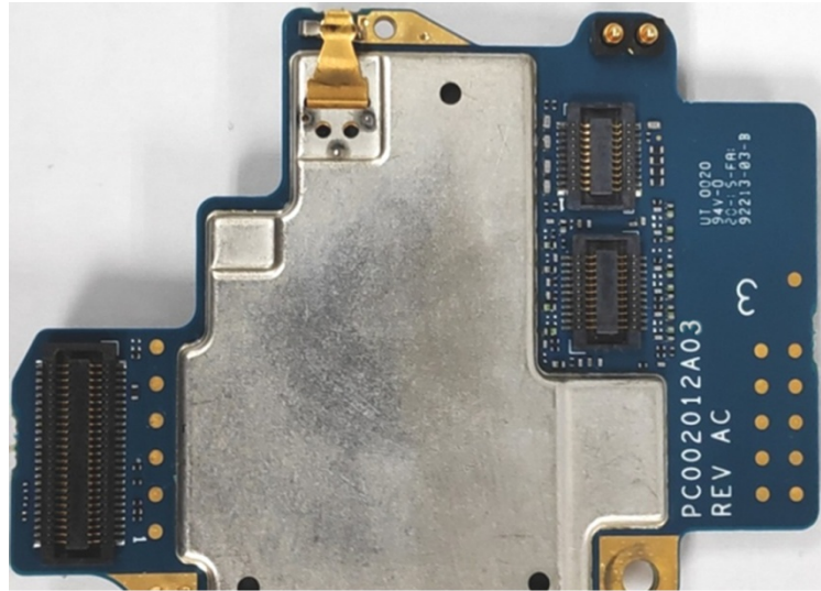
Vocon board with shields (Top) (APX8000H/ APX8000HXE)
