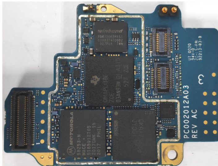
Vocon board without shields (Top) (APX8000H/ APX8000HXE)
