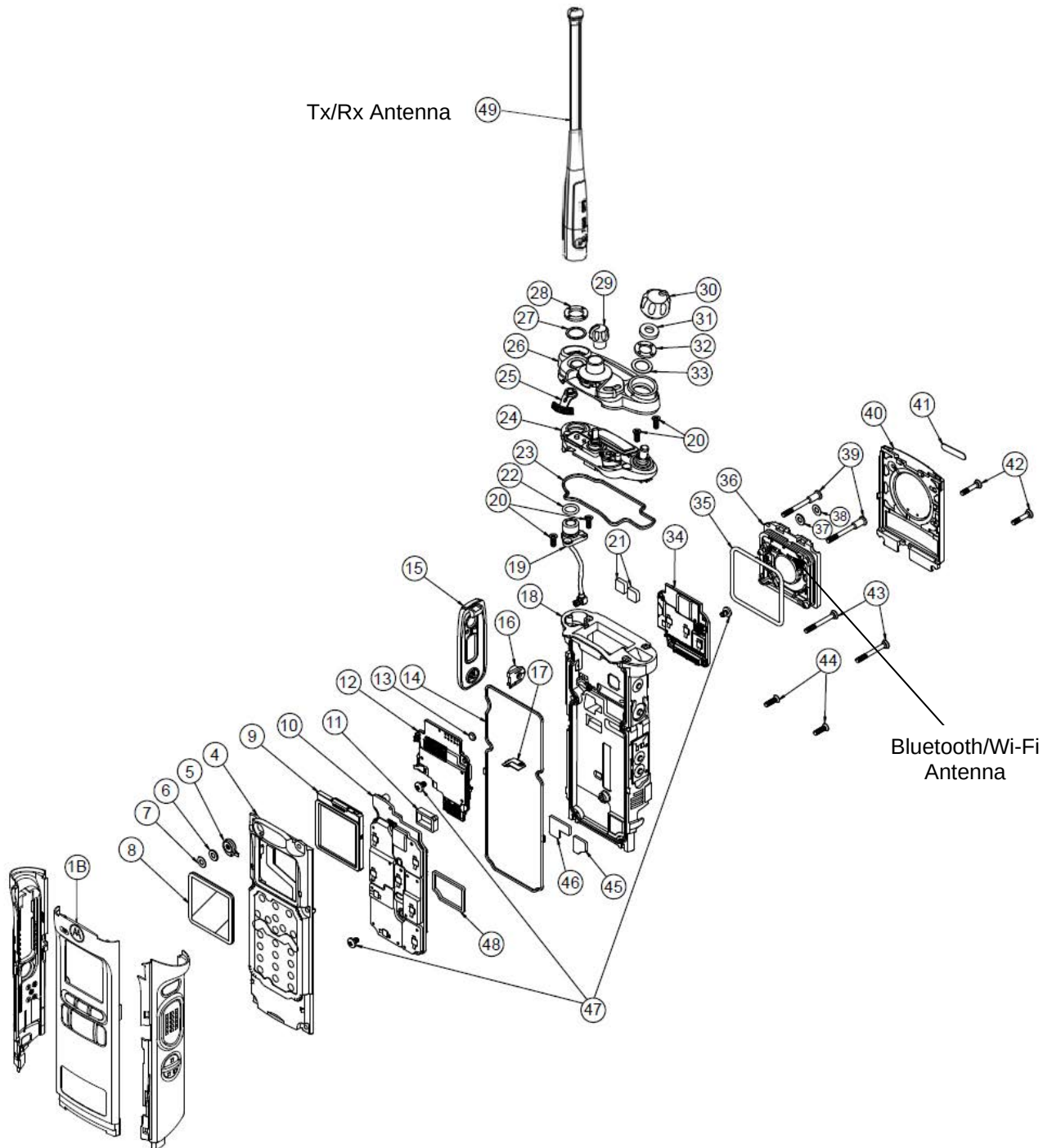
Exploded view of APX8000H Model 2.5 BLK/BRN
