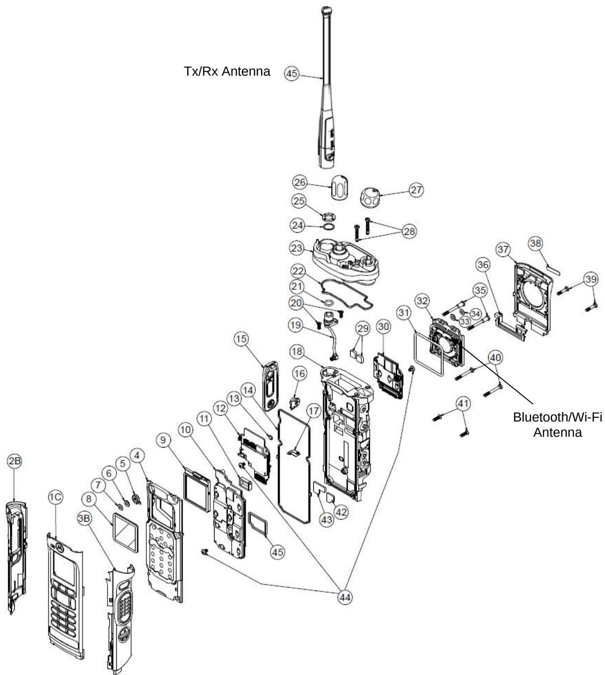
Exploded view of APX8000HXE Model 3.5 GRN
