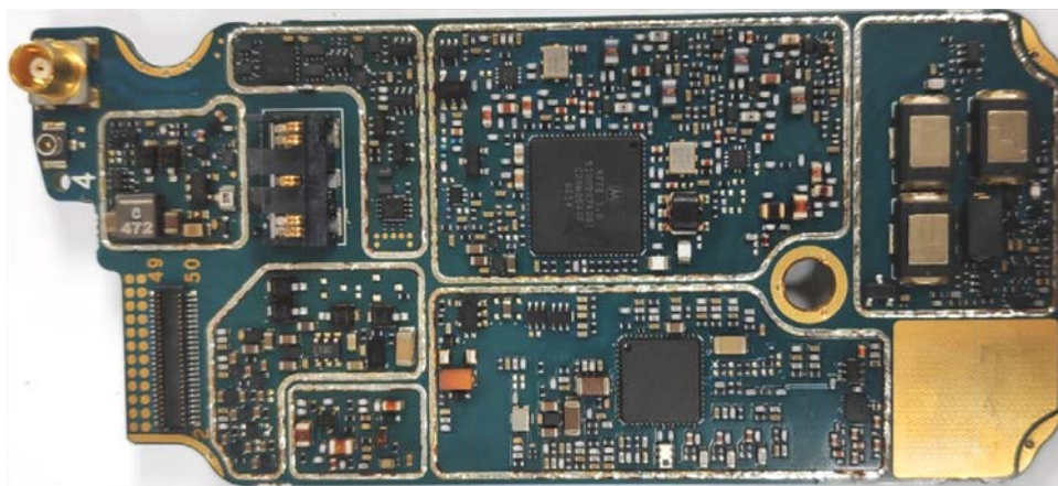
RF board without Shields (Bottom) (APX8000H/ APX8000HXE)
