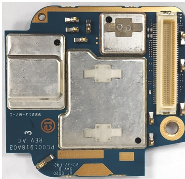
Expansion board with shields (Bottom) (APX8000H/ APX8000HXE)
