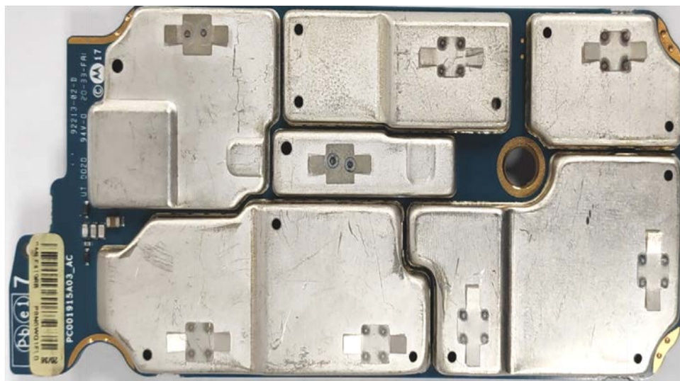
RF board with Shields (Top) (APX8000H/ APX8000HXE)
