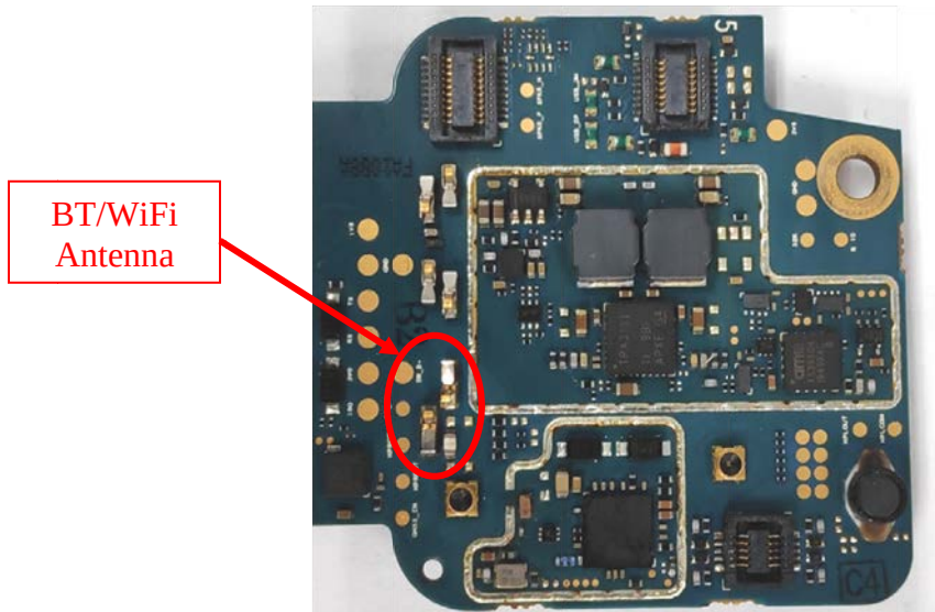
Expansion board without shields (Top) (APX8000H/ APX8000HXE)
