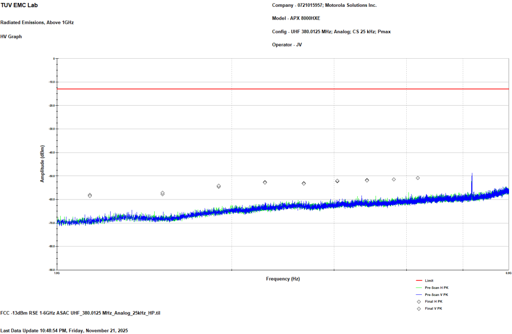
Figure 2.1.6-3: Reference plot for Field Strength of Spurious Emissions – 1 GHz – 6 GHz - Configuration 1
