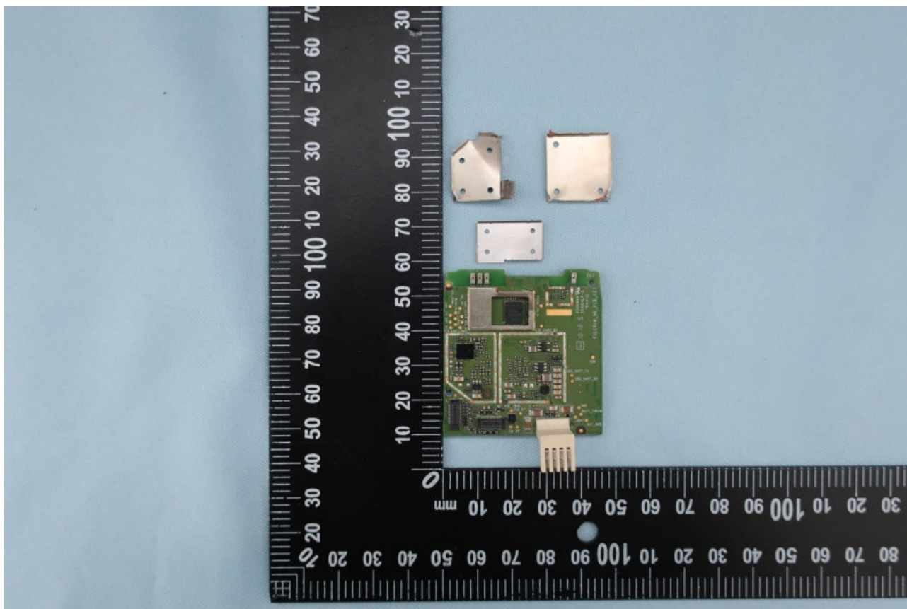
<Main PCBA top side remove shielding can>
