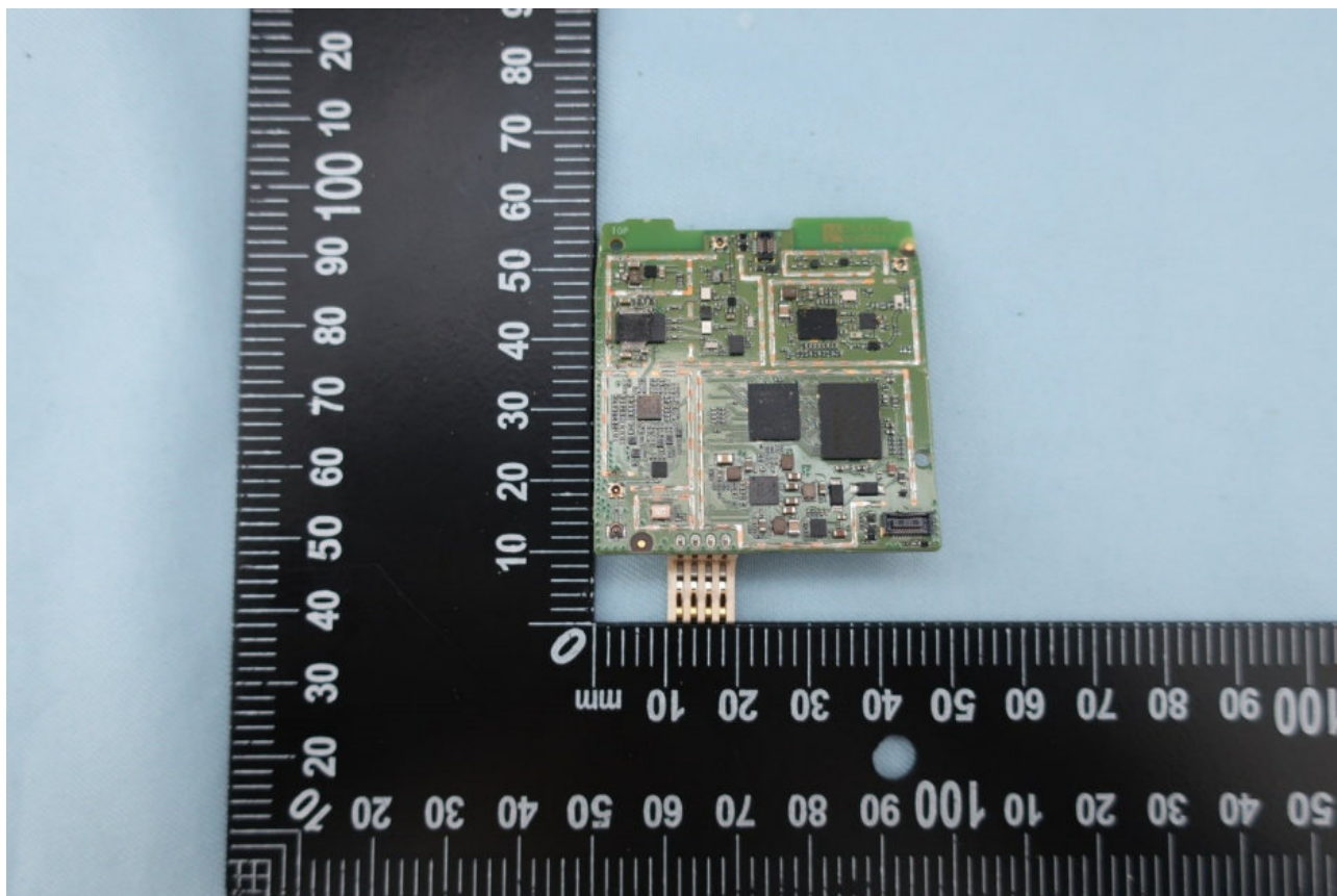
<Main PCBA bottom side remove shielding frame>
