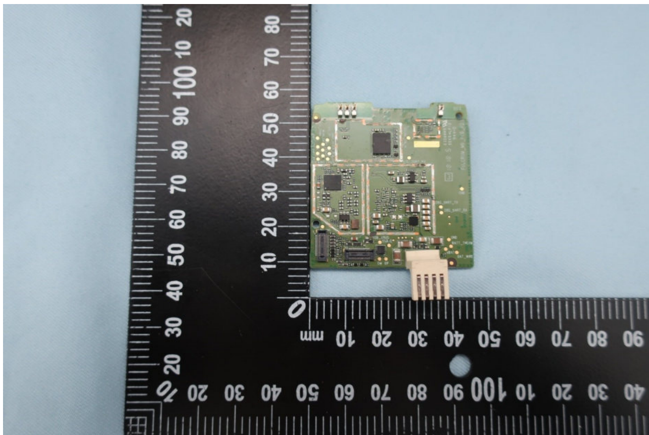
<Main PCBA top side remove shielding frame>
