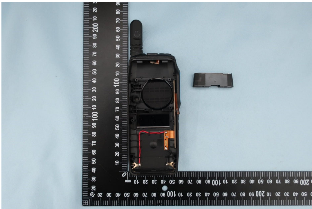
<Device disassembled GPS/WIFI/BT antenna frame>
