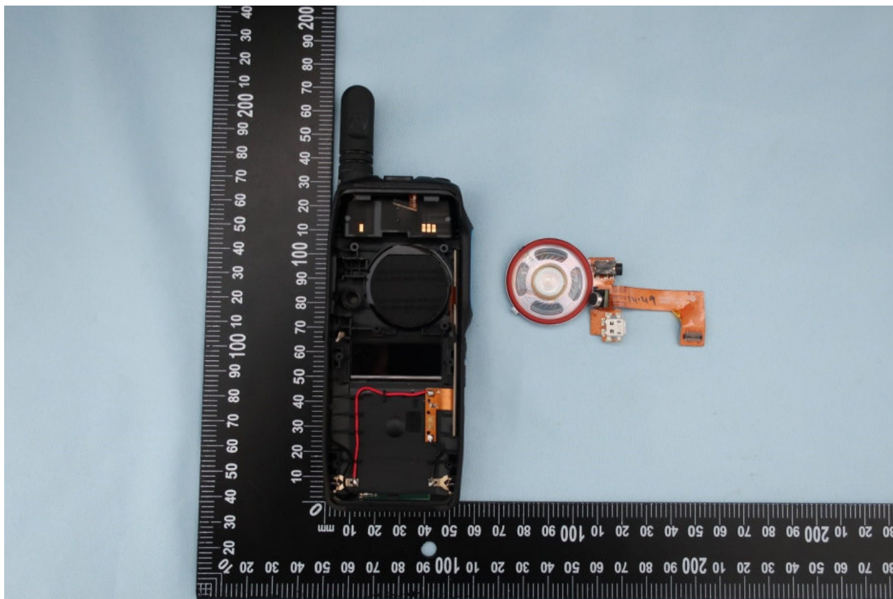
<Device disassembled speaker_mic_USB_audiojack FPCA>
