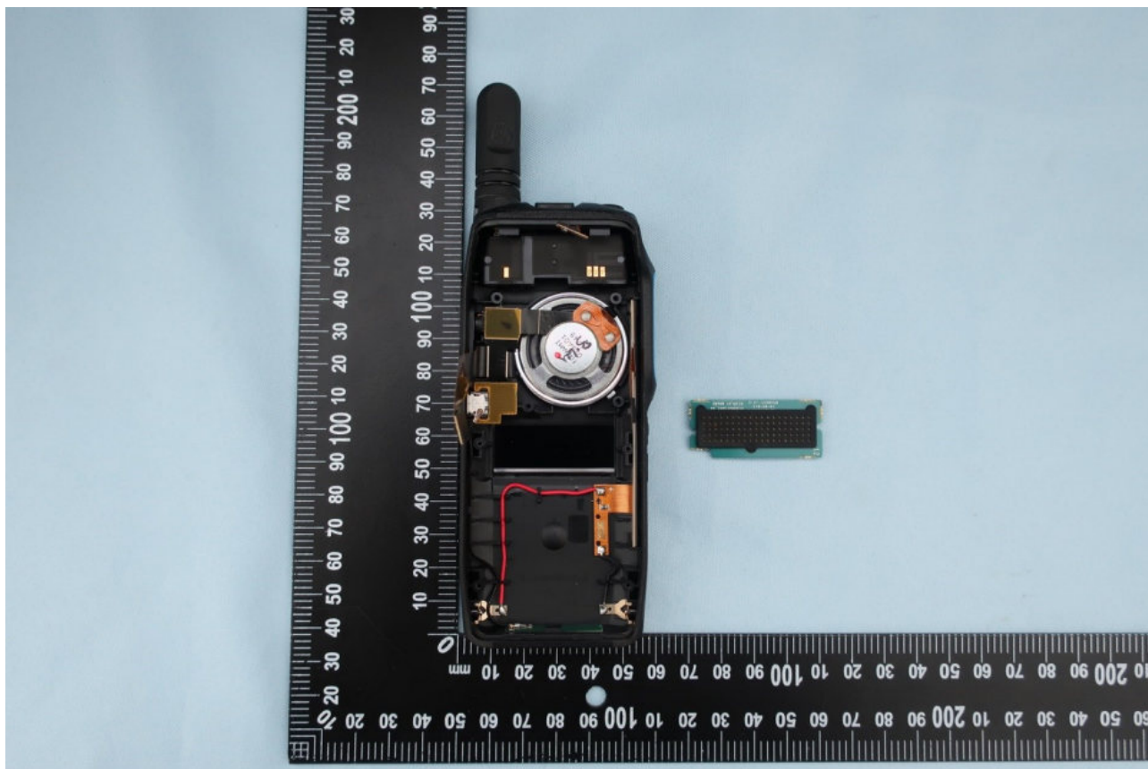
<Device disassembled display PCBA>
