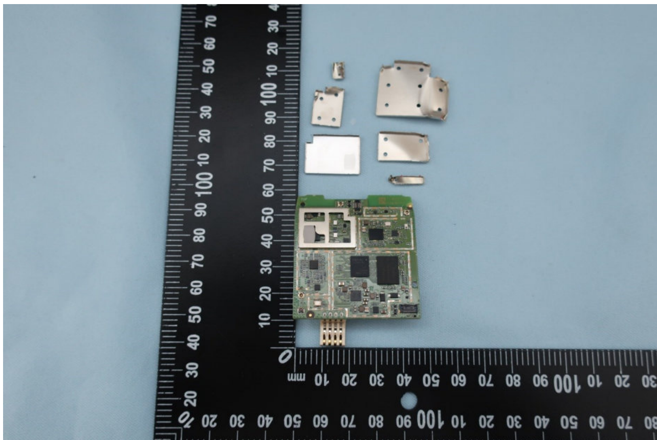
<Main PCBA bottom side remove shielding can>
