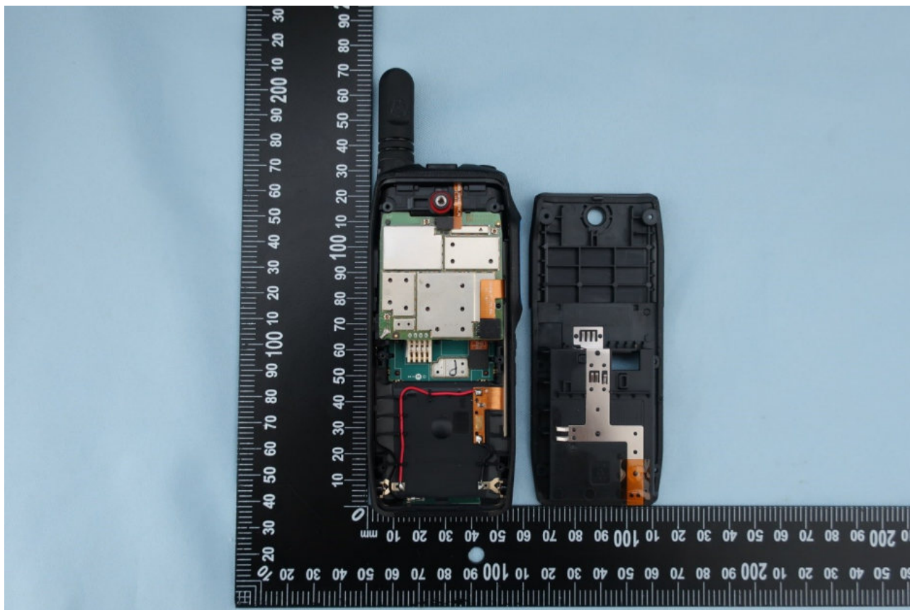
<Device disassembled rear housing>
