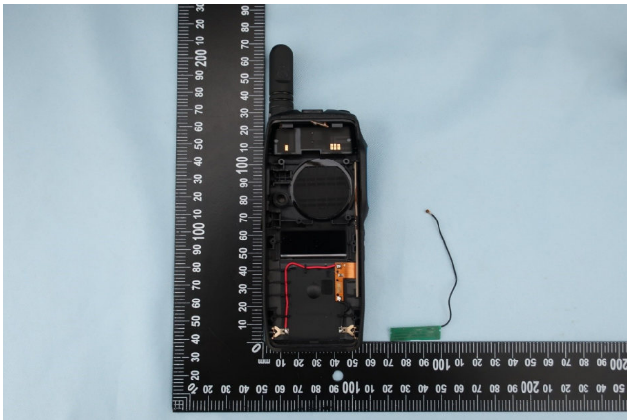
<Device disassembled LTE diversity antenna>
