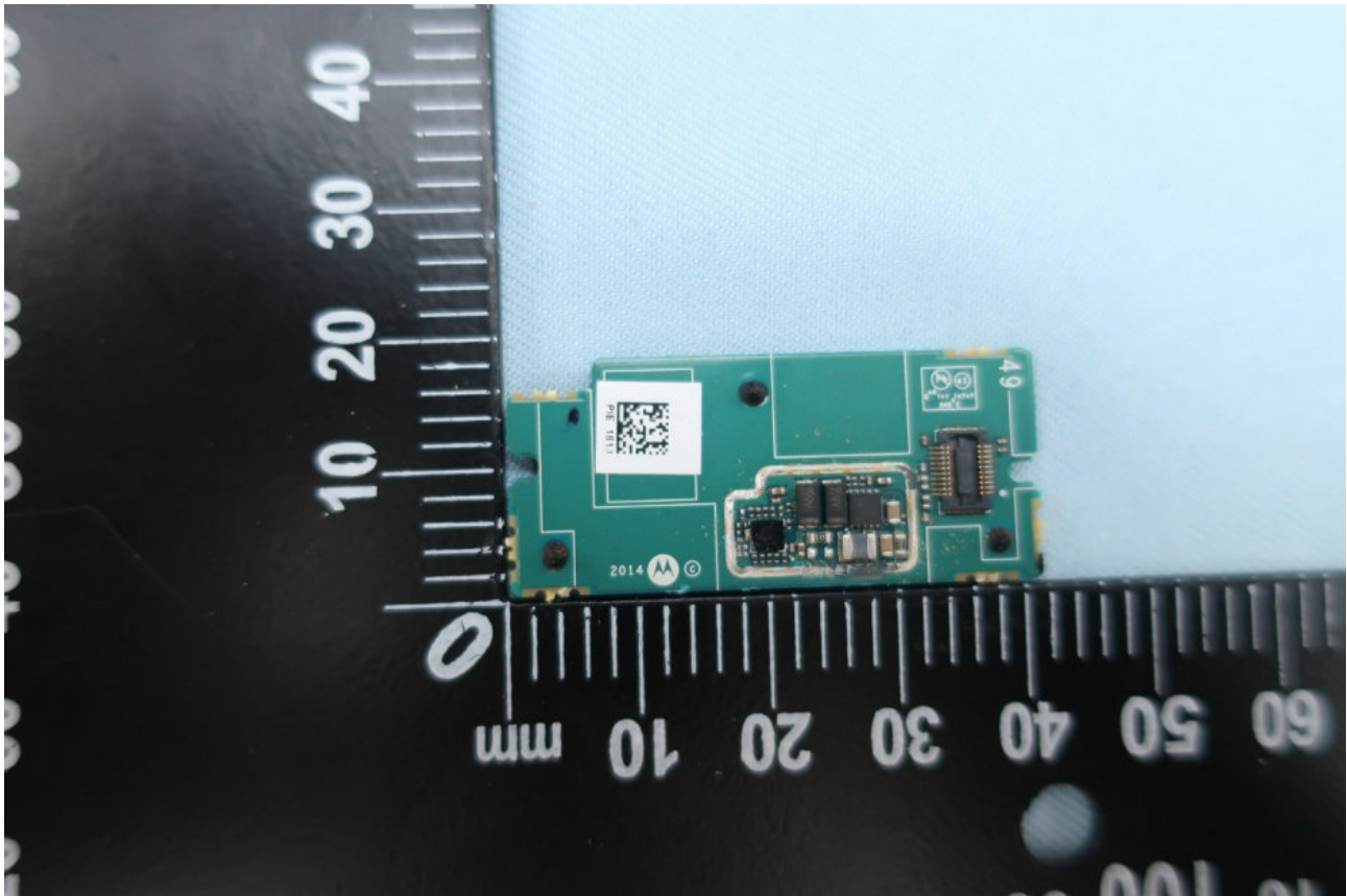
<Display PCBA bottom side without shielding can>
