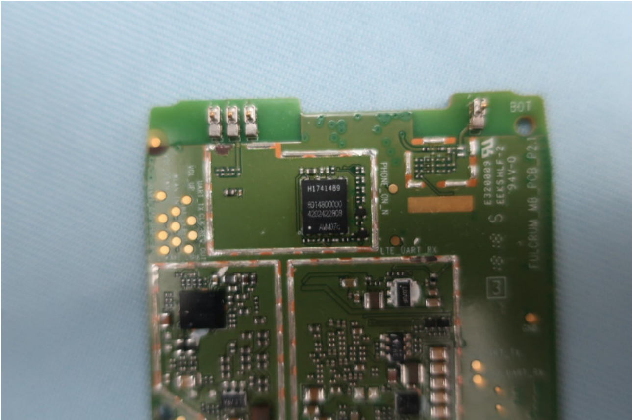
<Main PCBA bottom side without shielding can>
