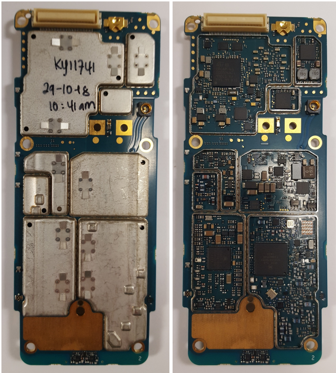
Exhibit 9B Main board with & without Shields (Bottom)
