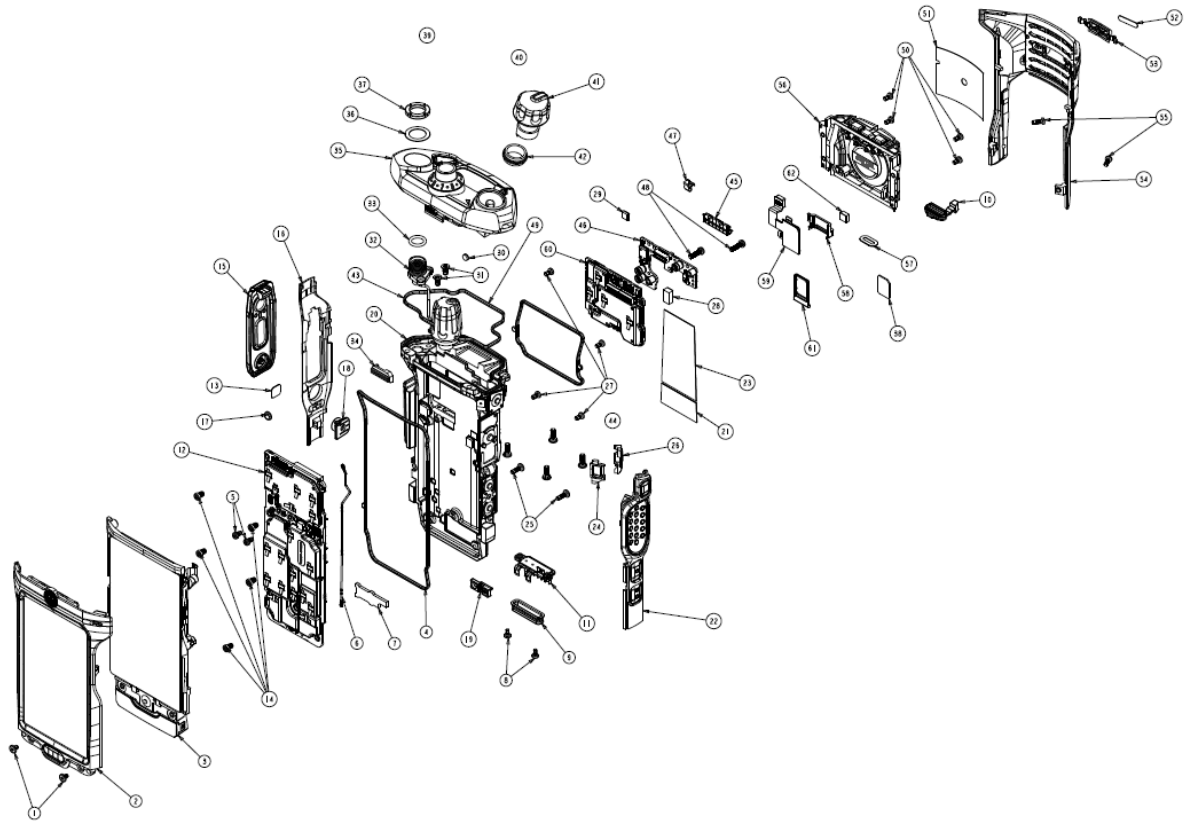
Exhibit 9I XE Exploded View of Radio
