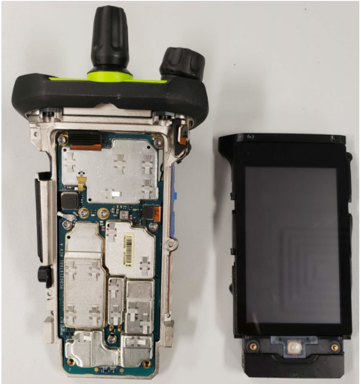
Exhibit 9G XE RF board with Chassis and Housing (Front)
