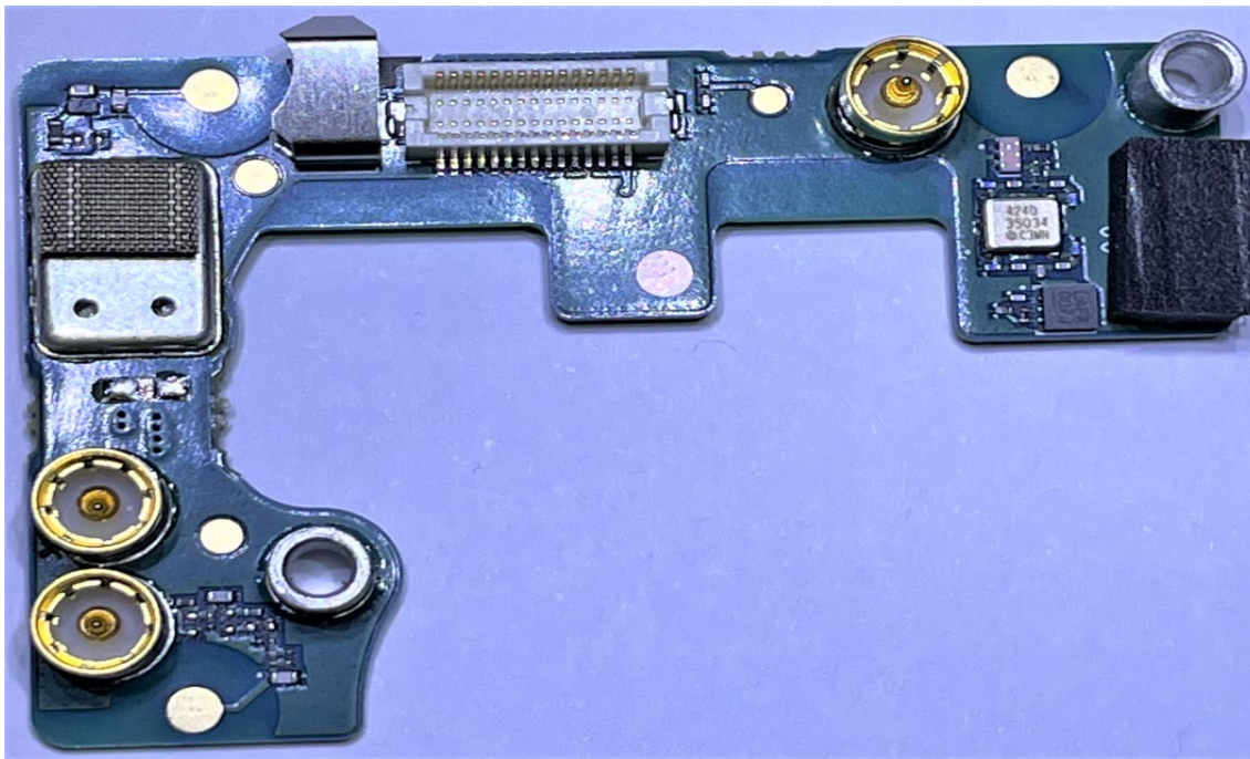
9L: IPCB board with Shields (Bottom)
