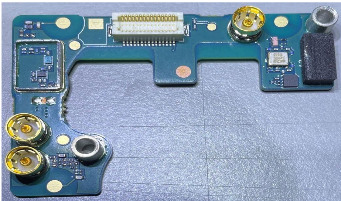
9M: IPCB board without Shields (Bottom)
