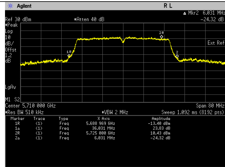
Frequency 5710 MHz, UNII-2C & UNII-3(FCC)
