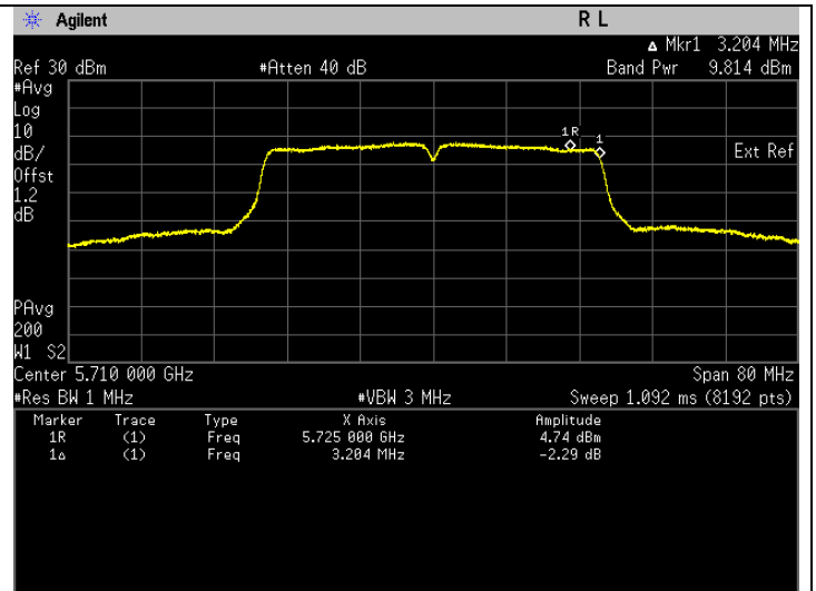
Frequency 5710 MHz, ISSED, U-NII-3. *Note: The band power is captured after the 5725 MHz.
