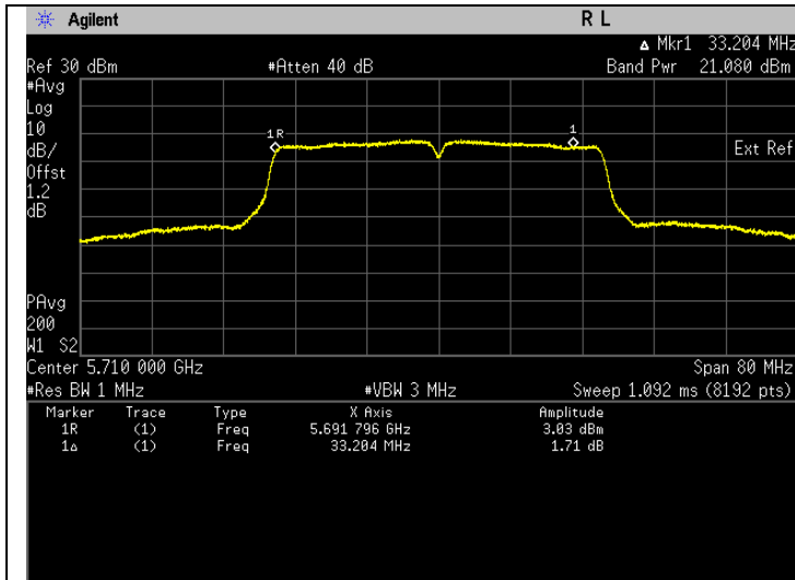
Frequency 5710 MHz, ISSED, U-NII-2C. *Note: The band power is captured before the 5725 MHz.
