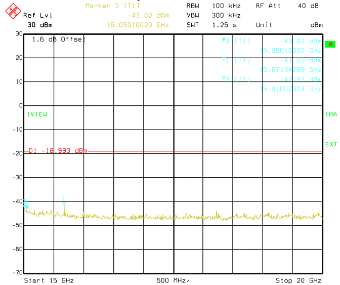
Date: 18.JAN.2019 15:01:14 Conducted Emissions. 802.11g, Frequency 2437 MHz Emission Level, 15 GHz -> 20 GHz
