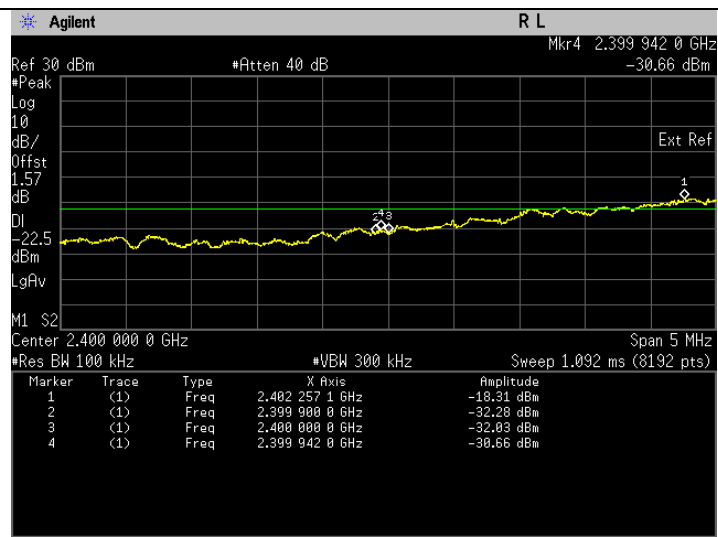
Band Edge. 802.11n Frequency 2422 MHz Band Edge
