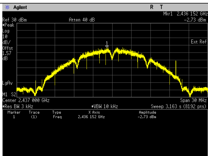
Frequency 2437 MHz, Antenna 1
