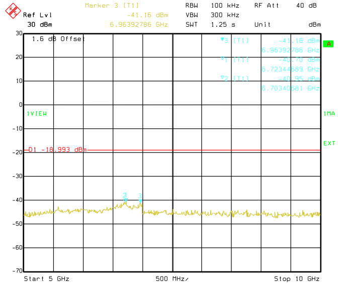
Date: 18.JAN.2019 14:59:27 Conducted Emissions. 802.11g, Frequency 2437 MHz Emission Level, 5 GHz -> 10 GHz
