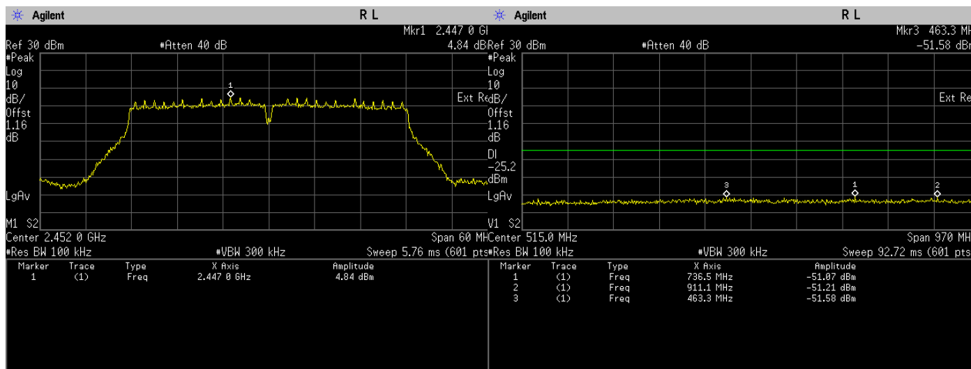
Conducted Emissions(Average). 802.11n, Frequency 2452 MHz Reference Level
