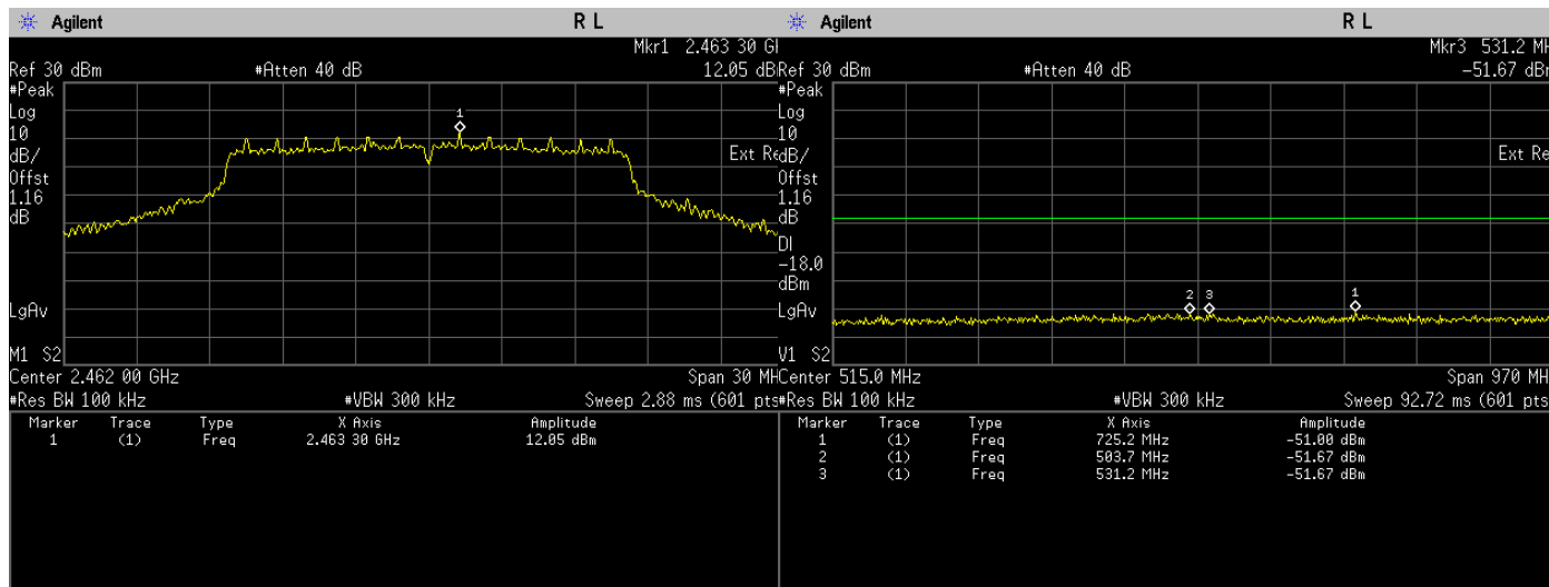
Conducted Emissions(Average). 802.11g, Frequency 2462 MHz Reference Level
