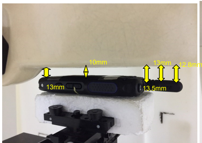
Back, Test Separation 10 mm
