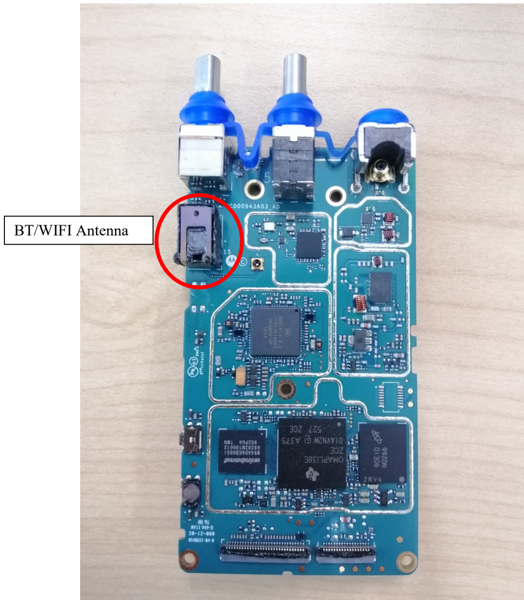
RF board without Shields (Top)
