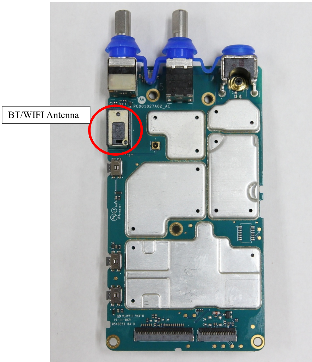
RF board with Shields (Top)
