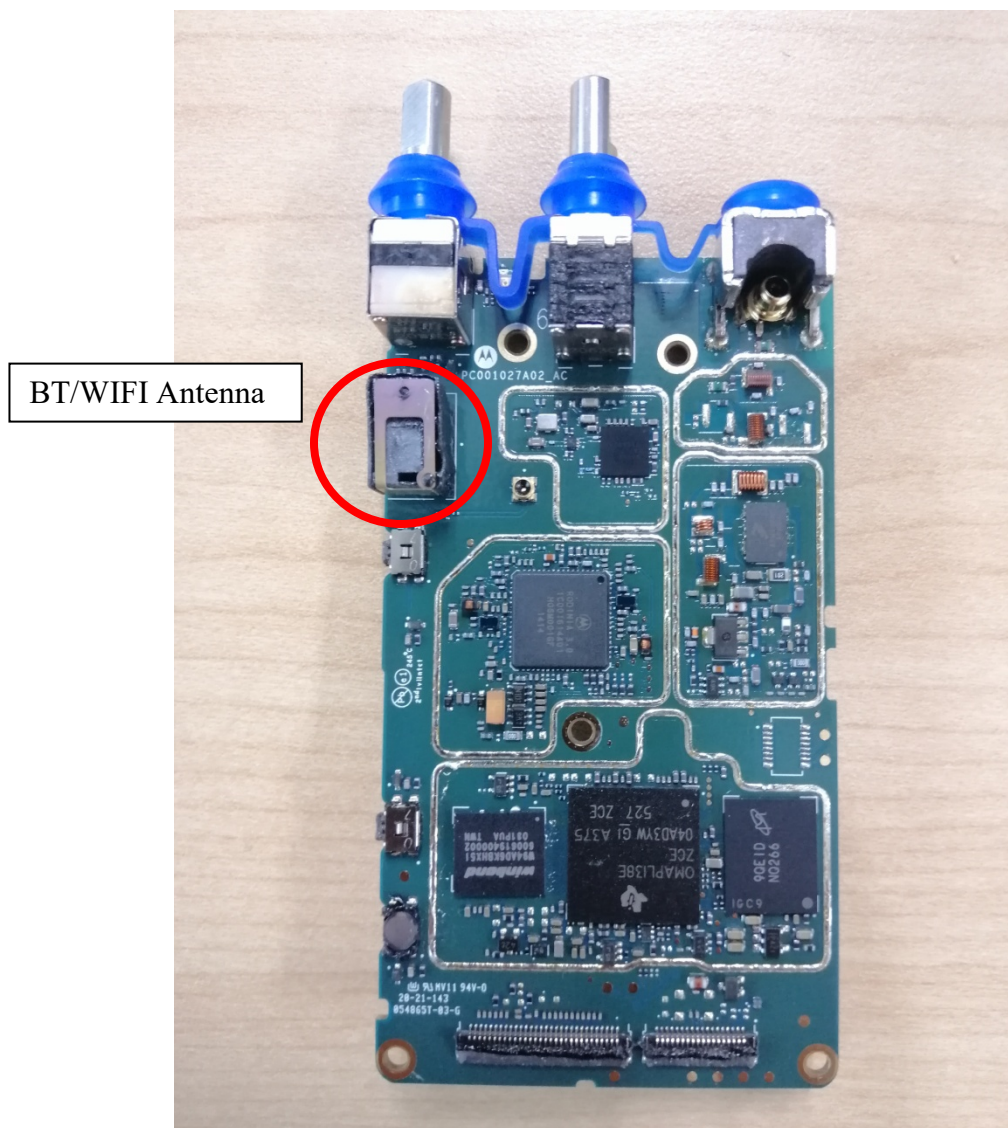
RF board without Shields (Top)
