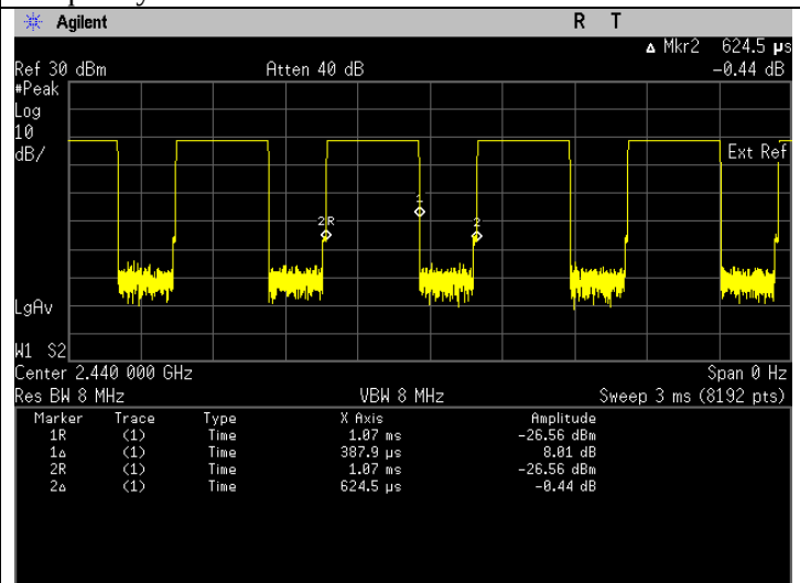
Duty Cycle
