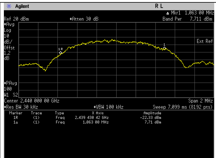
Frequency 2440 MHz
