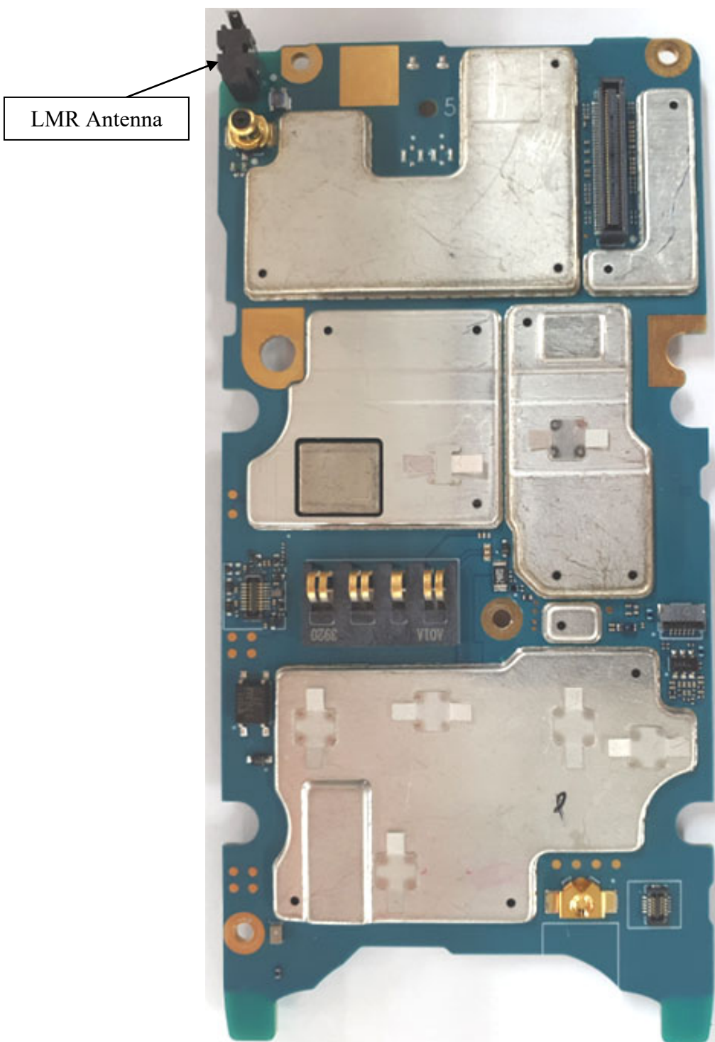
Exhibit 9G: LMR RF board with Shields (Bottom)
