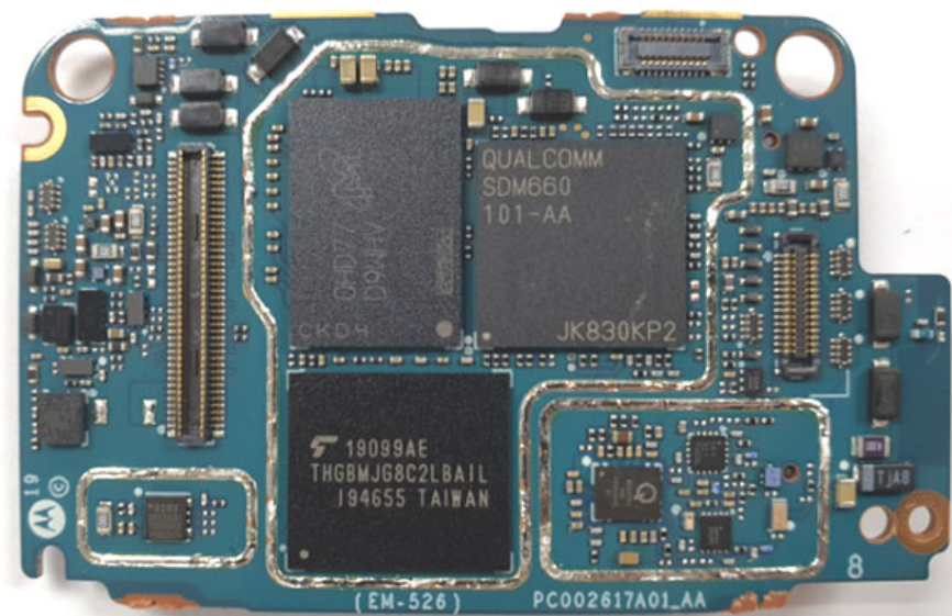
Exhibit 9F: AP board without Shields (Top)
