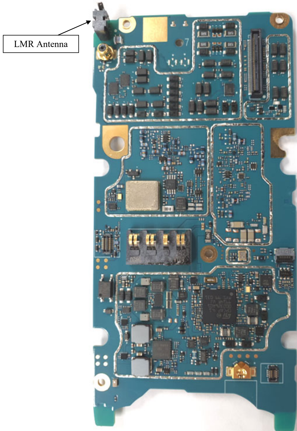
Exhibit 9J: LMR RF board without Shields (Bottom)
