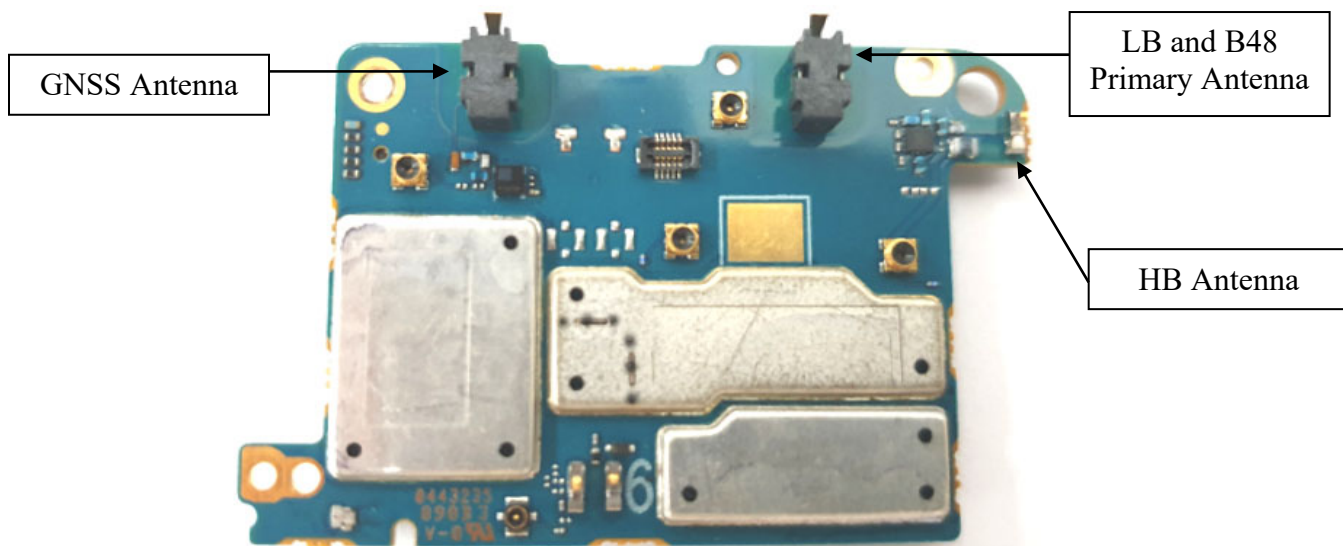
Exhibit 9H: LTE RF board with Shields (Bottom)
