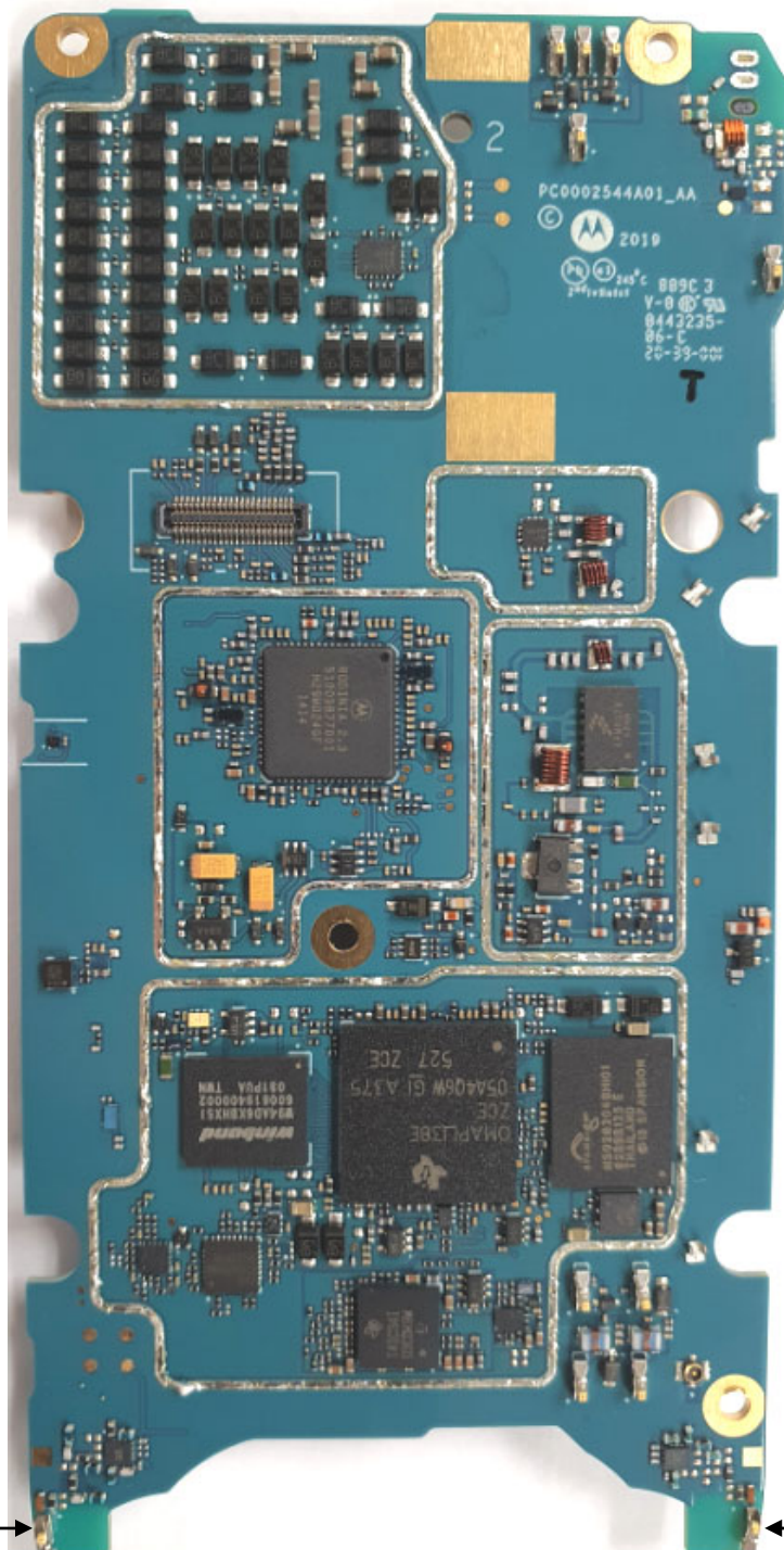
Exhibit 9D: LMR RF board without Shields (Top)
