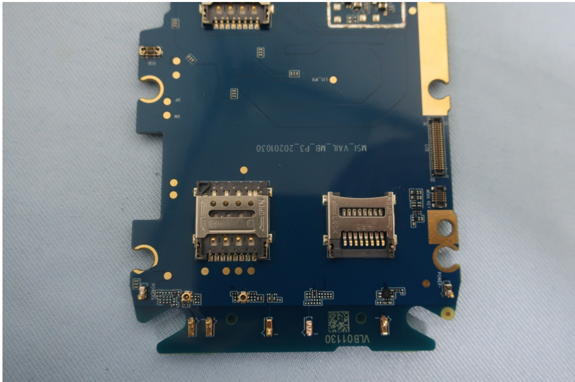
SIM1 card connector T-Flash connector
