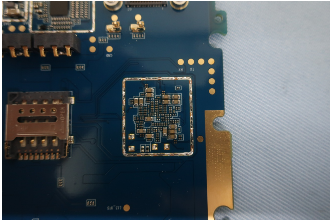
SIM2 card connector CPU power decoupling capacitor circuit on PCBA
