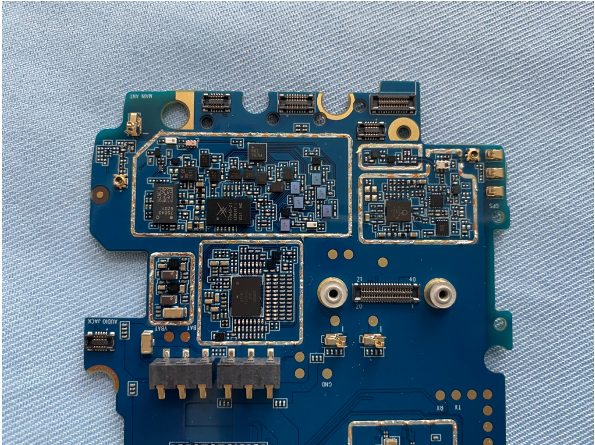
APT and transceiver circuit on PCBA
