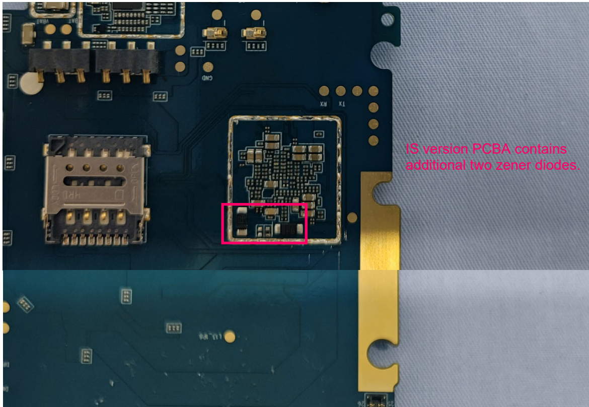
SIM2 card connector CPU power decoupling capacitor circuit on PCBA
