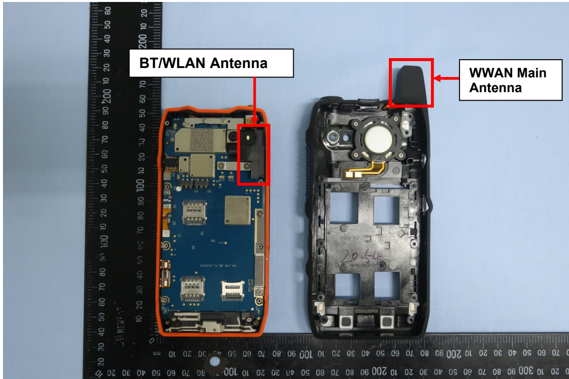
PCB board with chassis (Top) and rear housing
