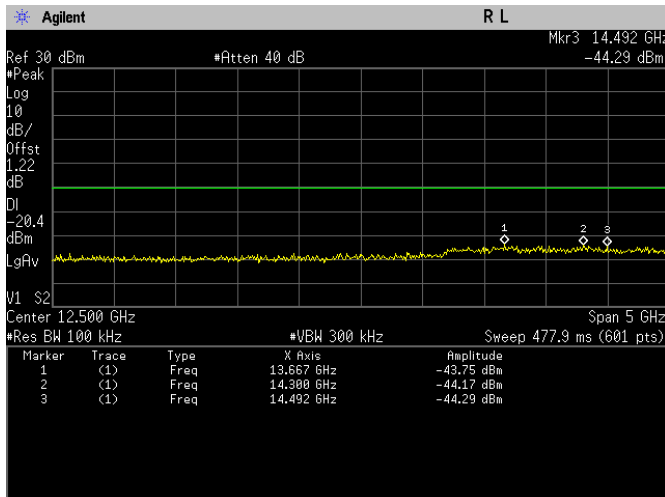
Conducted Emissions(Peak). 802.11g, Frequency 2412 MHz Emission Level, 10 GHz -> 15 GHz
