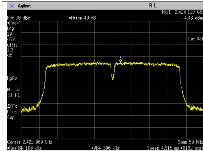
Band Edge(Peak). 802.11n Frequency 2422 MHz Reference Level
