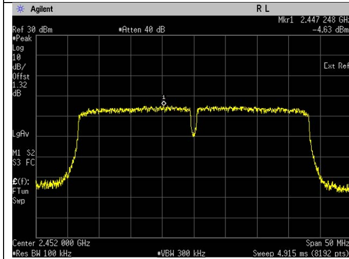
Band Edge(Peak). 802.11n Frequency 2452 MHz Reference Level
