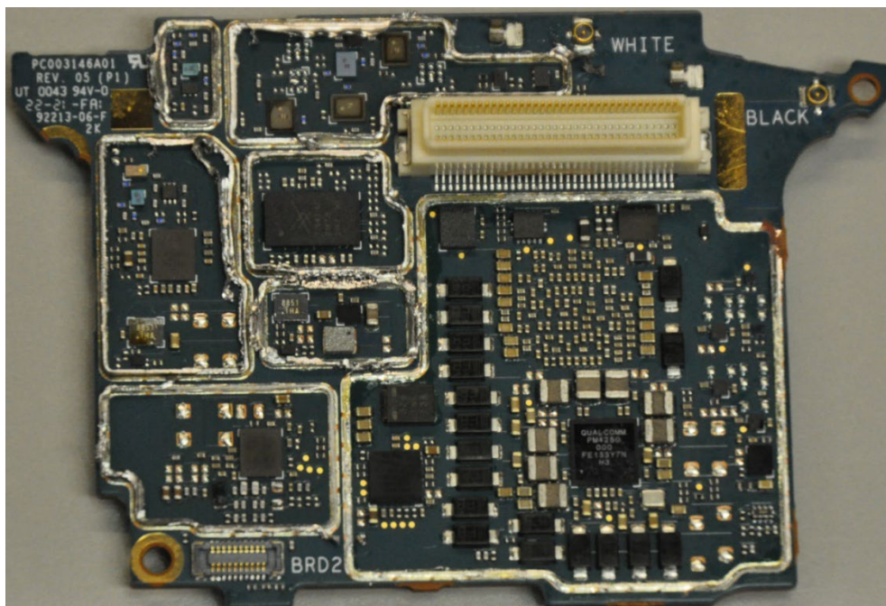
Exhibit 9J - AP board without Shields (Bottom)
