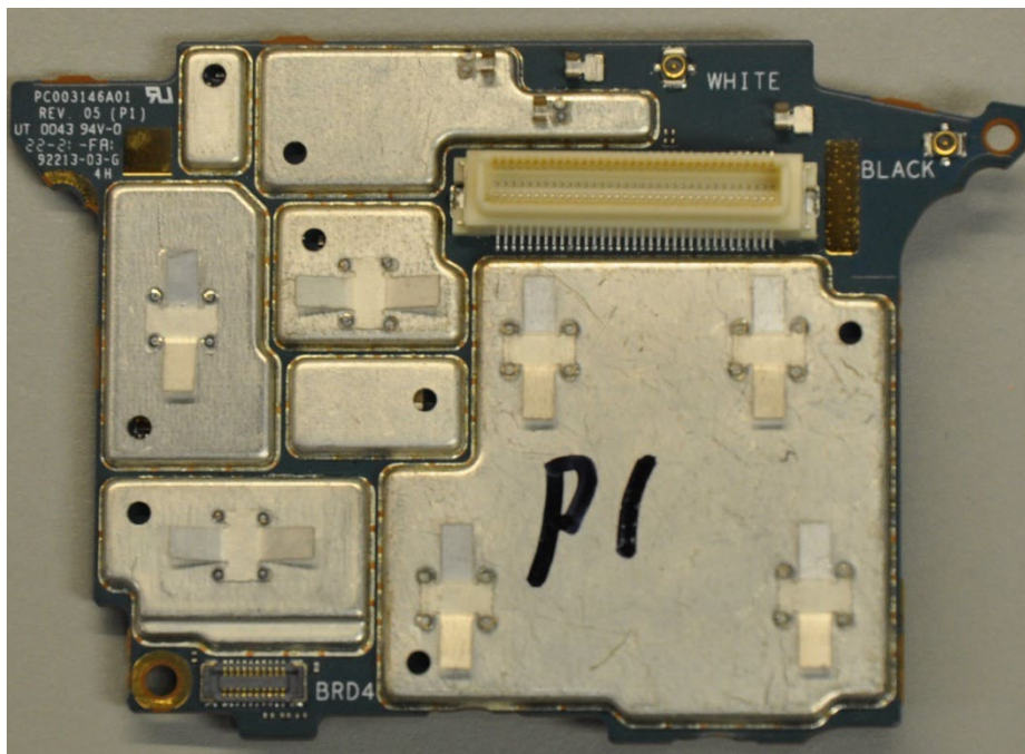
Exhibit 9I - AP board with Shields (Bottom)
