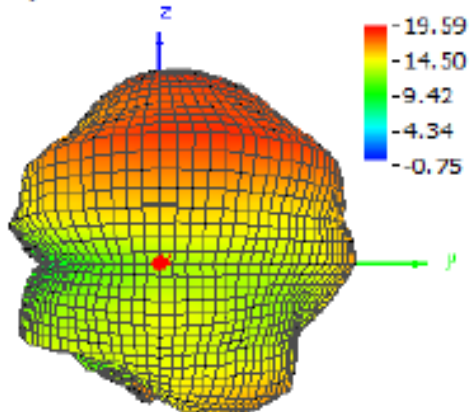
Theta = 90, Phi = 0
