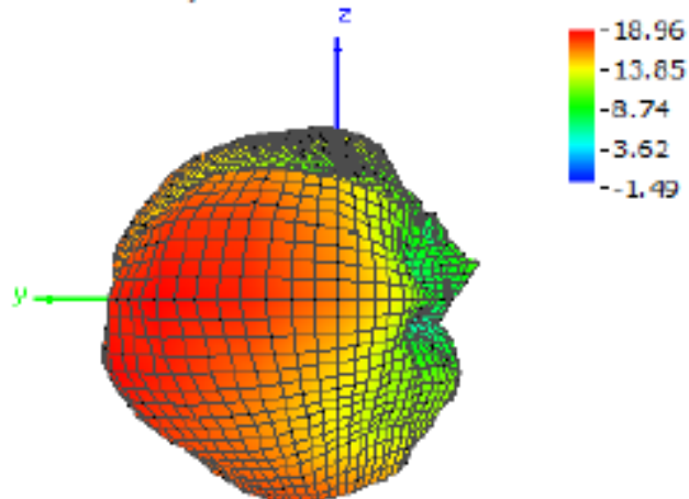
Theta = 90, Phi = 180
