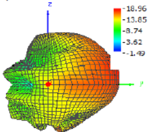
Theta = 90, Phi = 0
