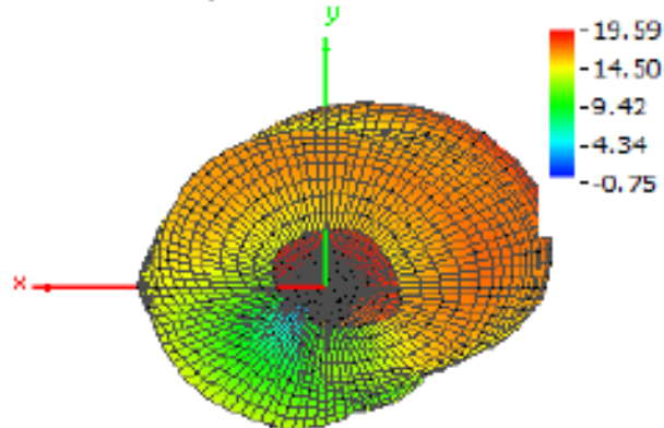
Theta = 180, Phi = 0
