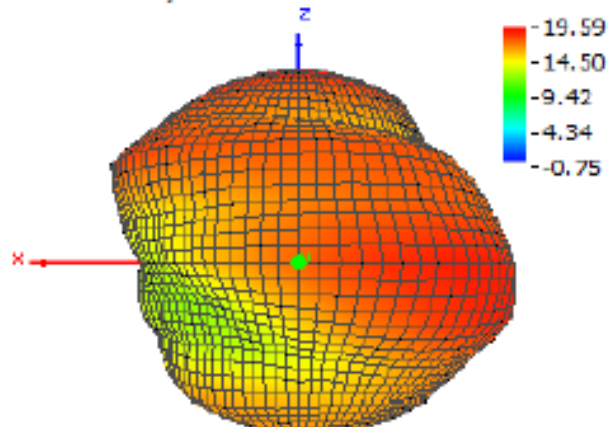
Theta = 90, Phi = 90
