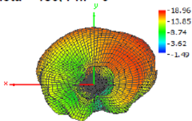
Theta = 180, Phi = 0
