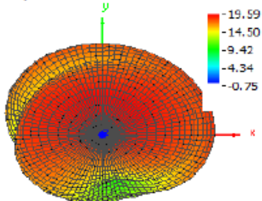
Theta = 0, Phi = 0
