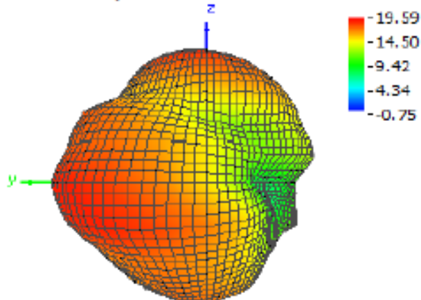
Theta = 90, Phi = 180
